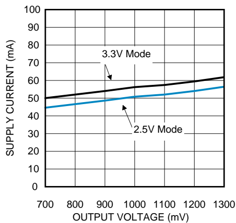
Figure 8. Supply Current vs. Output Voltage Setting
