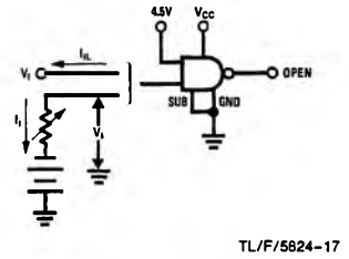
Each input is tested separately. FIGURE 3. V_I , I_I
