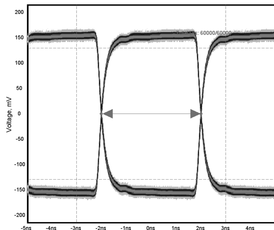
Figure 15. LVDS RxCLKOUT Output (1.25 Gbps, 40m CAT-5e, 0x000 DS32ELX0124 EQ setting, 0x10 DS32EL0421 De-Emphasis setting)
