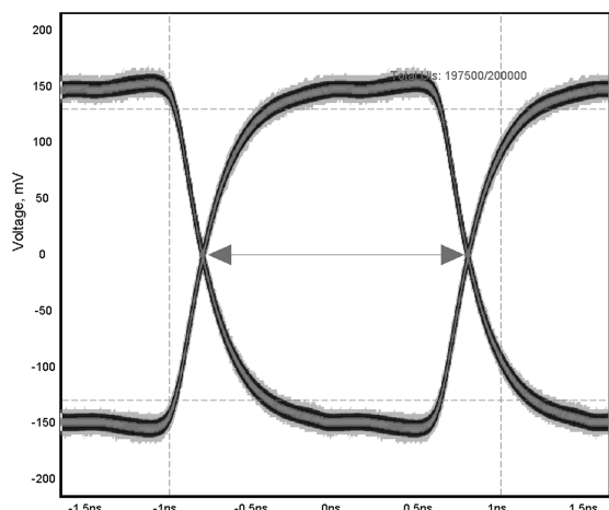
Figure 17. LVDS RxCLKOUT Output (3.125 Gbps, 20m CAT-6 SCTP, 0x001 DS32ELX0124 EQ setting, 0x10 DS32EL0421 De-Emphasis setting)
