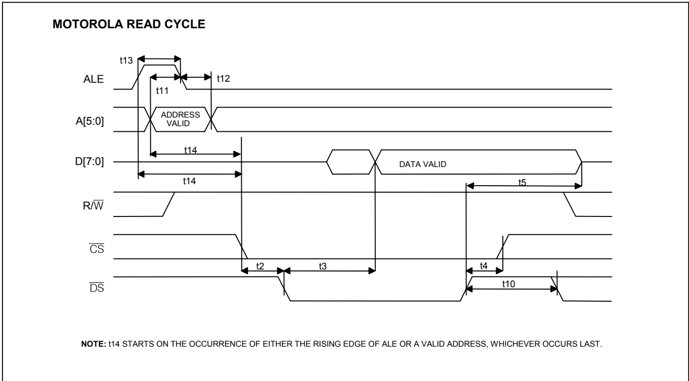
Figure 13-4. CPU Bus AC Timing Diagram (Multiplexed) (continued)
