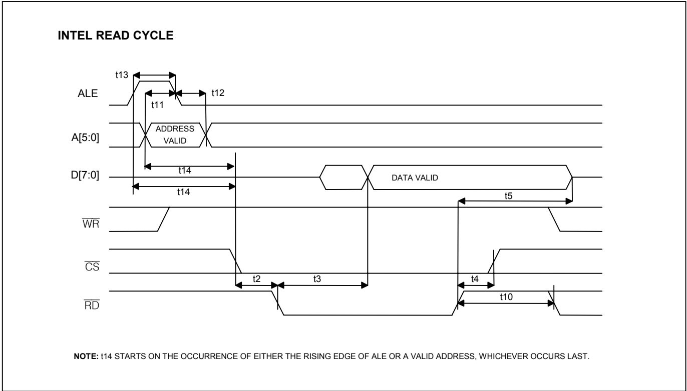
Figure 13-4. CPU Bus AC Timing Diagram (Multiplexed)
