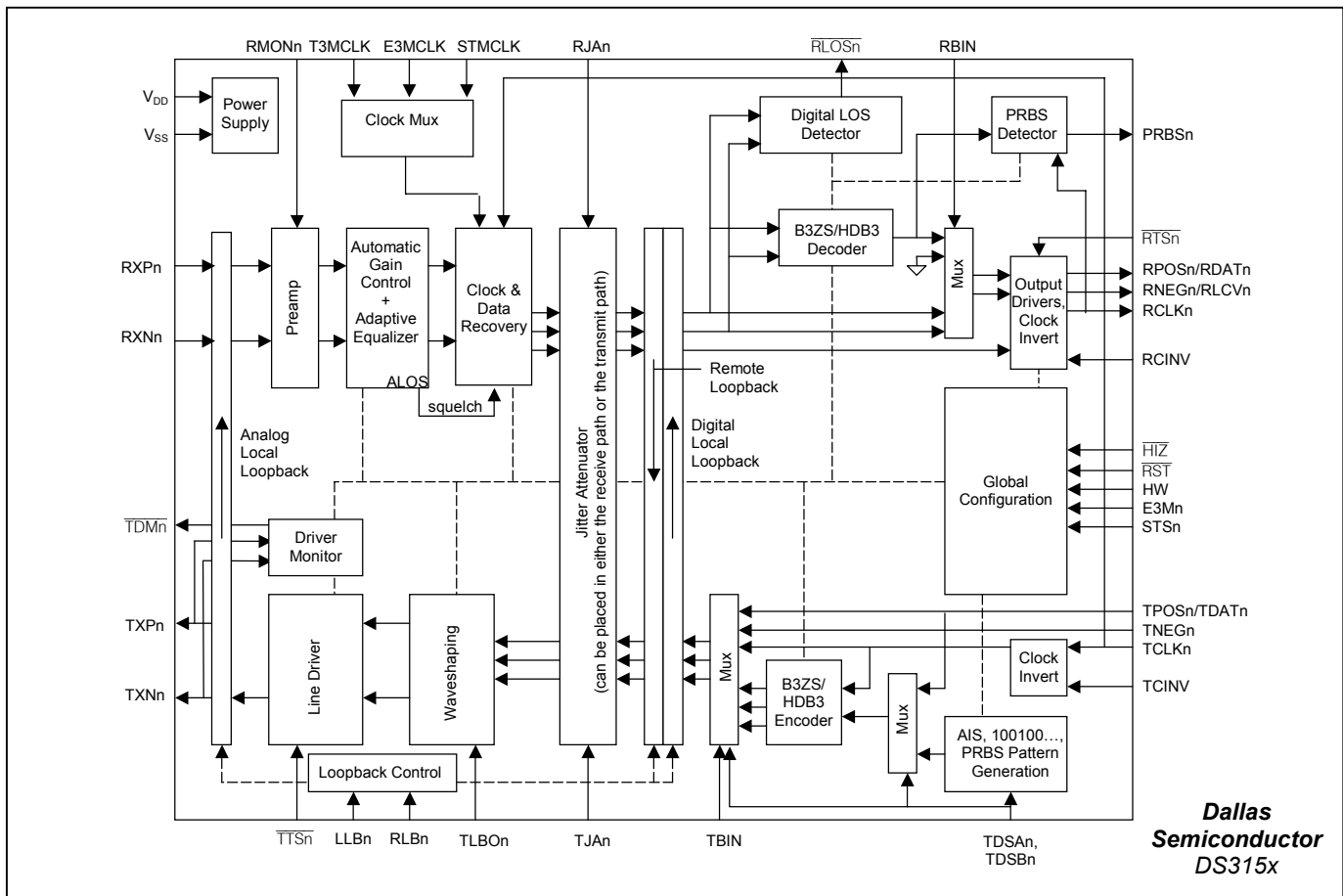
Figure 3-1. Hardware Mode Block Diagram
