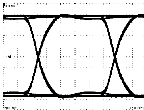
Figure 6. A 2.5 Gbps NRZ PRBS-7 After 2" Differential FR-4 Stripline V:100 mV / DIV, H:75 ps / DIV
