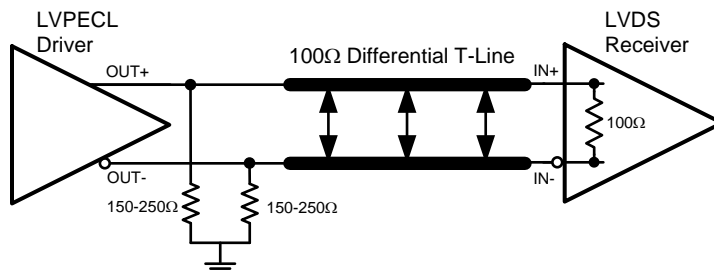
Figure 3. Typical LVPECL Driver DC-Coupled Interface to DS25CP152 Input
