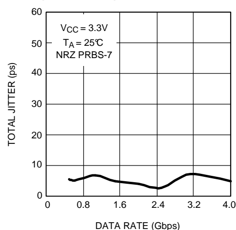
Figure 8. Total Jitter as a Function of Data Rate
