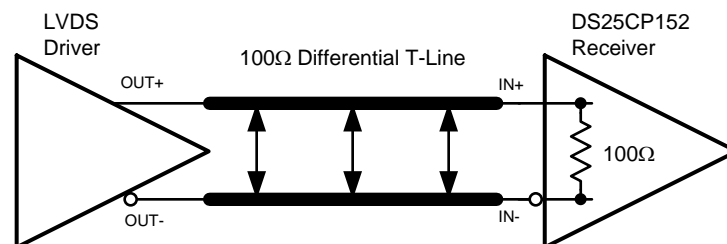
Figure 1. Typical LVDS Driver DC-Coupled Interface to DS25CP152 Input
