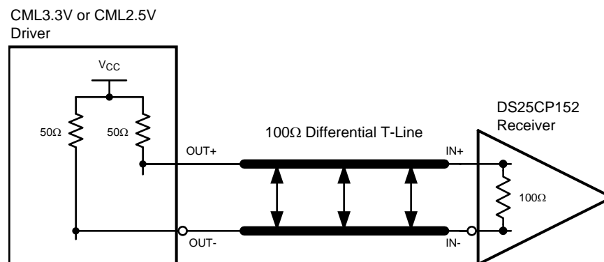
Figure 2. Typical CML Driver DC-Coupled Interface to DS25CP152 Input
