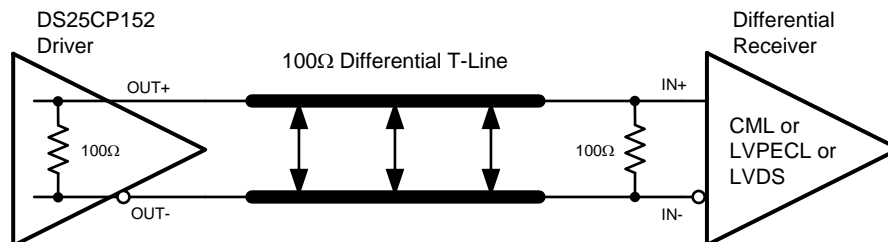
Figure 4. Typical DS25CP152 Output DC-Coupled Interface to an LVDS, CML or LVPECL Receiver
