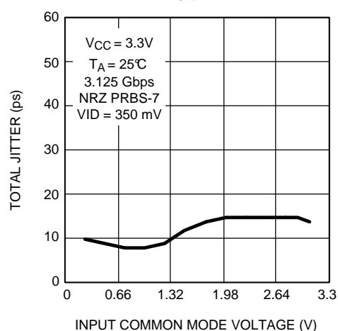
Figure 7. Total Jitter as a Function of Input Common Mode Voltage
