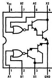
Top View Order Number DS1633J-8 or DS3633N
