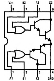
Top View Order Number DS1634J-8 or DS3634N
