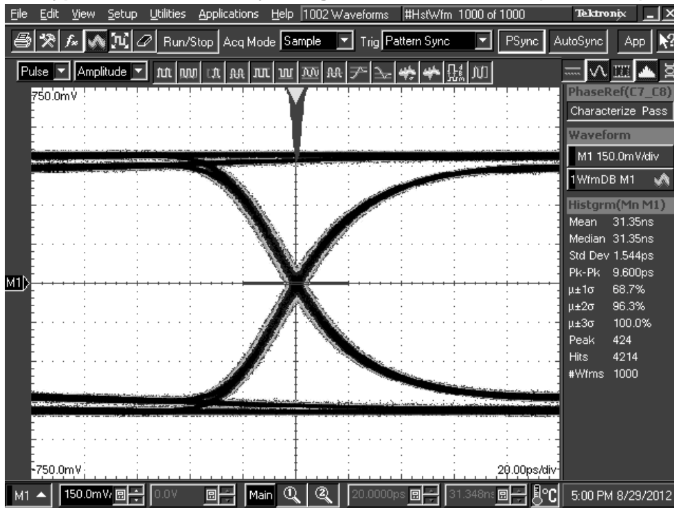
Figure 15. TL = 20 inch 5-mil FR4 trace, 5 Gbps DS125BR800 settings: EQ[1:0] = 0, 1 = 03'h, DEM[1:0] = 0, 1
