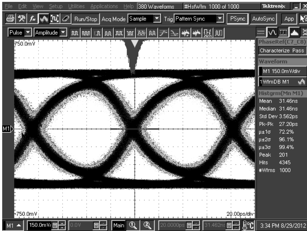
Figure 22. TL1 = 8-meter 30-AWG 100 Ohm Twin-axial Cable, 12 Gbps DS125BR800 settings: EQ[1:0] = R, 1 = 0F'h, DEM[1:0] = 0, 1
