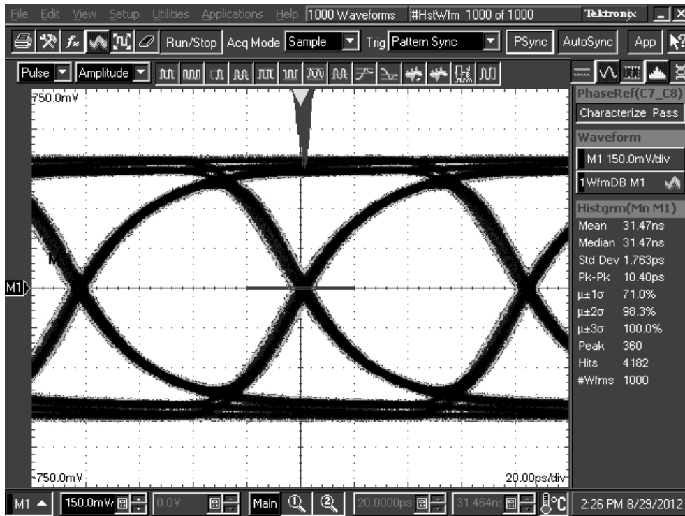
Figure 14. TL = 10 inch 5-mil FR4 trace, 12 Gbps DS125BR800 settings: EQ[1:0] = 0, R = 01'h, DEM[1:0] = 0, 1
