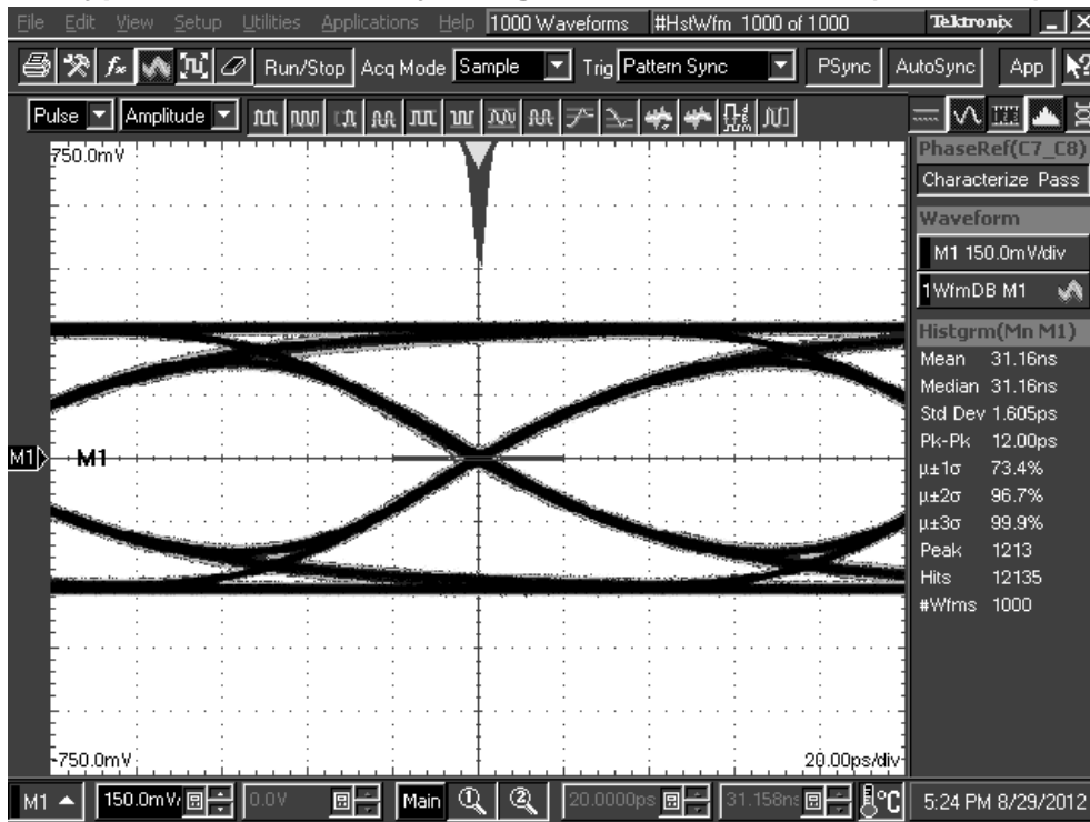
Figure 25. TL1 = 20 inch 5-mil FR4 trace, TL2 = 10 inch 5-mil FR4 trace, 8 Gbps DS125BR800 settings: EQ[1:0] = R, 1 = 03'h, DEM[1:0] = R, 0
