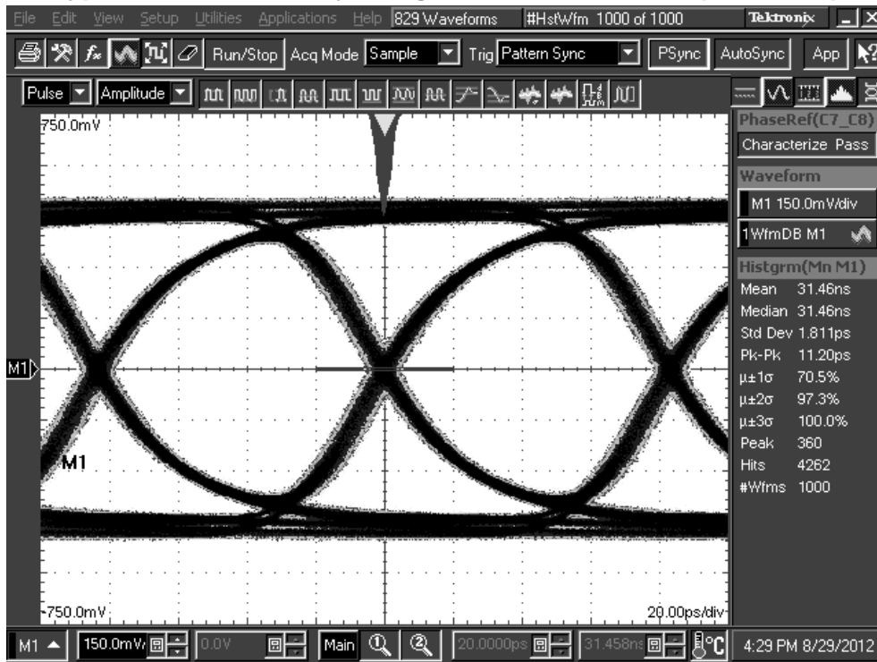
Figure 17. TL = 20 inch 5-mil FR4 trace, 12 Gbps DS125BR800 settings: EQ[1:0] = 0, 1 = 03'h, DEM[1:0] = 0, 1
