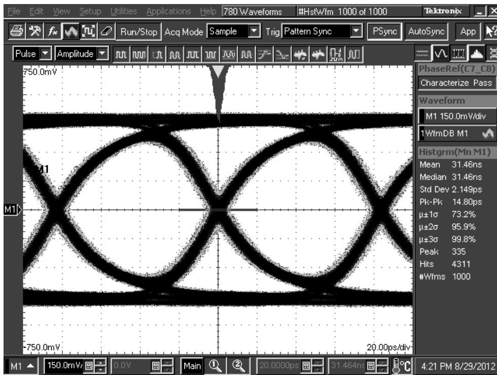
Figure 20. TL = 30 inch 5-mil FR4 trace, 12 Gbps DS125BR800 settings: EQ[1:0] = R, 0 = 07'h, DEM[1:0] = 0, 1
