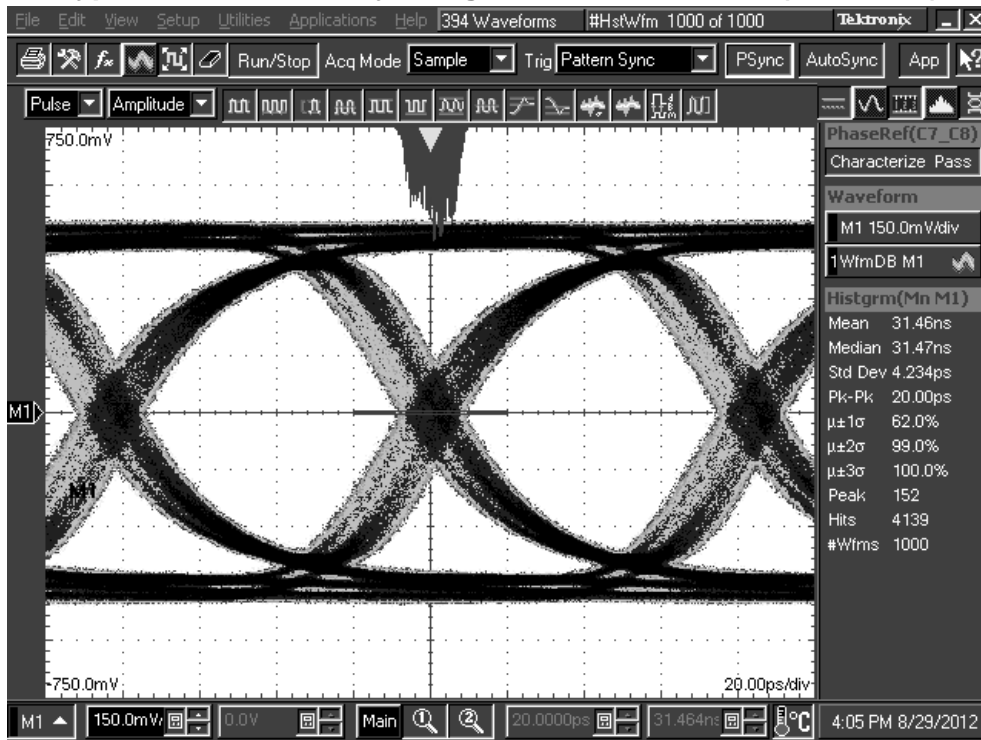
Figure 21. TL1 = 5-meter 30-AWG 100 Ohm Twin-axial Cable, 12 Gbps DS125BR800 settings: EQ[1:0] = R, 0 = 07'h, DEM[1:0] = 0, 1
