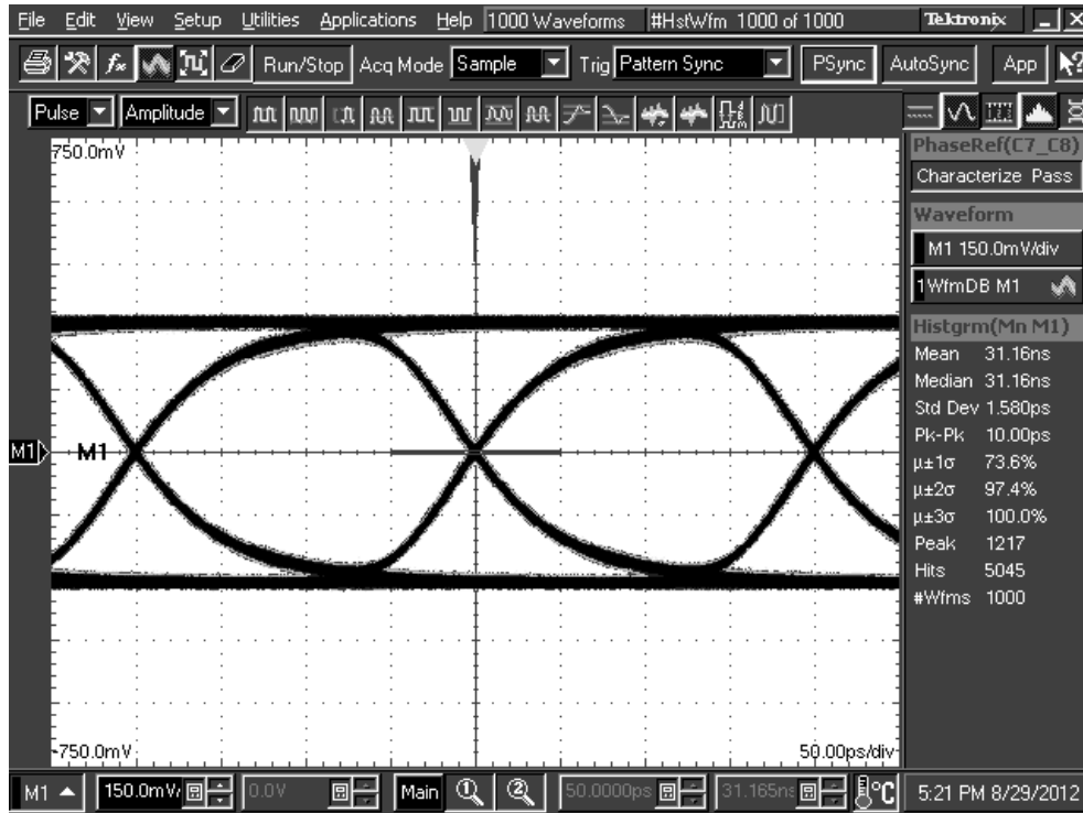
Figure 24. TL1 = 20 inch 5-mil FR4 trace, TL2 = 10 inch 5-mil FR4 trace, 5 Gbps DS125BR800 settings: EQ[1:0] = 0, 1 = 03'h, DEM[1:0] = R, 0
