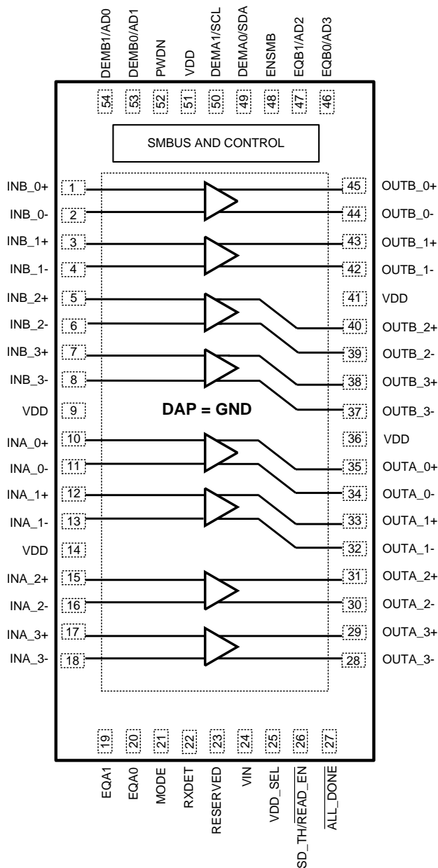
Figure 1. DS125BR800 Pin Diagram 54 lead
