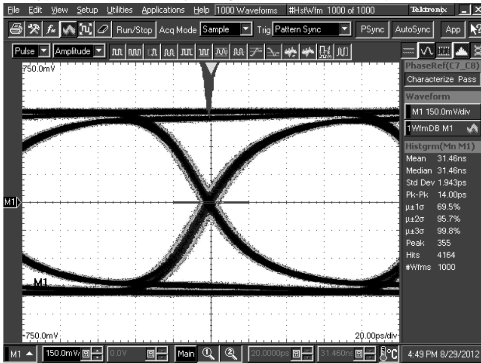
Figure 19. TL = 30 inch 5-mil FR4 trace, 8 Gbps DS125BR800 settings: EQ[1:0] = R, 0 = 07'h, DEM[1:0] = 0, 1
