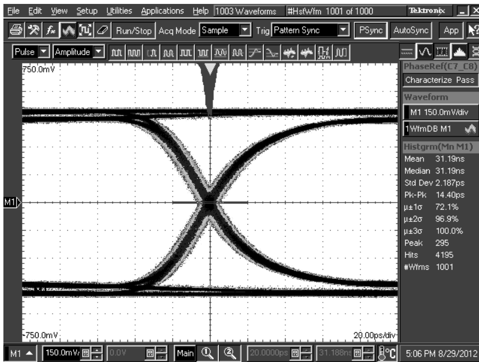
Figure 18. TL = 30 inch 5-mil FR4 trace, 5 Gbps DS125BR800 settings: EQ[1:0] = R, 0 = 07'h, DEM[1:0] = 0, 1
