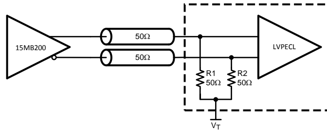
Figure 6. DC Coupled LVDS to LVPECL Interface
