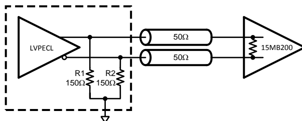
Figure 4. DC Coupled LVPECL to LVDS Interface
