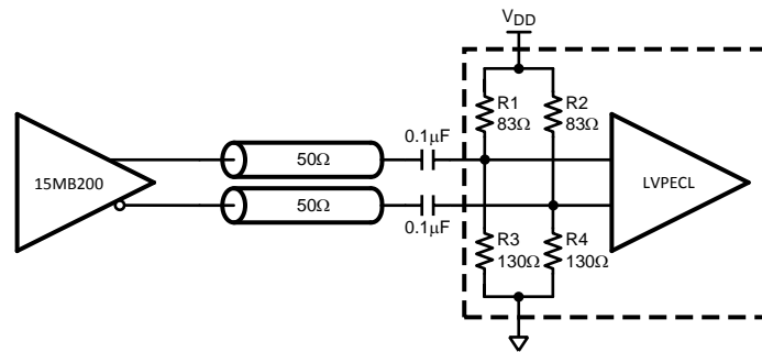
Figure 7. AC Coupled LVDS to LVPECL Interface
