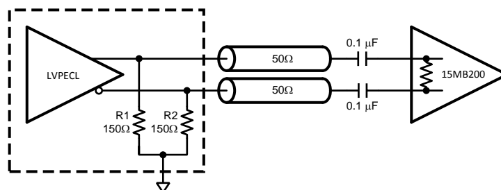
Figure 5. AC Coupled LVPECL to LVDS Interface
