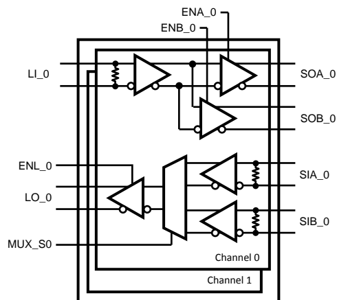
Figure 1. DS08MB200 Block Diagram
