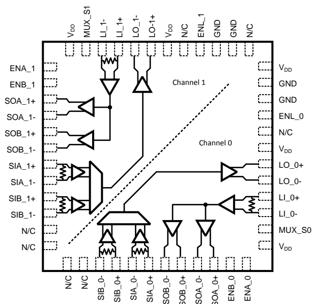
Figure 3. Directional Signal Paths Top View (Refer to pin names for signal polarity)
