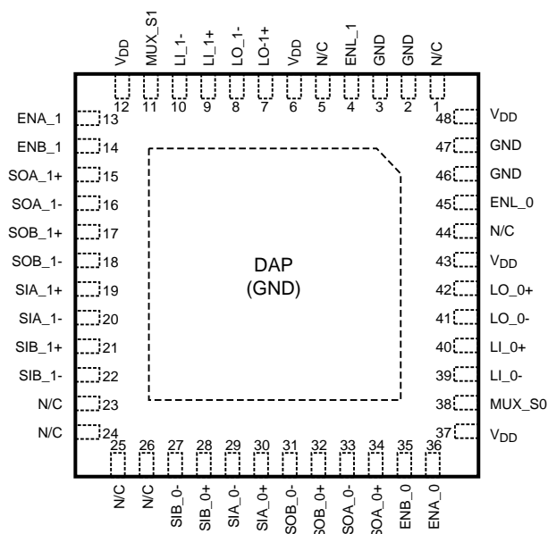
Figure 2. Top View DAP = GND
