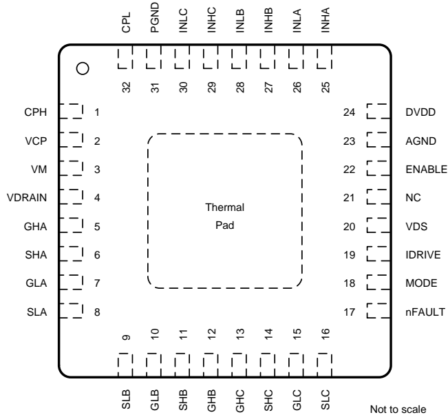
Pin Functions—32-Pin DRV8320 Devices
