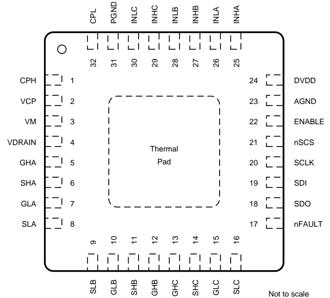
Pin Functions—32-Pin DRV8320 Devices
