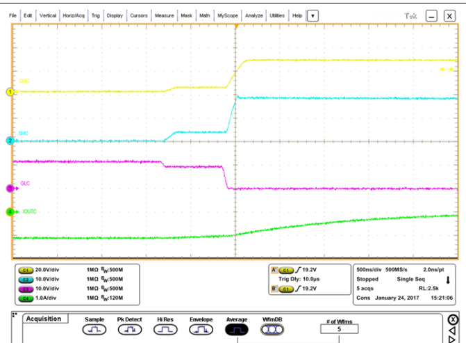
Figure 57. IDRIIVE Maximum Setting Negative Current
