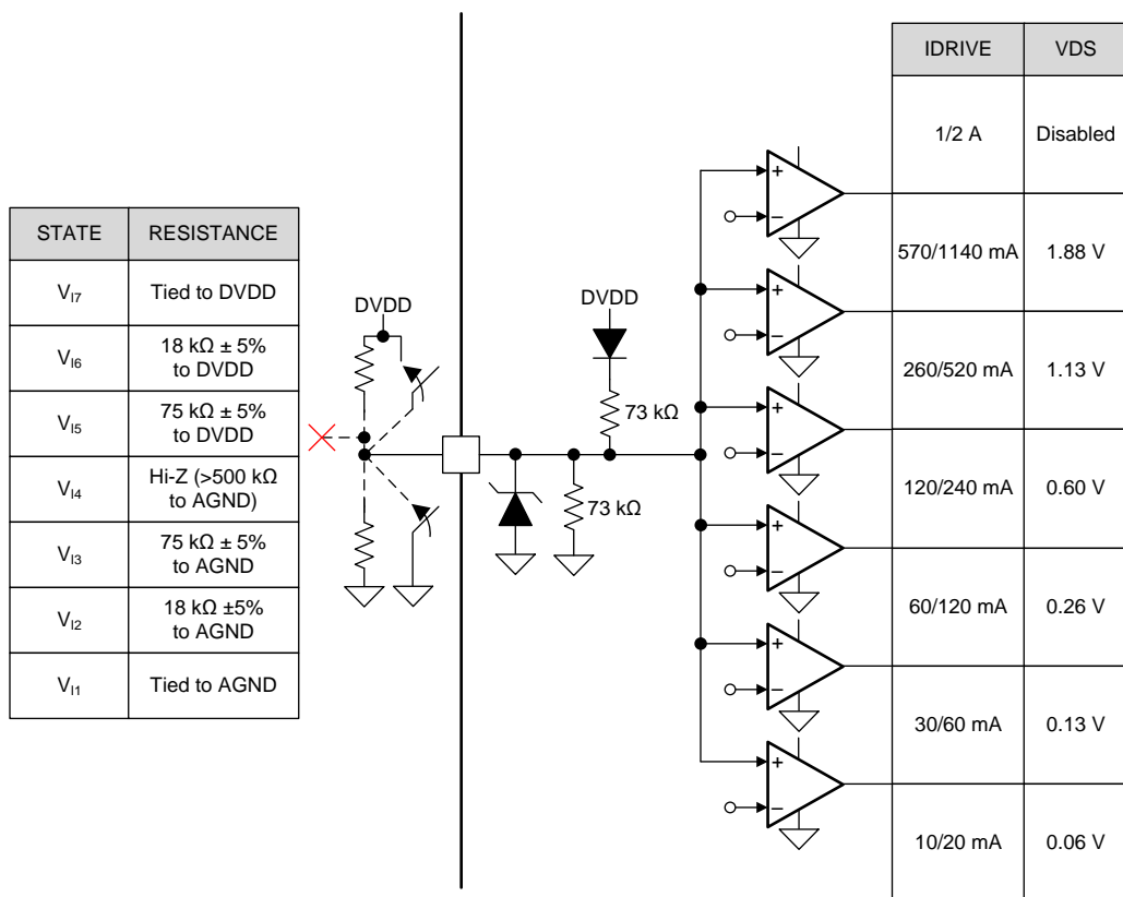
Figure 33 shows the structure of the seven level input pins, IDRIVE and VDS, on hardware interface devices. The input can be set with an external resistor.
