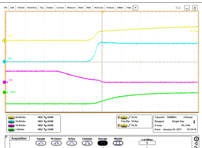
Figure 59. IDRIIVE Minimum Setting Negative Current
