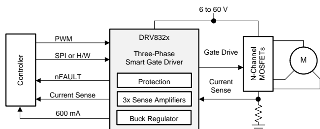
Simplified Schematic
