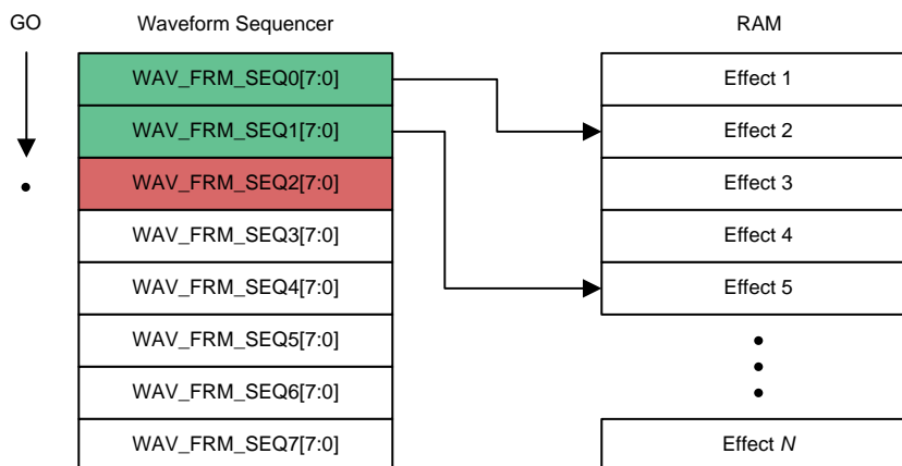
Figure 33. Waveform Sequencer Programming
