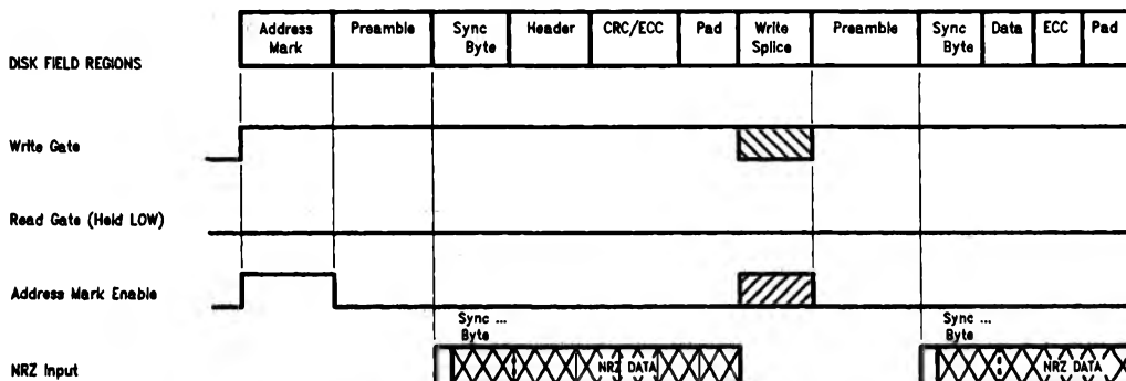
Write Cycle
