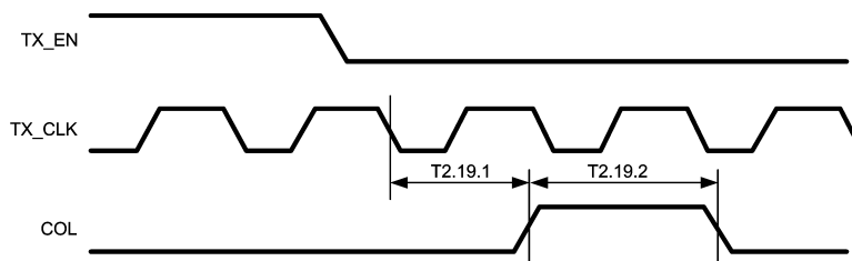
Figure 3-19. 10 Mb/s Heartbeat Timing
