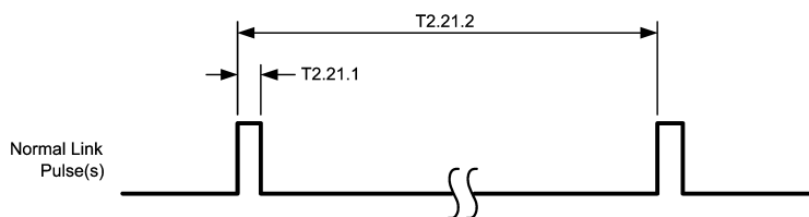
Figure 3-21. 10BASE-T Normal Link Pulse Timing
