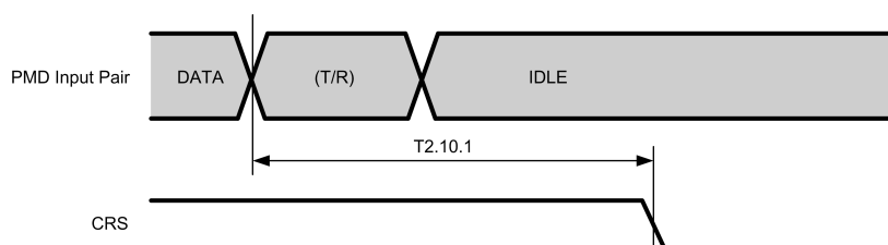
Figure 3-10. 100BASE-TX Receive Packet Deassertion Timing
