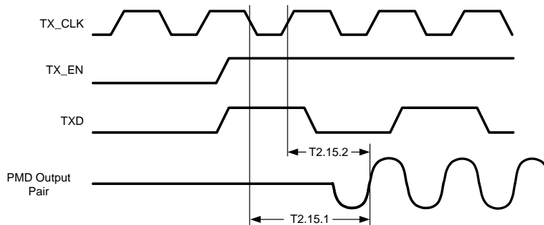
Figure 3-15. 10BASE-T Transmit Timing (Start of Packet)
