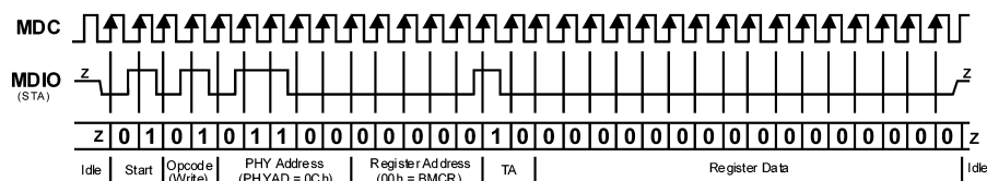
Figure 2-5. Typical MDC/MDIO Write Operation
