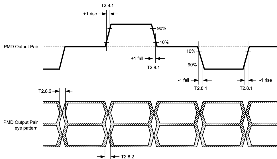
Figure 3-8. 100BASE-TX Transmit Timing ( t_{R/F} & Jitter)
