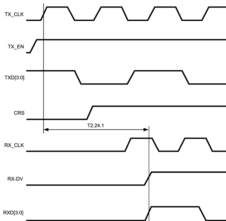
Figure 3-24. 100 Mb/s Internal Loopback Timing
