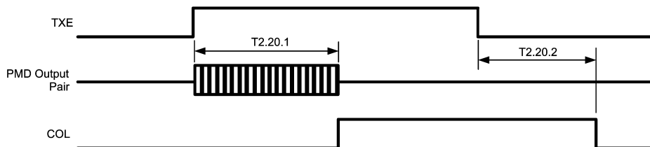
Figure 3-20. 10 Mb/s Jabber Timing
