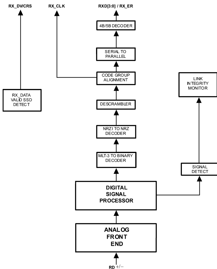
Figure 2-7. 100BASE-TX Receive Block Diagram
