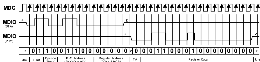
Figure 2-4. Typical MDC/MDIO Read Operation
