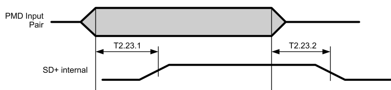
Figure 3-23. 100BASE-TX Signal Detect Timing
