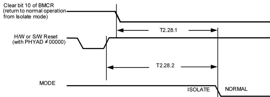
Figure 3-28. Isolation Timing
