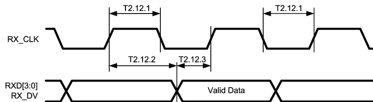
Figure 3-12. 10 Mb/s MII Receive Timing
