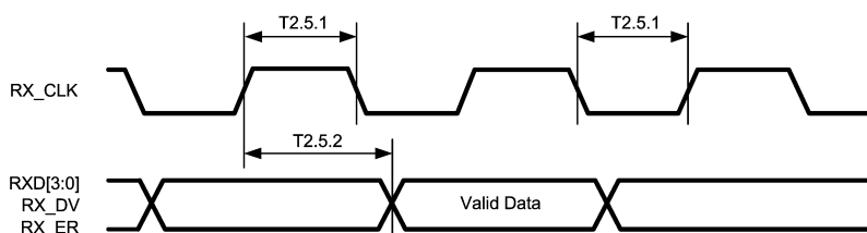
Figure 3-5. 100 Mb/s MII Receive Timing
