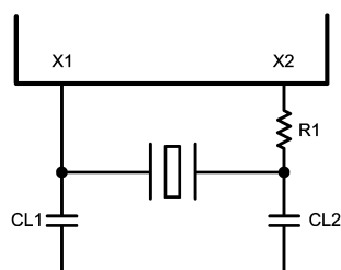
Figure 2-12. Crystal Oscillator Circuit
