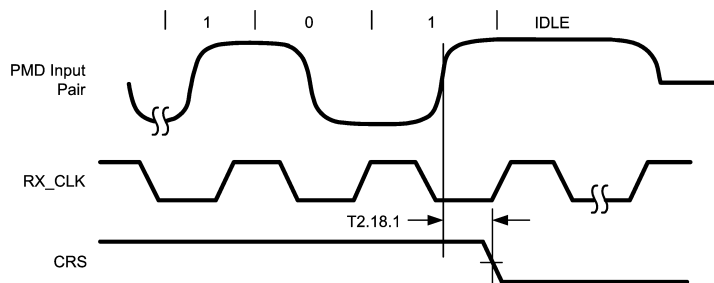
Figure 3-18. 10BASE-T Receive Timing (End of Packet)
