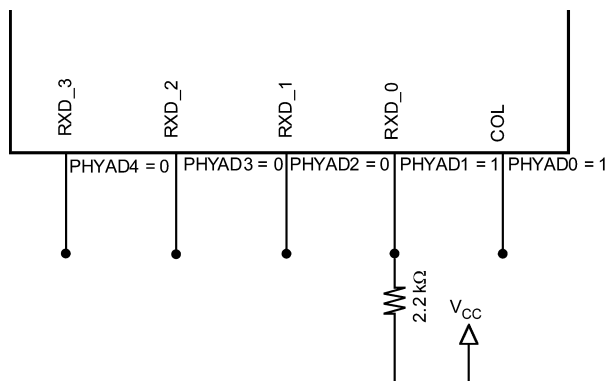
Figure 2-2. PHYAD Strapping Example
