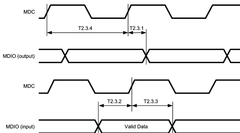
Figure 3-3. MII Serial Management Timing
