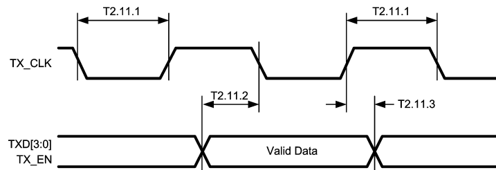
Figure 3-11. 10 Mb/s MII Transmit Timing
