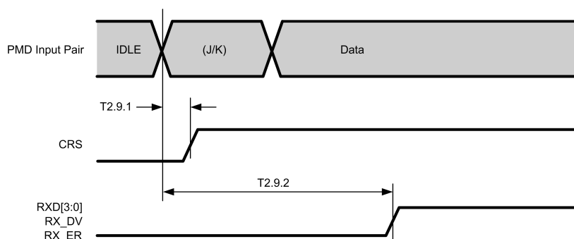
Figure 3-9. 100BASE-TX Receive Packet Latency Timing
