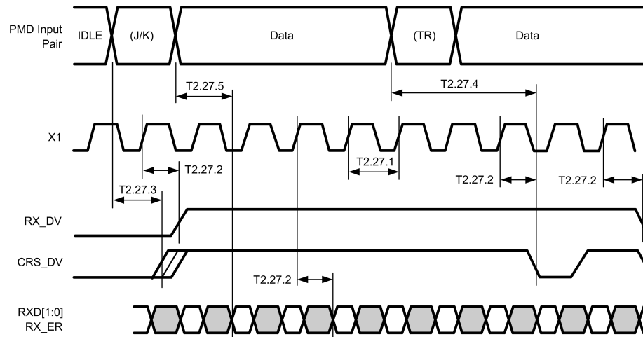
Figure 3-27. RMII Receive Timing
