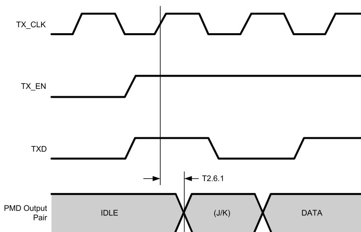
Figure 3-6. 100BASE-TX and 100BASE-FX MII Transmit Packet Latency Timing
