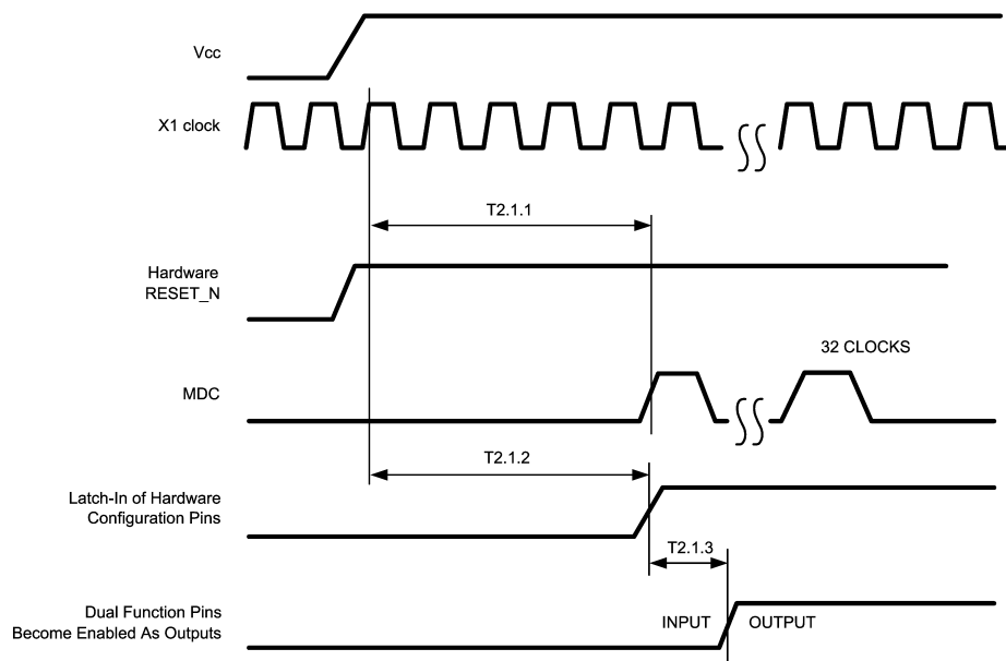
Figure 3-1. Power Up Timing
