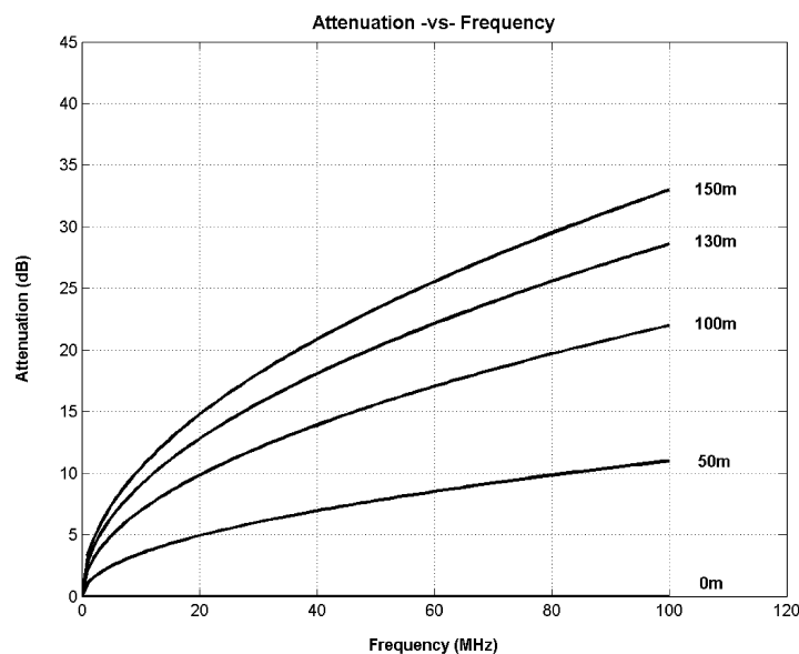
Figure 2-8. EIA/TIA Attenuation vs. Frequency for 0, 50, 100, 130 & 150 Meters of CAT 5 Cable
