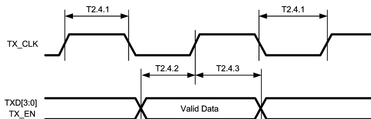
Figure 3-4. 100 Mb/s MII Transmit Timing
