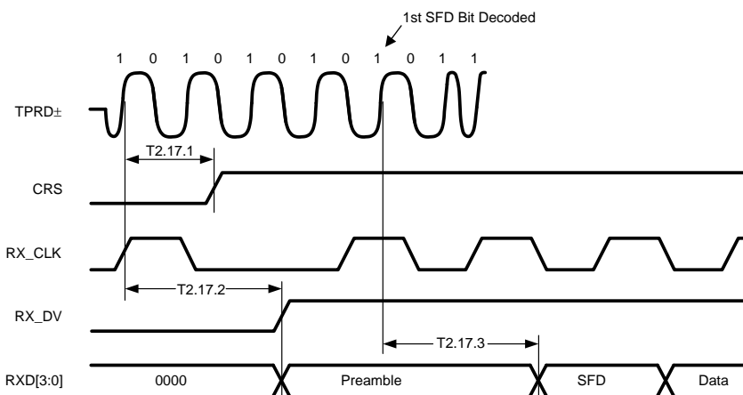
Figure 3-17. 10BASE-T Receive Timing (Start of Packet)
