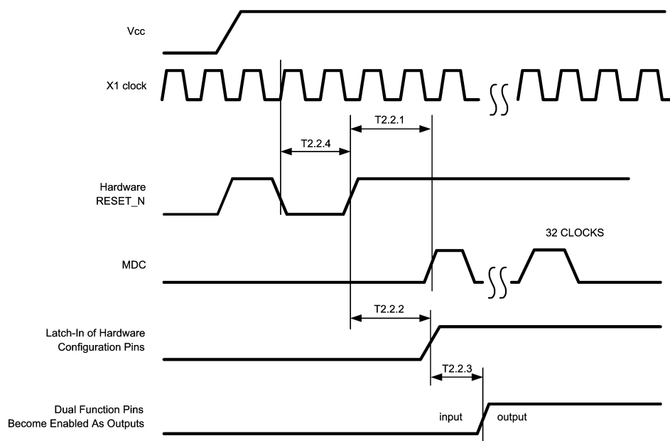
Figure 3-2. Reset Timing
