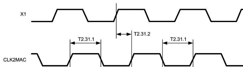
Figure 3-29. 25 MHz_OUT Timing
