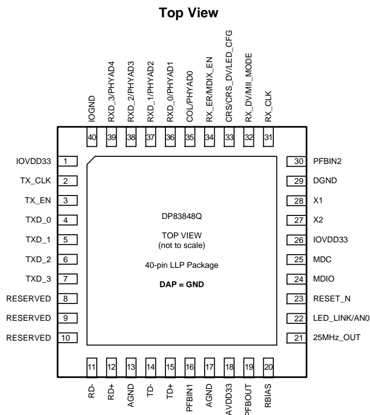
Figure 2-1. WQFN Package See Package Number RTA0040A
