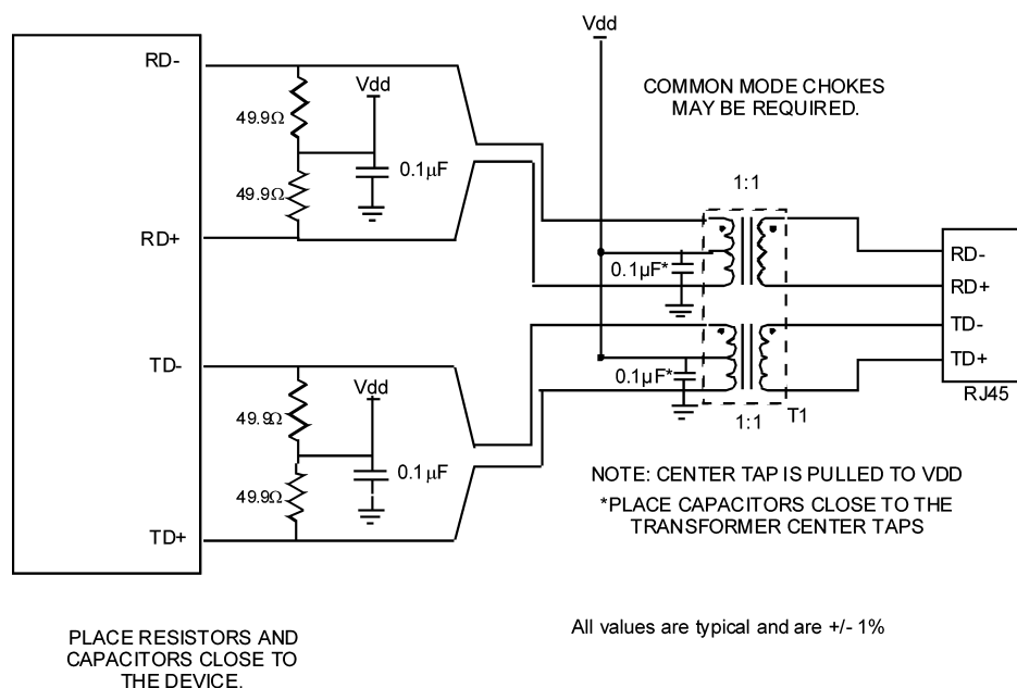
Figure 2-11. 10/100 Mb/s Twisted Pair Interface
