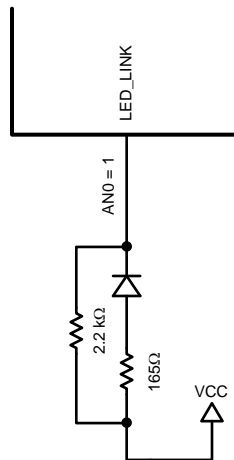
Figure 2-3. AN0 Strapping and LED Loading Example
