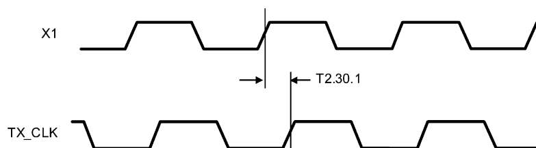
Figure 3-30. 100 Mb/s X1 to TX_CLK Timing
