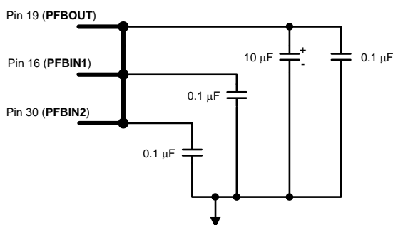
Figure 2-13. Power Feedback Connection
