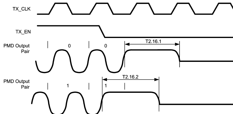
Figure 3-16. 10BASE-T Transmit Timing (End of Packet)
