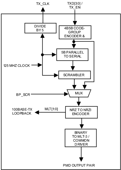
Figure 2-6. 100BASE-TX Transmit Block Diagram
