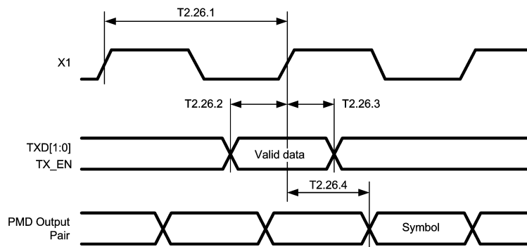
Figure 3-26. RMII Transmit Timing
