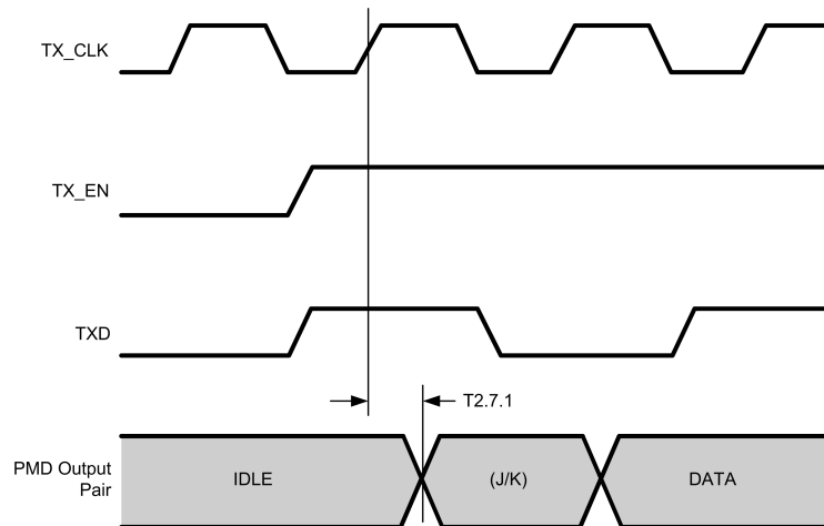
Figure 3-7. 100BASE-TX Transmit Packet Deassertion Timing
