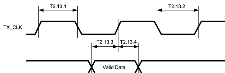
Figure 3-13. 10 Mb/s Serial Mode Transmit Timing
