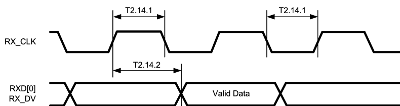
Figure 3-14. 10 Mb/s Serial Mode Receive Timing
