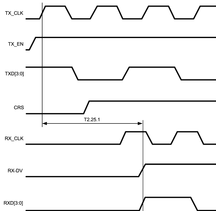
Figure 3-25. 10 Mb/s Internal Loopback Timing
