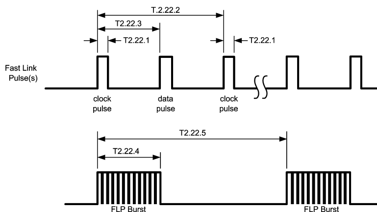
Figure 3-22. Auto-Negotiation Fast Link Pulse (FLP) Timing
