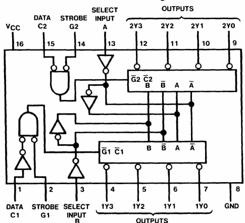
Dual-In-Line Package
