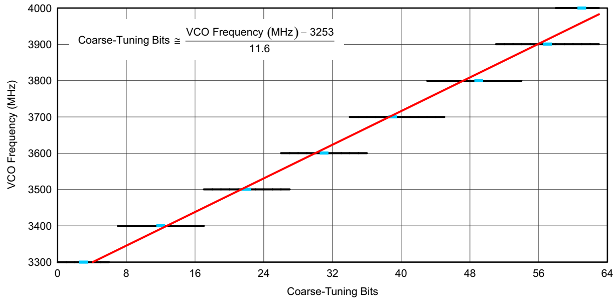
Figure 58. Typical PLL/VCO Lock Range vs Coarse Tuning Bits
