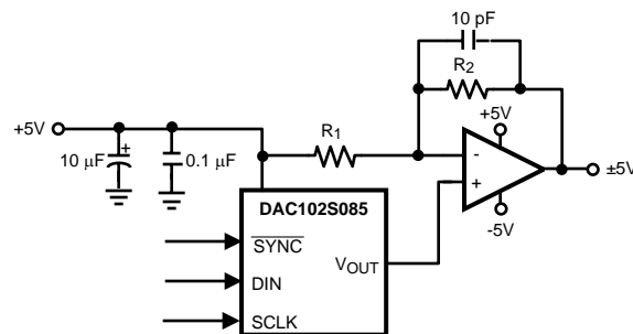
Figure 37. Bipolar Operation
