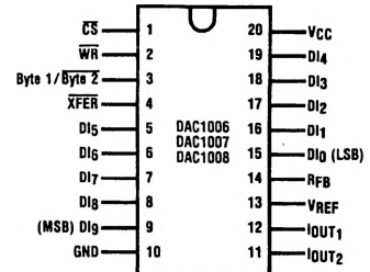
DAC1006/1007/1008 (20-Pin Parts) Dual-In-Line Package
