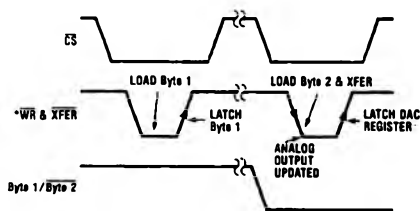
DAC1006/1007/1008 (20-Pin Parts)
