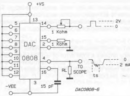
FIGURE 14. Reference Current Slew Rate Measurement
