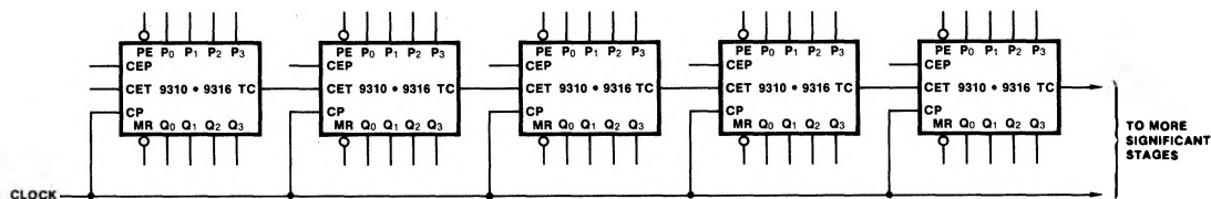
Fig. a Synchronous Multistage Counting Scheme (Slow)
