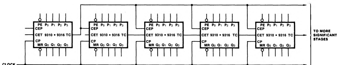
Fig. b Synchronous Multistage Counting Scheme (Fast)
