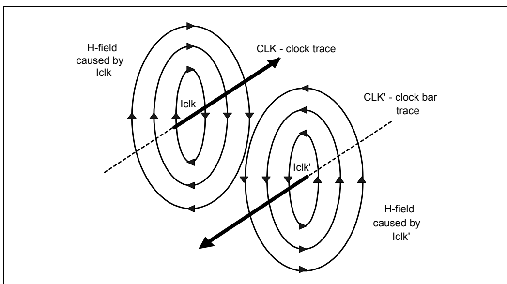
Figure 204. Cancellation of H-Fields through Inverse Currents
