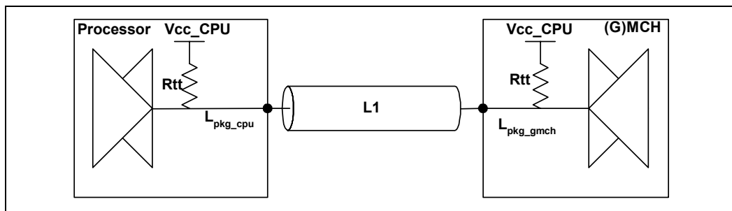
Figure 33. Topology 1
