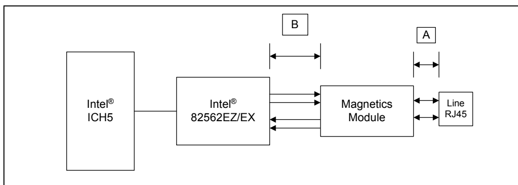
Figure 139. Critical Dimensions for Component Placement
