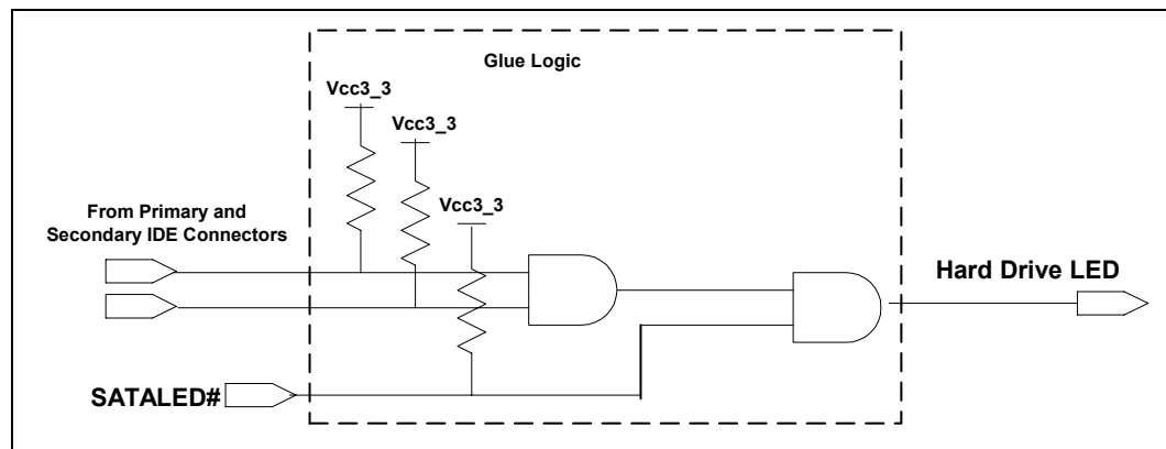
Figure 102. SATALED# Circuitry Example
