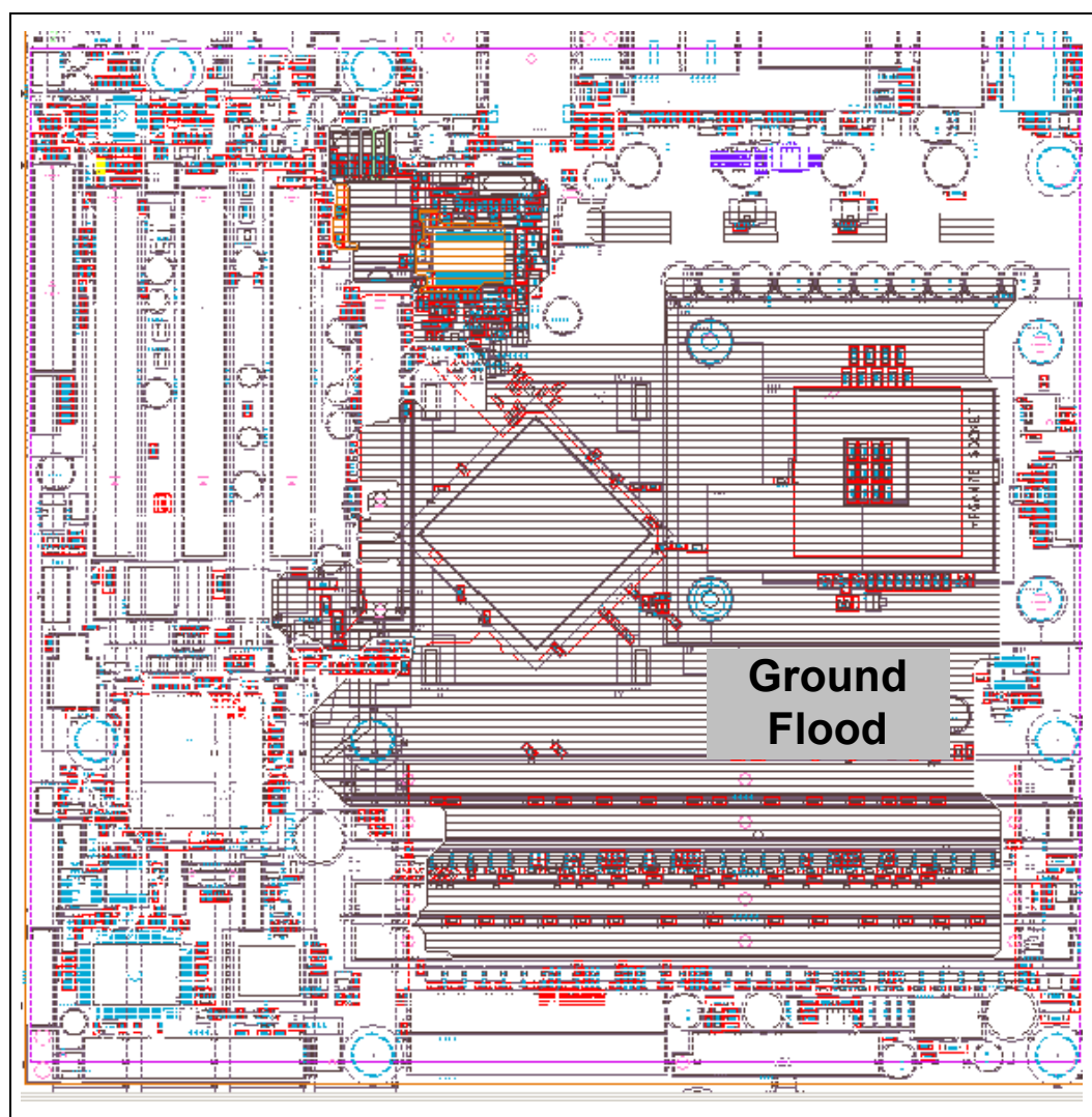
Figure 54. Example of Ground Flood on Layer 2
