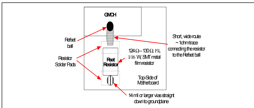
Figure 85. REFSET Placement
