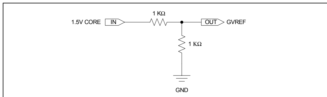
Figure 84. VREF Circuit for Intel® DVO Down Solution
