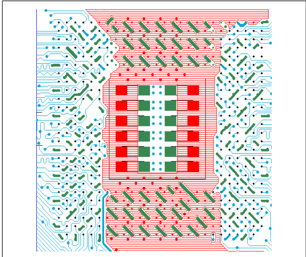
Figure 164. Capacitor Orientation
