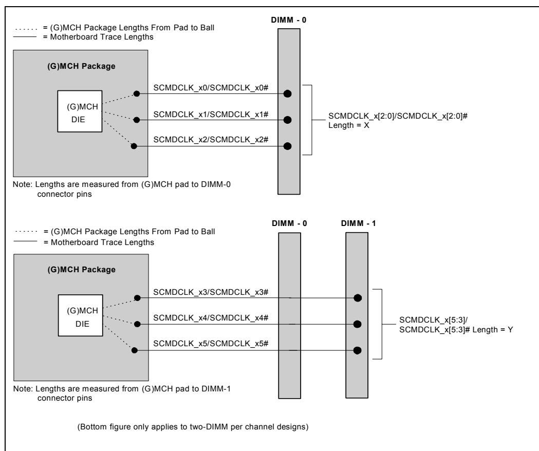
Figure 59. Differential Clock Trace Length Matching Requirements
