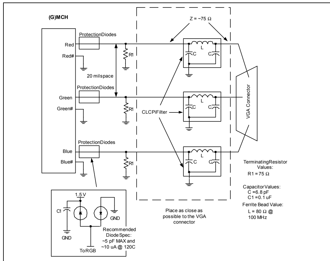
Figure 86. Ideal Single-Ended Routing Scheme Example
