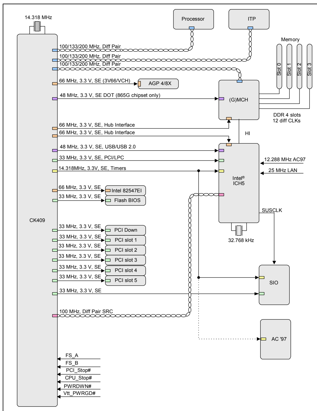
Figure 15. Intel® 865G/865PE Chipset-Based System Clocking Diagram
