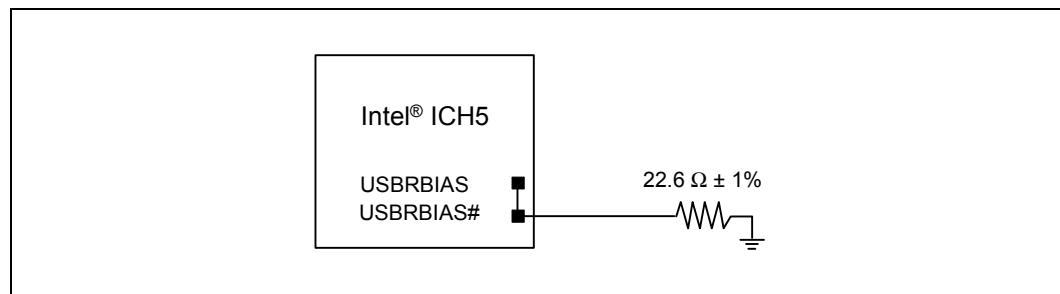
Figure 119. USBRBIAS/USBRBIAS# Connection
