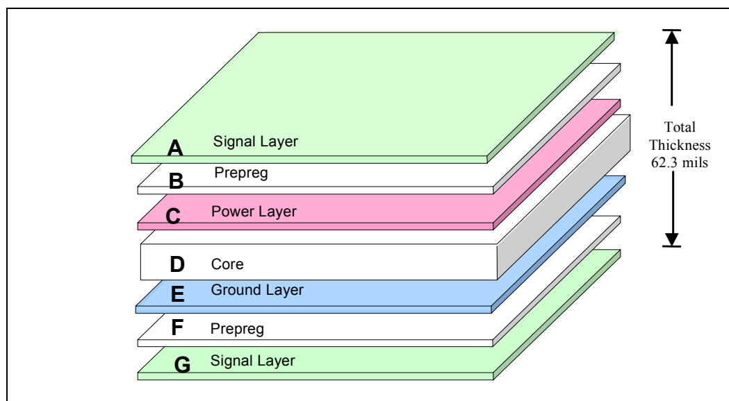
Figure 7. 4-Layer PCB Stack-Up Example
