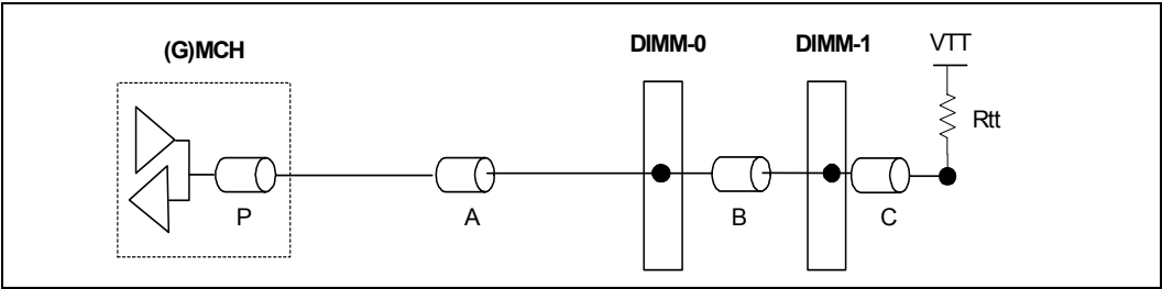
Figure 65. One DIMM per-Channel Data Signal Length Matching Topology
