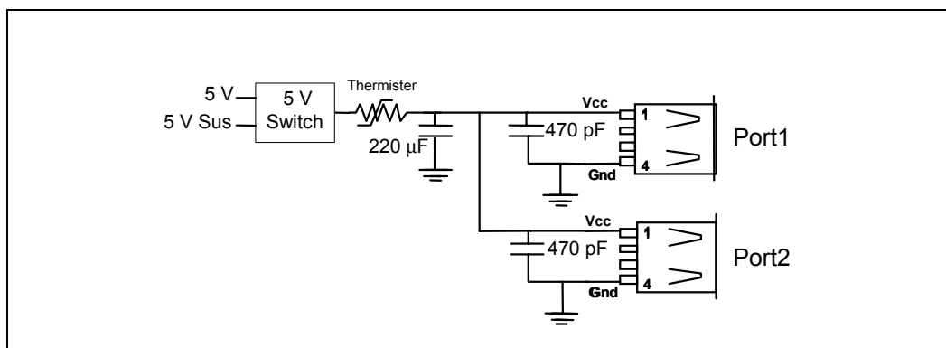
Figure 120. Good Downstream Power Connection
