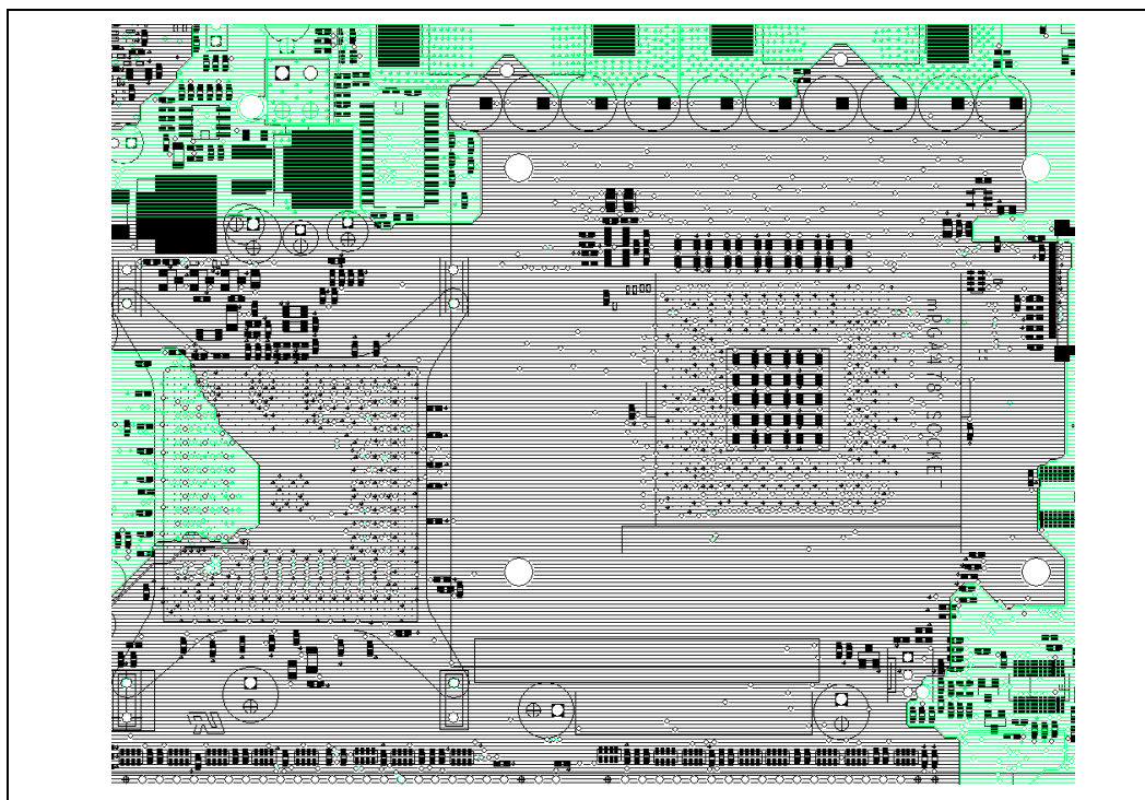
Figure 163. Bottom Layer Power Delivery Shape (VCC_CPU)
