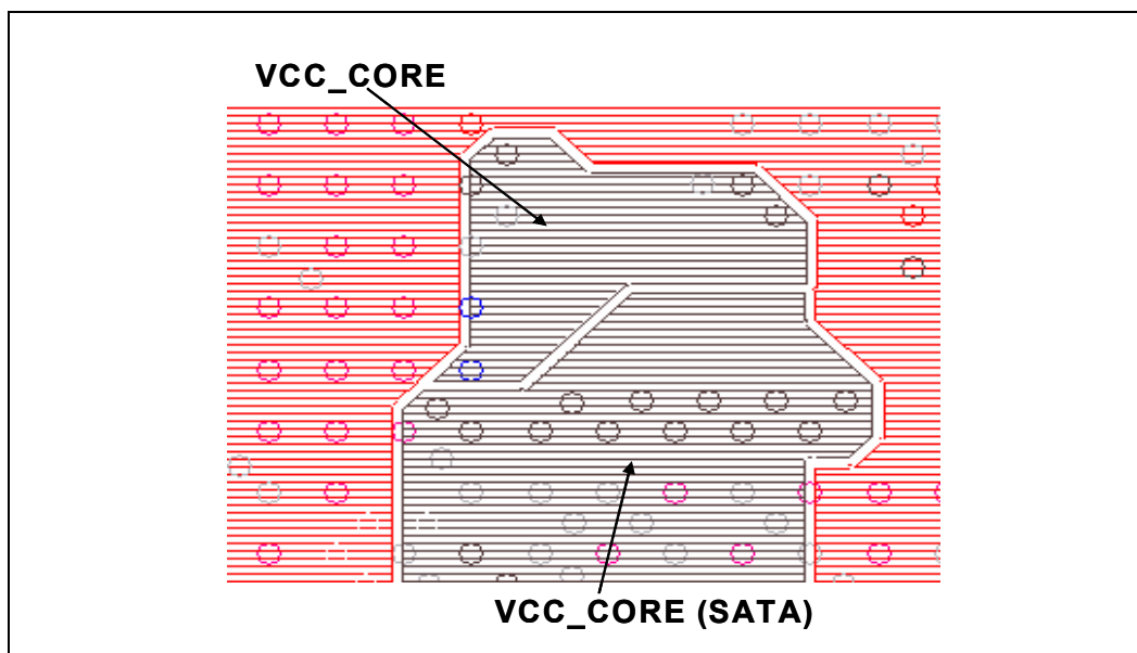
Figure 198. Intel® ICH5 Layer 4 Power Delivery
