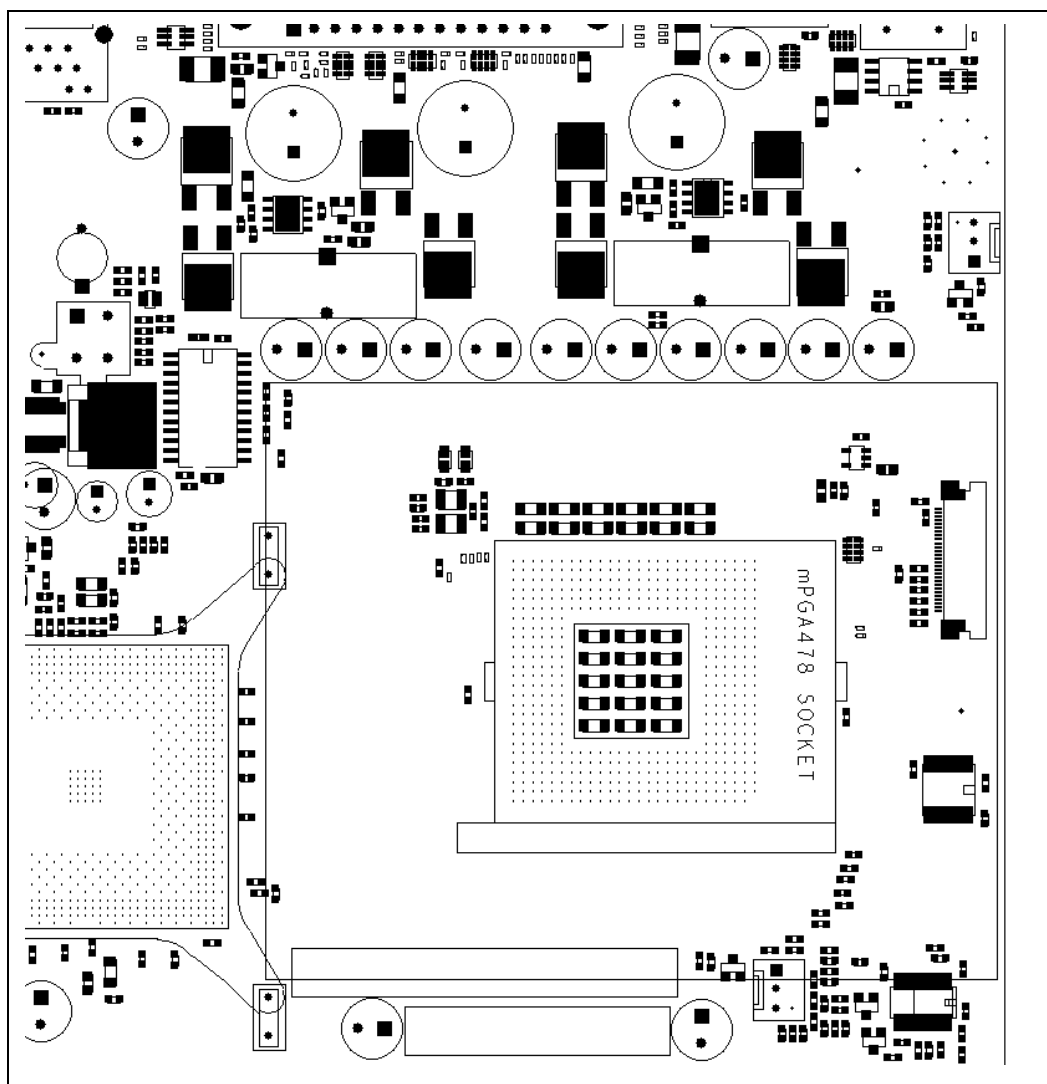
Figure 159. VR Component Placement
