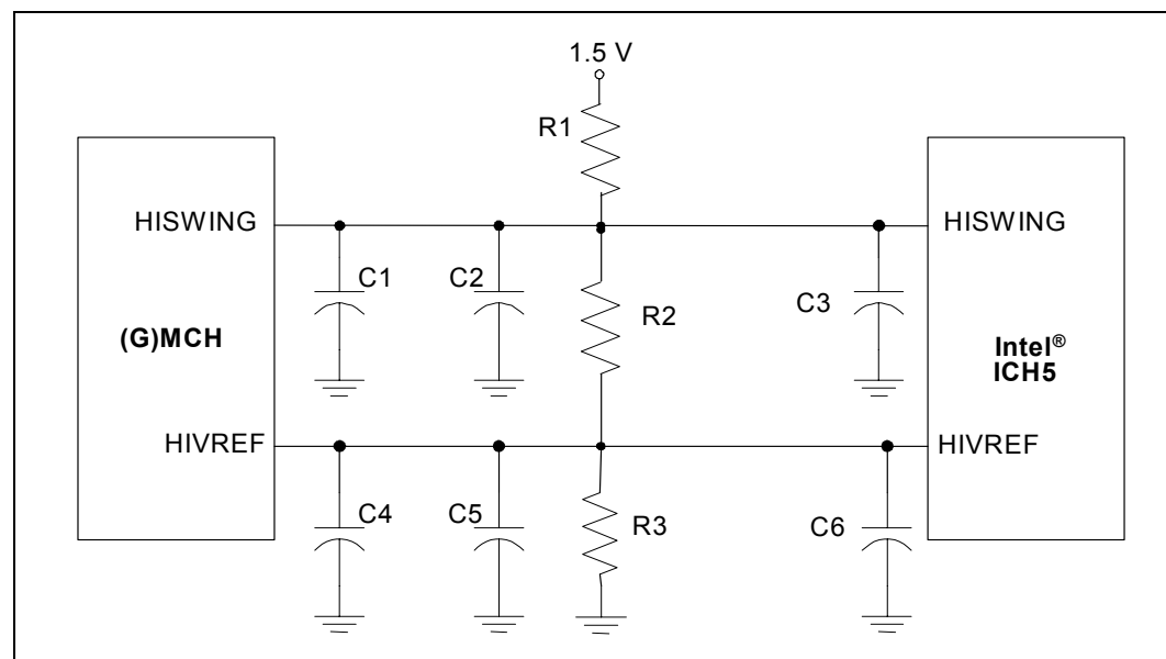
Figure 78. Hub Interface Single HIVREF/HISWING Generation Circuit
