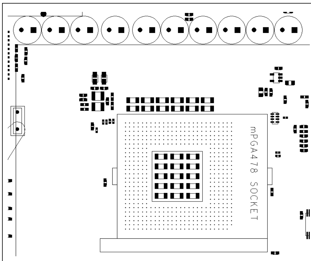
Figure 160. Decoupling Placement
