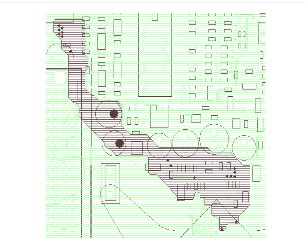
Figure 178. VCC_CPU Power Plane (Layer 2)
