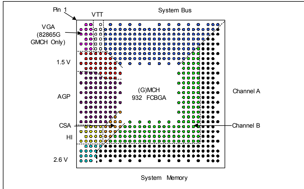
Figure 12. (G)MCH Component Quadrant Layout (Top View)
