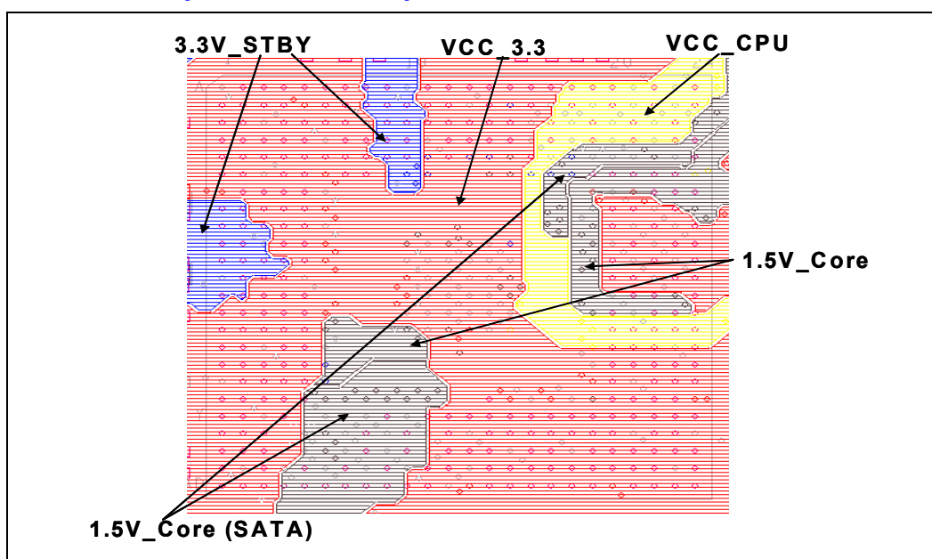
Figure 195. Intel® ICH5 Layer 2 Power Delivery
