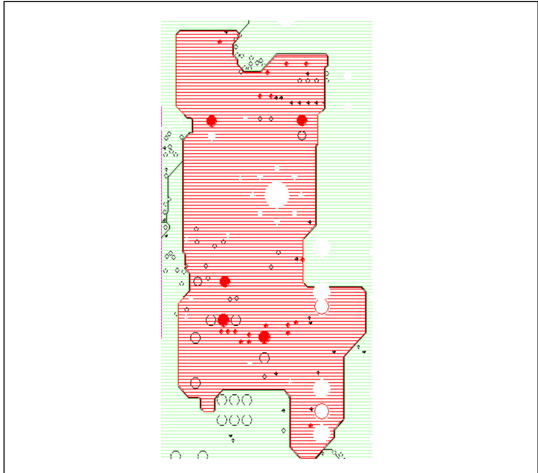
Figure 176. 2.6 V Layer 2 DDR Power Plane
