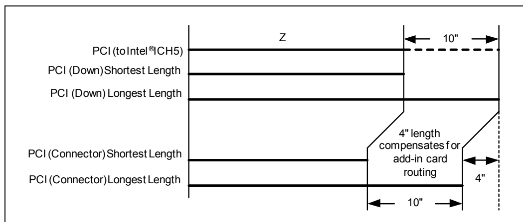
Figure 21. 33 MHz Clock Relationships
