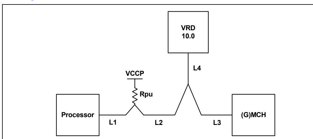
Figure 41. Routing Illustration for PROCHOT#
