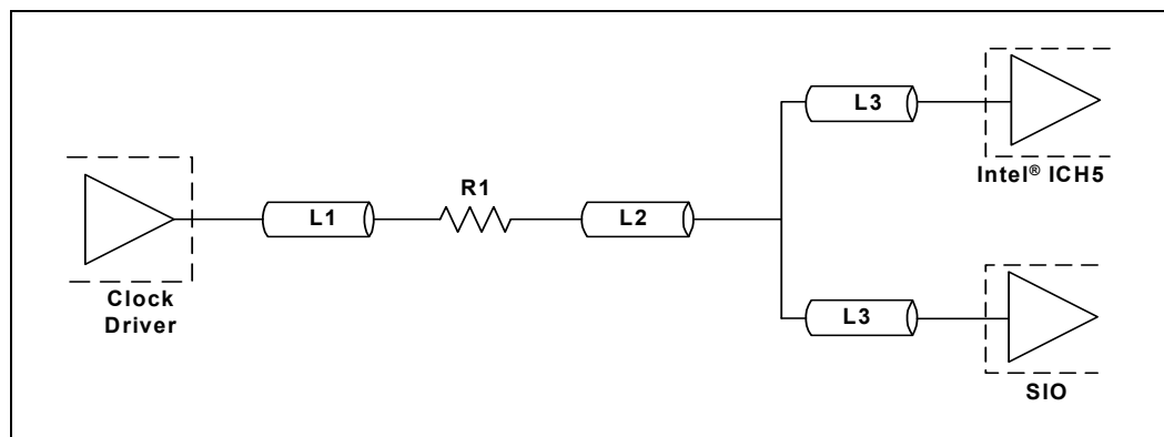
Figure 27. Topology for CLK14
