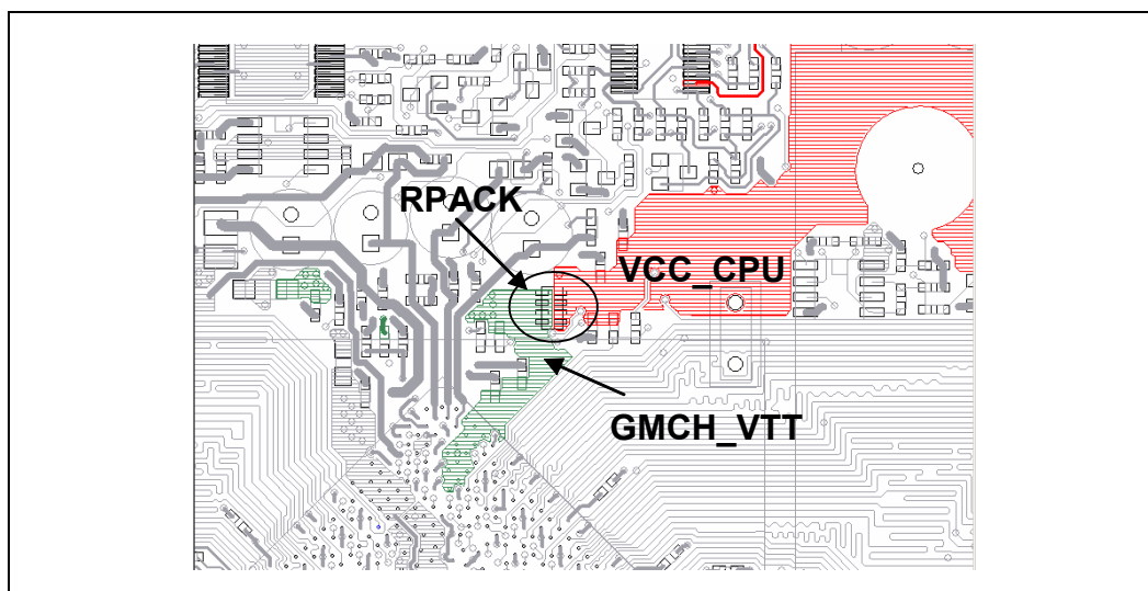
Figure 157. RPACK for Combining VCC_CPU and GMCH_VTT
