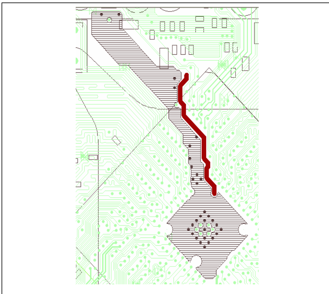
Figure 181. 1.5 V Power Plane (Layer 4)
