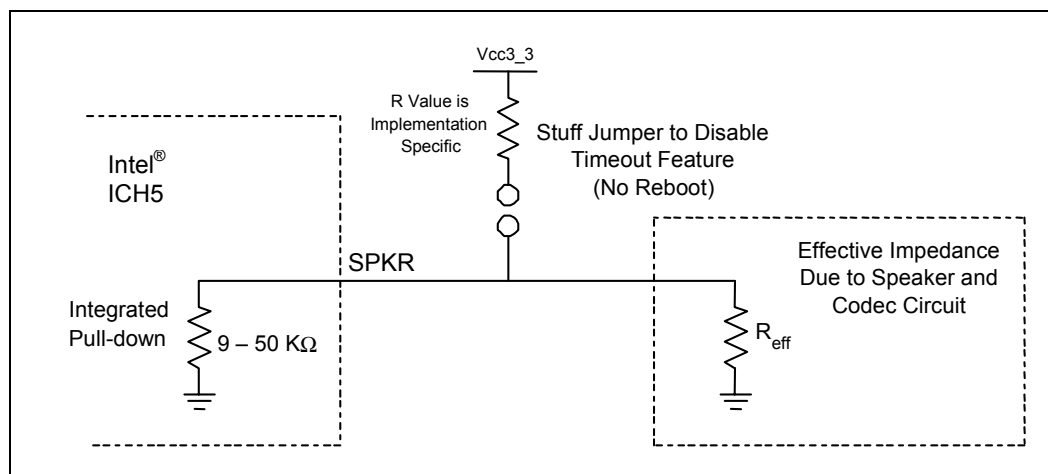
Figure 114. Example Speaker Circuit
