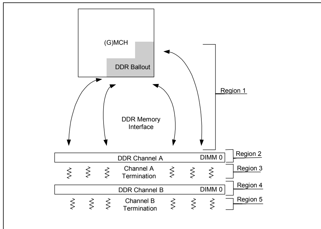
Figure 56. One DIMM per-Channel DDR Regions for Trace Width and Spacing
