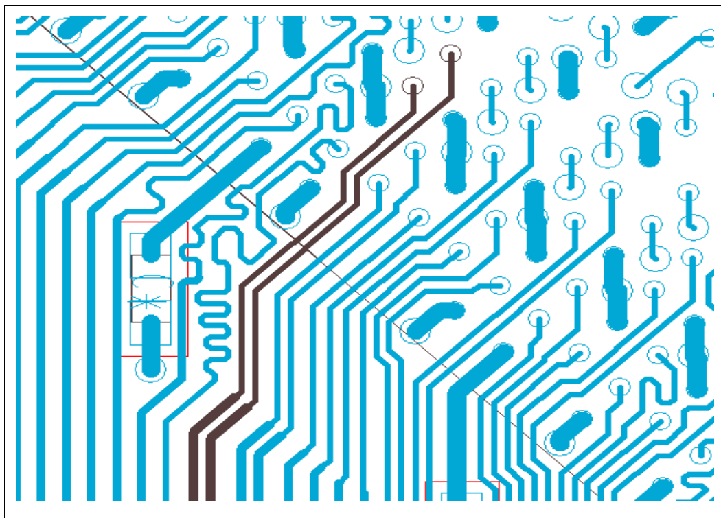
Figure 57. Example of DDR Clock Neckdown at (G)MCH
