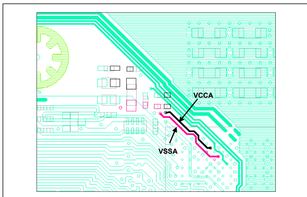
Figure 174. VCCA and VSSA Layer 4 Routing
