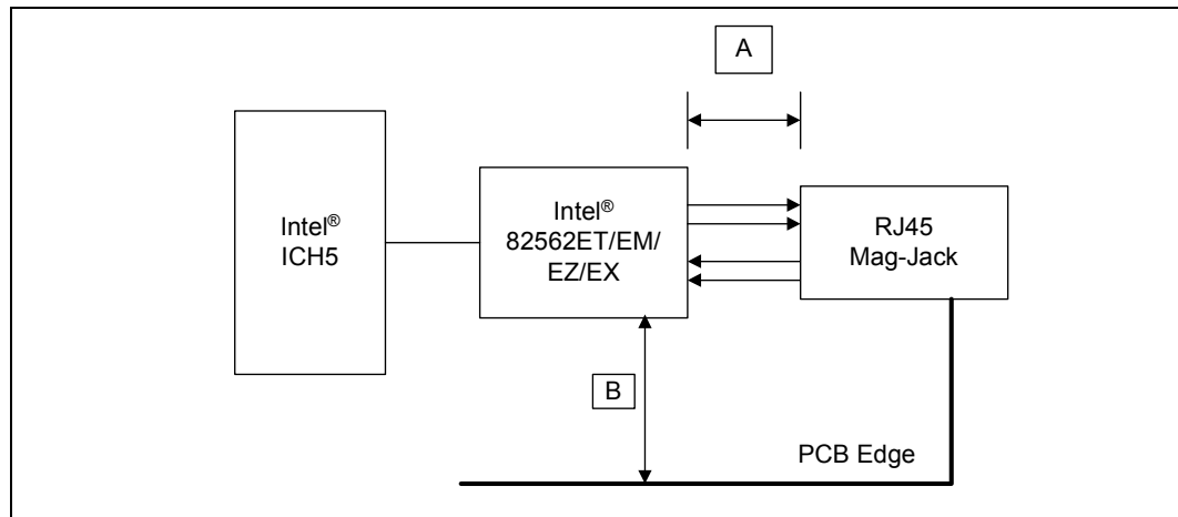
Figure 140. Critical Dimensions for Component Placement
