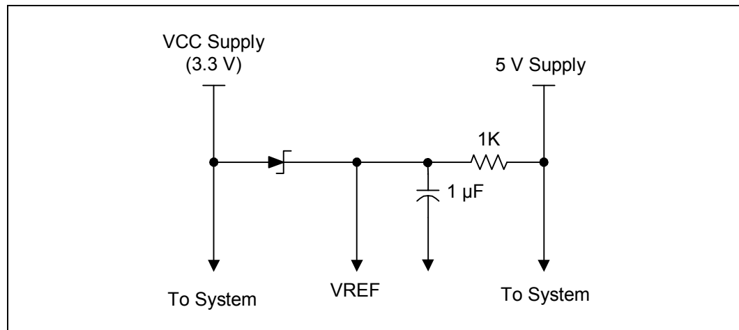
Figure 193. Example 3.3 V/V5REF Sequencing Circuitry
