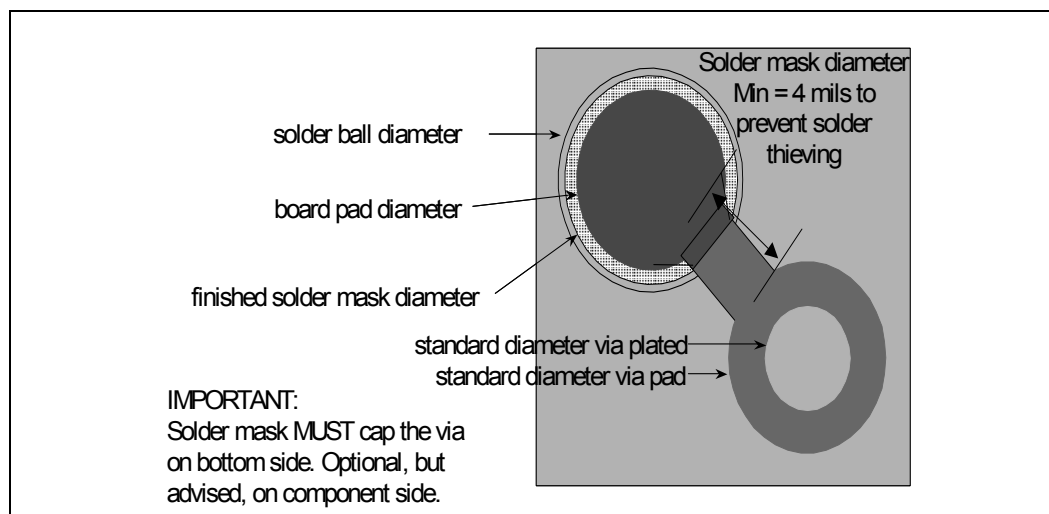
Figure 9. Via-Pad Layout Metal-Defined Pads
