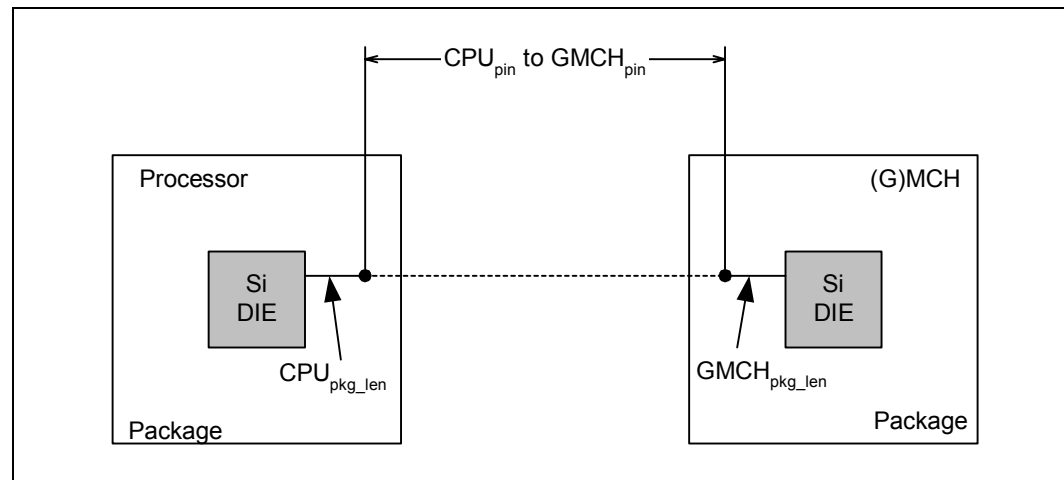
Figure 50. Trace Length Matching for the Front Side Bus
