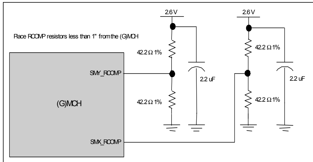
Figure 74. DDR (SMRCOMP) Resistive Compensation
