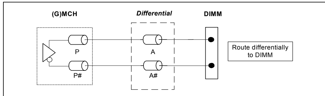
Figure 58. DDR Differential Clock Length Matching Topology
