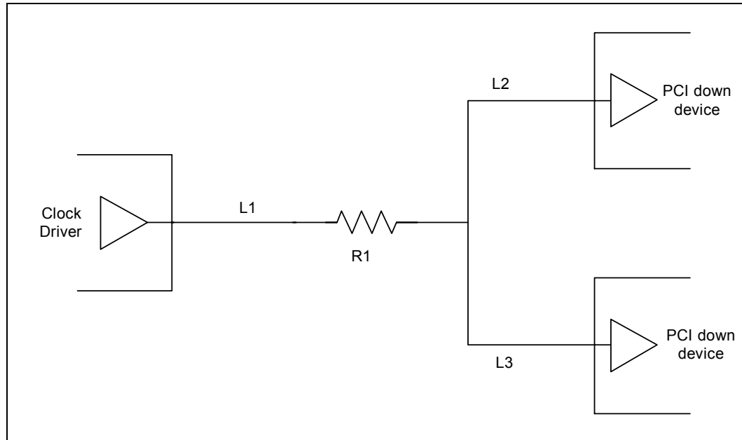
Figure 26. Topology for Sharing CLK33 between Two PCI Down Devices
