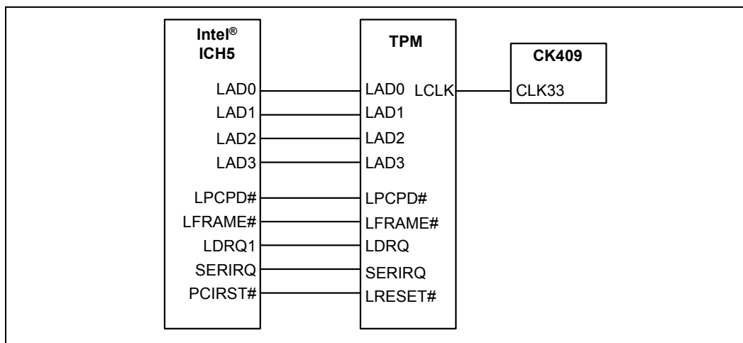
Figure 145. TPM LPC Block Diagram
