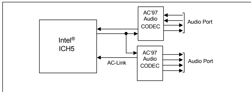
Figure 4. AC '97 with Audio Codecs (4 Channel Secondary)
