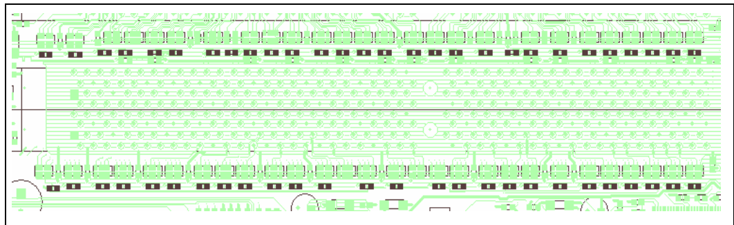
Figure 192. DDR DIMM VTT High-Speed Decoupling
