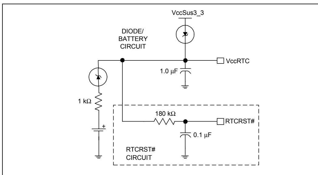
Figure 133. RTCRST# External Circuit for the Intel® ICH5 RTC
