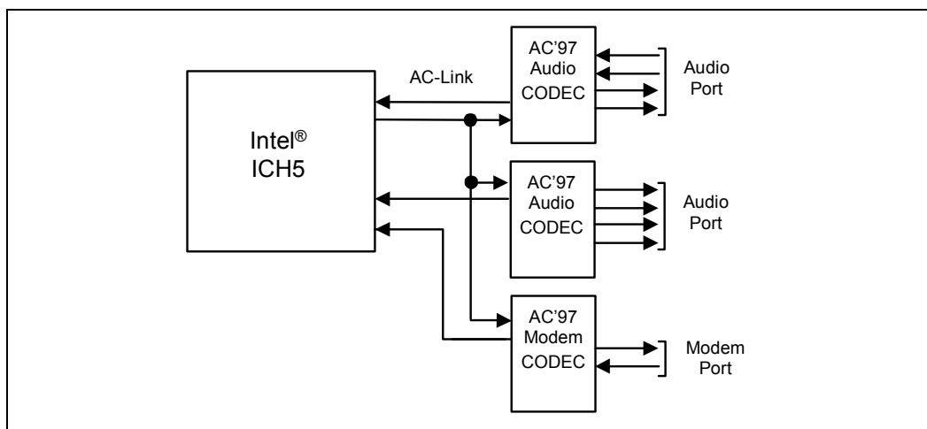
Figure 6. AC '97 with Audio and Modem Codec
