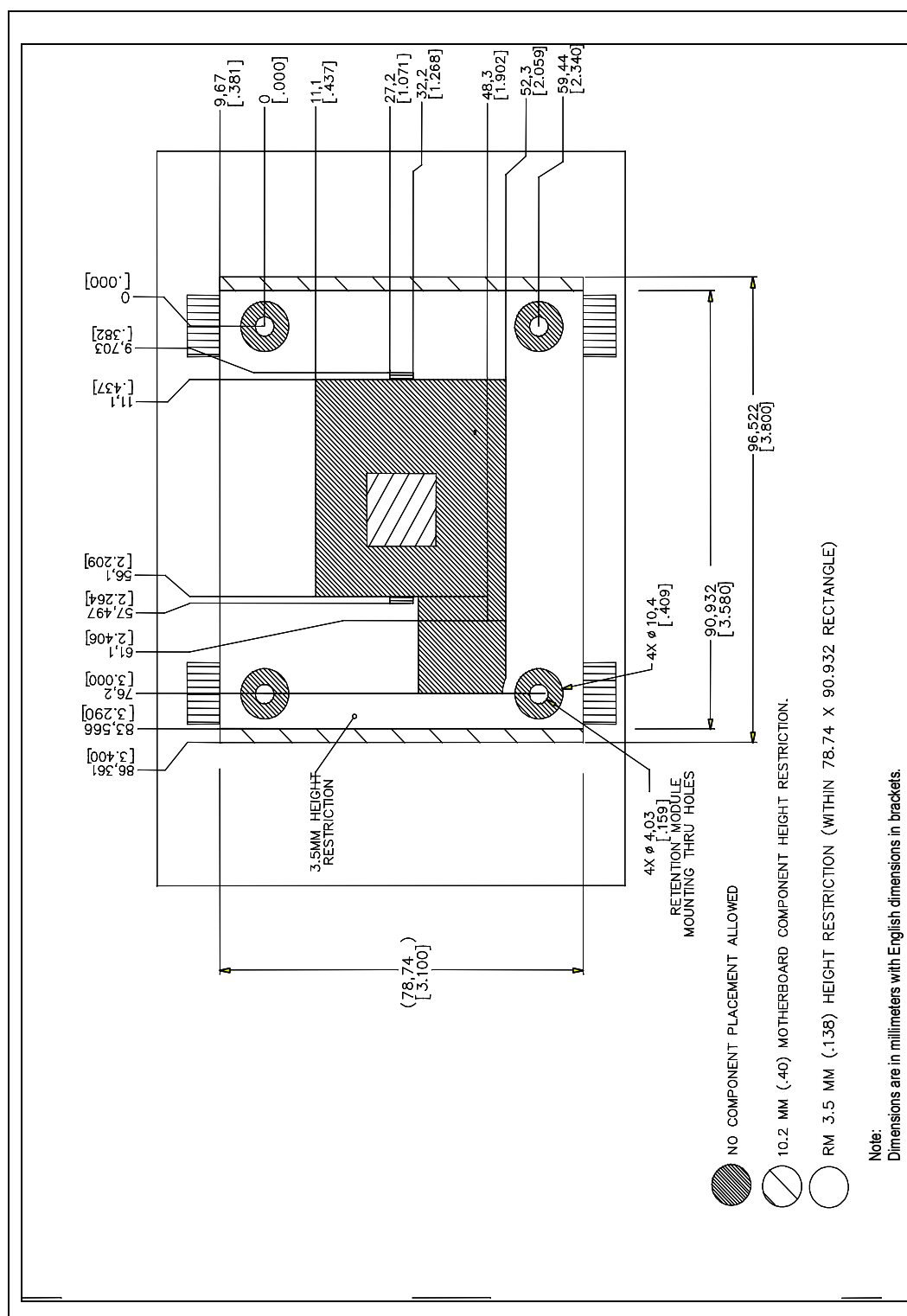
Figure 52. Retention Mechanism Keepout Drawing 2
