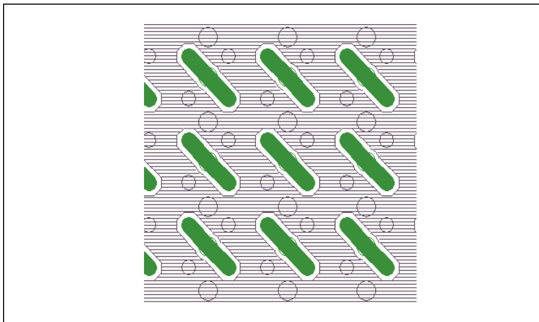
Figure 165. Shared Ground and Power Vias
