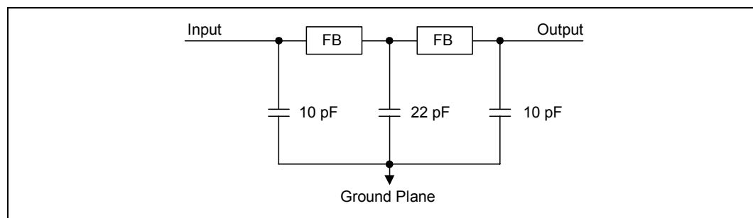
Figure 87. Alternate RGB Filter Recommendation
