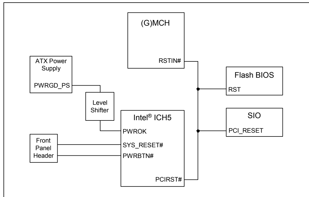
Figure 146. SYS_RESET# and PWRBTN# Connection
