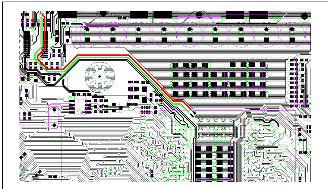
Figure 166. Routing of Feedback Signal
