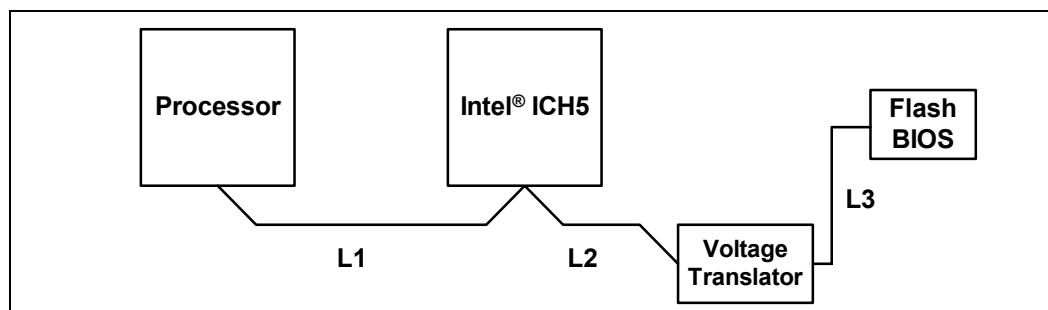
Figure 38. INIT# Topology
