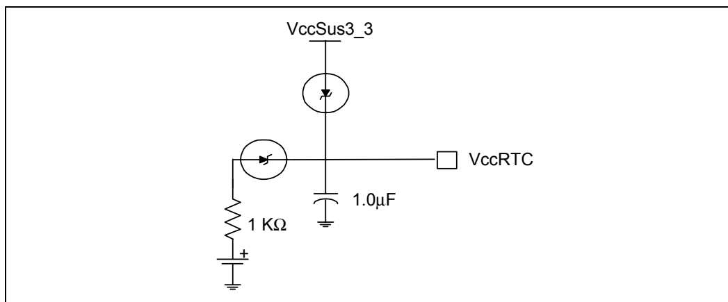
Figure 132. A Diode Circuit to Connect RTC External Battery
