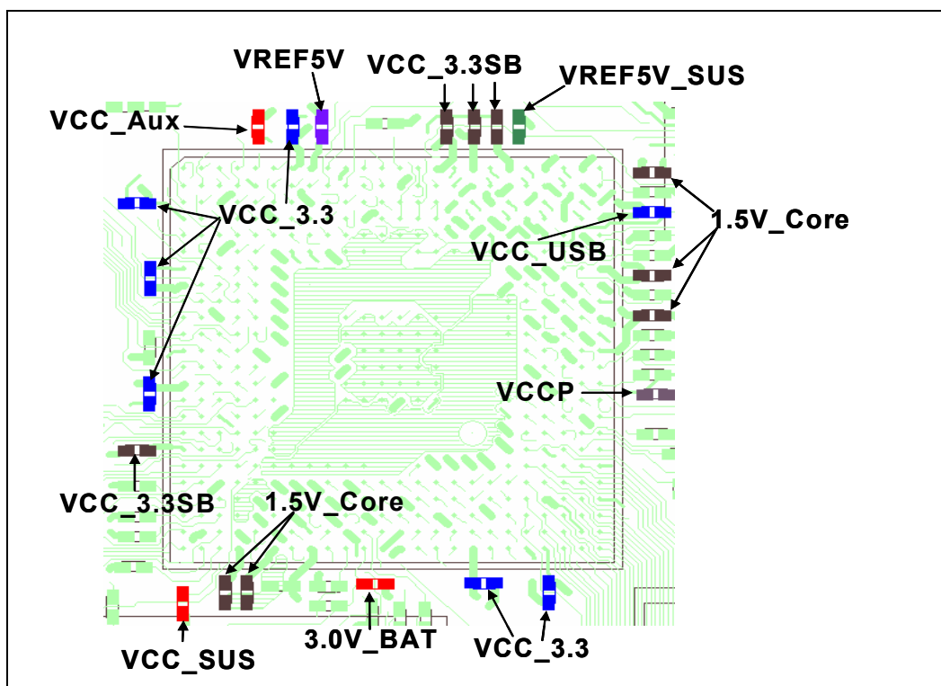
Figure 201. Intel® ICH5 Example Decoupling Capacitor Placement
