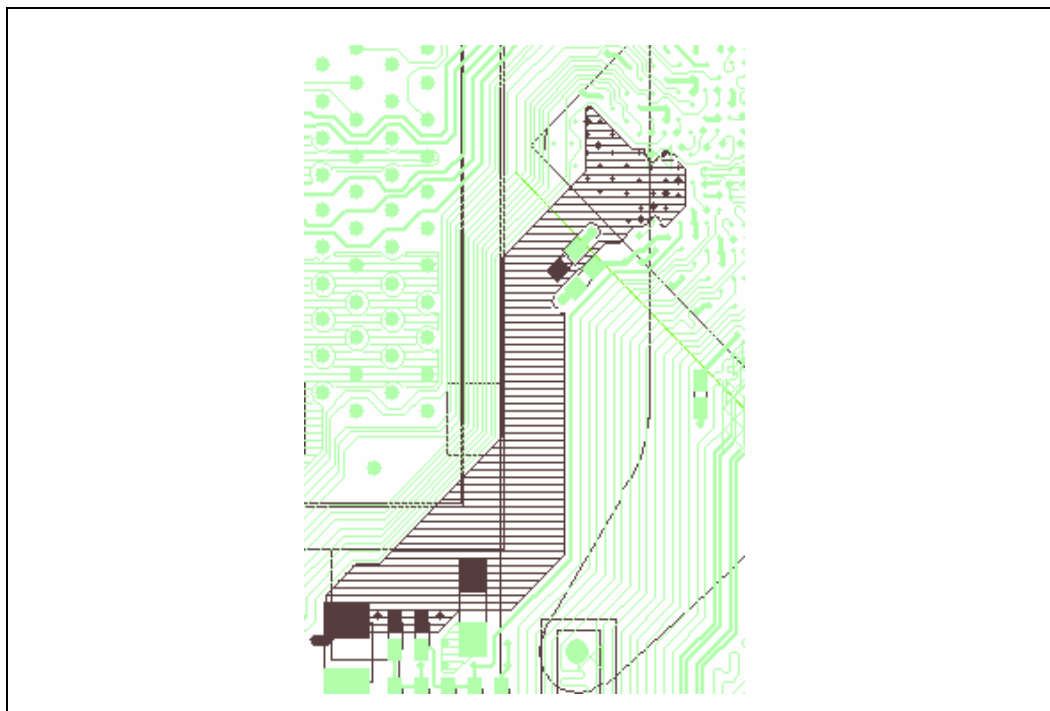
Figure 175. DDR Power Plane Layer 1
