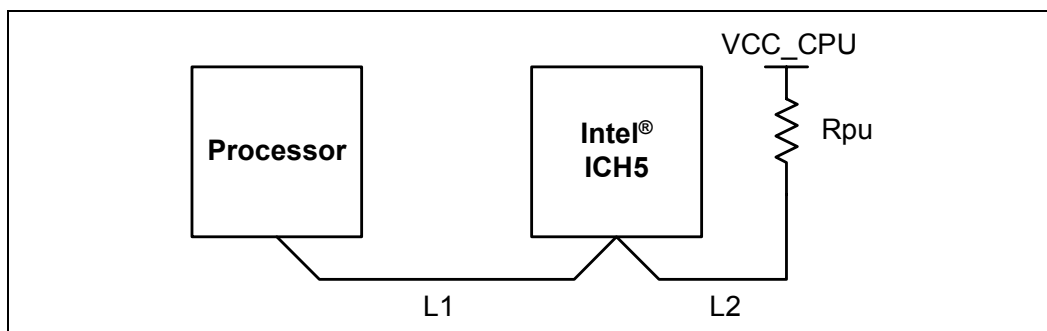
Figure 34. Routing Illustration for FERR# and THERMTRIP#
