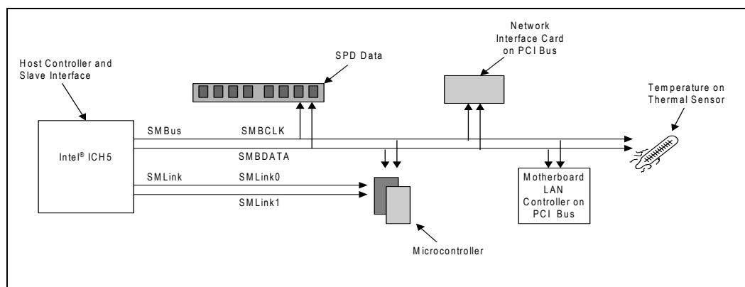
Figure 125. SMBUS 2.0/SMLink Interface
