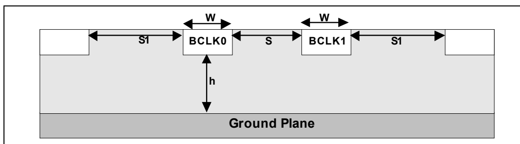
Figure 19. Trace Spacing for HOST_CLK Clocks
