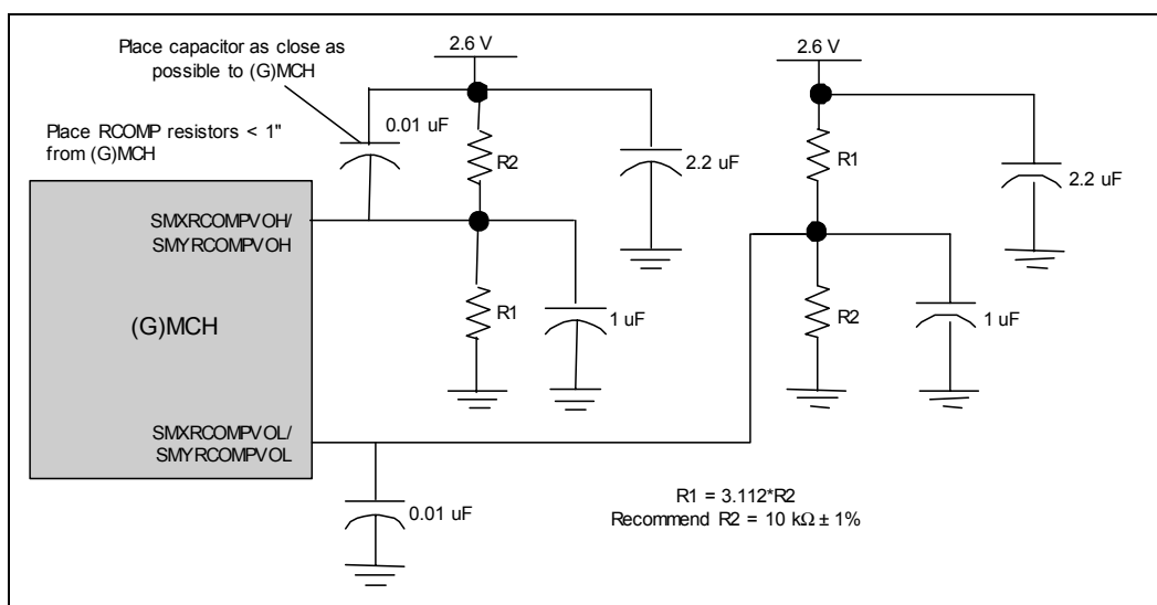
Figure 75. DDR RCOMP VOH and VOL Circuitry
