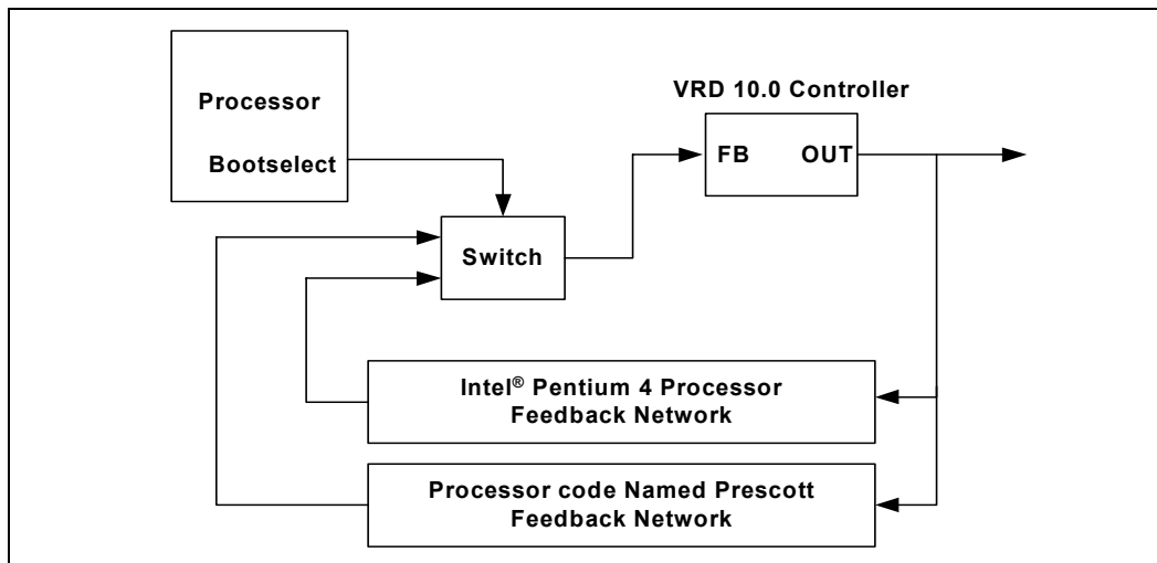
Figure 45. Routing Illustration for BOOTSELECT
