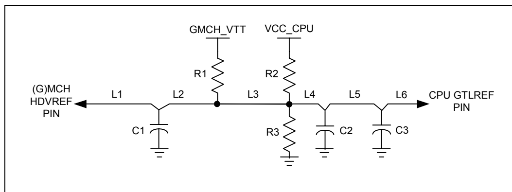
Figure 46. HD_VREF Circuit Topology
