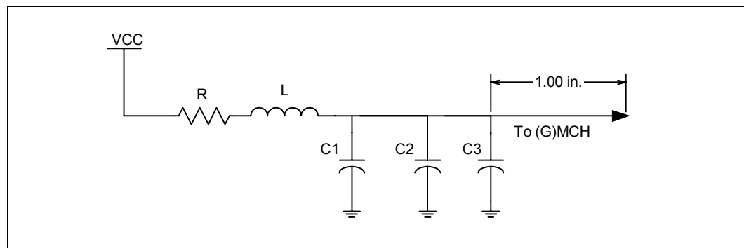
Figure 185. (G)MCH Analog Filter Topologies
