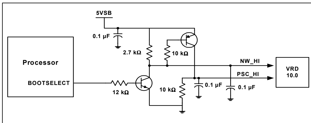
Figure 45. Routing Illustration for BOOTSELECT
