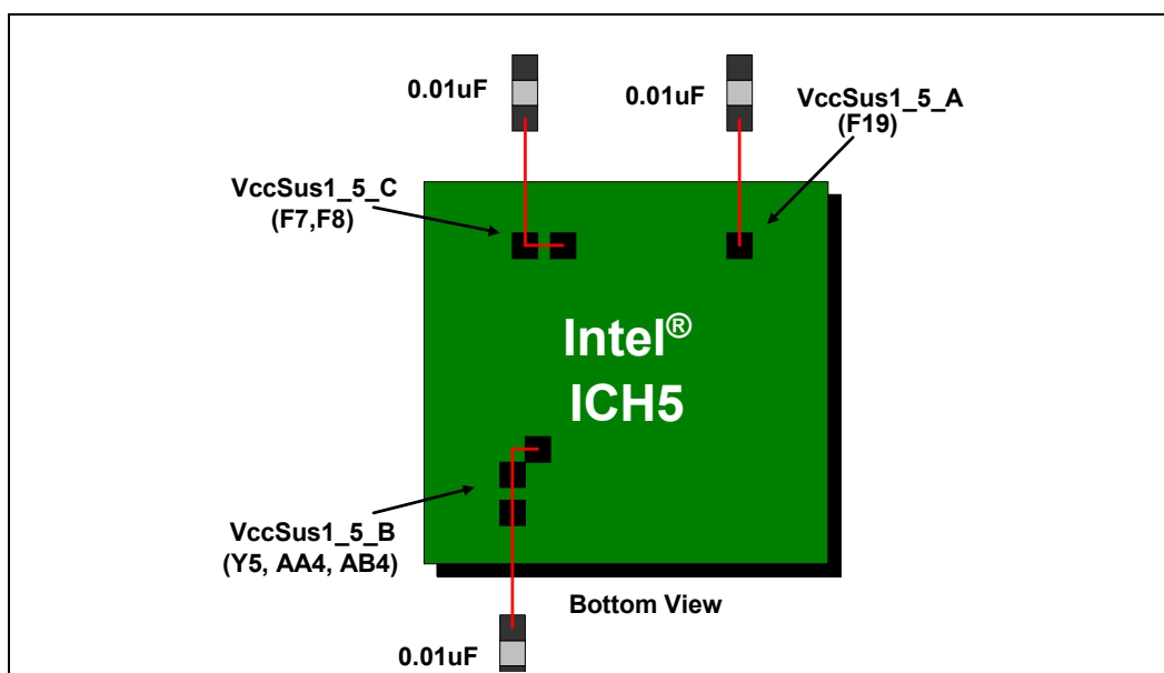
Figure 201. Intel® ICH5 Example Decoupling Capacitor Placement
