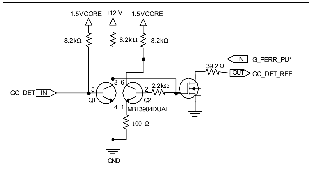
Figure 81. AGP Mode Detection Circuit (Option 1)
