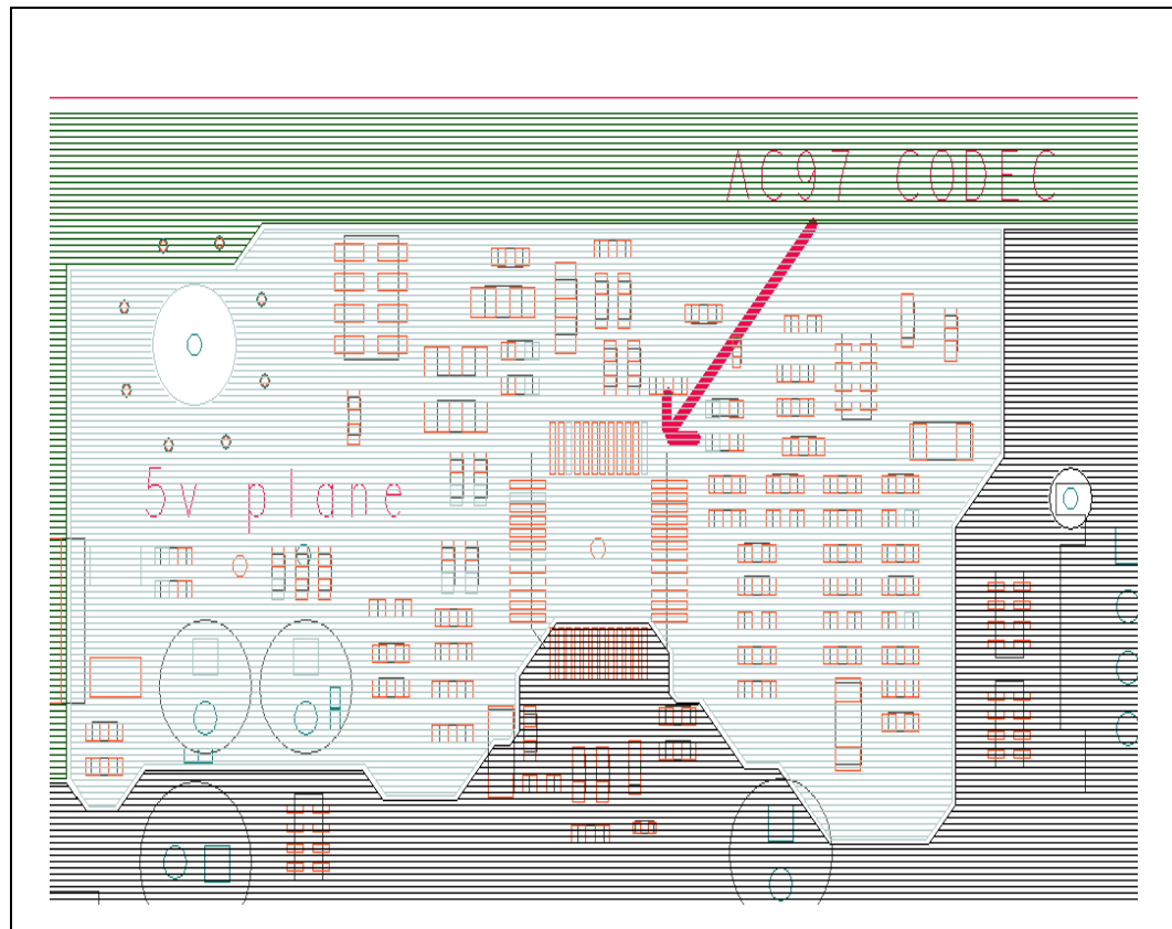
Figure 112. AC '97 Power Plane Configurations
