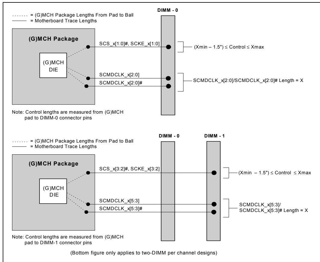
Figure 69. Control Signal Length Matching Requirements
