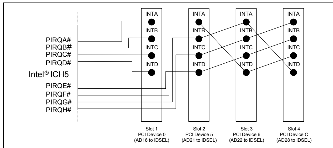
Figure 124. Example PIRQ Routing
