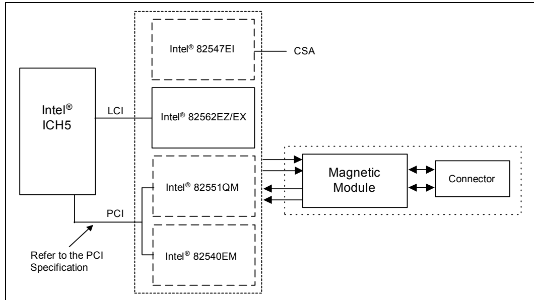
Figure 134. Intel® ICH5/Platform LAN Connect Sections
