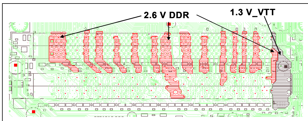
Figure 190. DDR DIMMS Layer 4 Power Delivery
