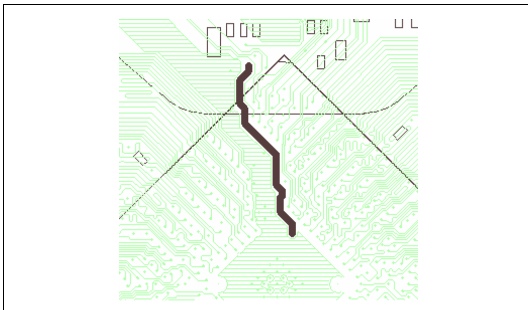
Figure 188. Layer 4 VCCA_DDR
