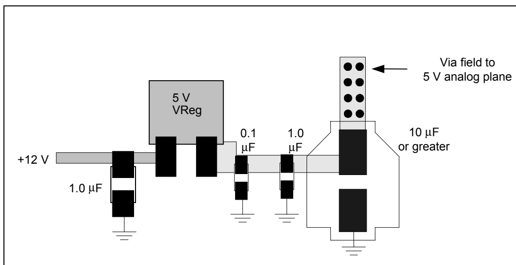
Figure 113. AC '97 Analog Power Delivery
