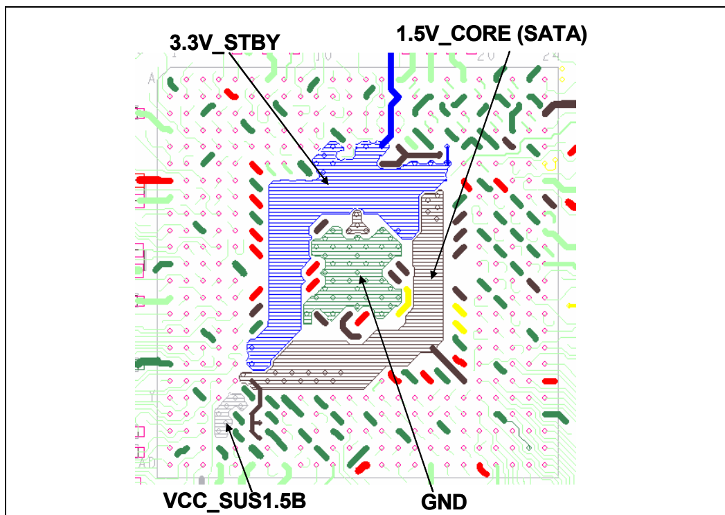
Figure 195. Intel® ICH5 Layer 2 Power Delivery
