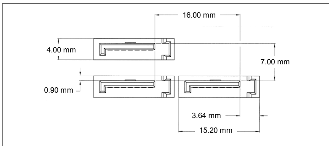
Figure 107. Minimum Host Connector Placement Spacing from SATA Specification
