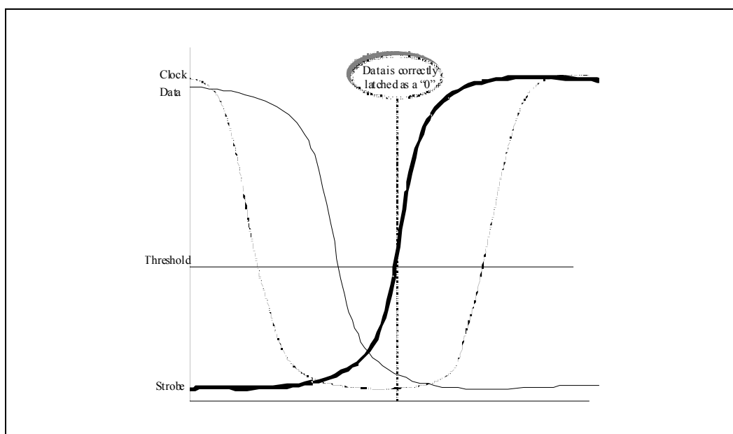
Figure 94. Effect of Crosstalk on Strobe Signal
