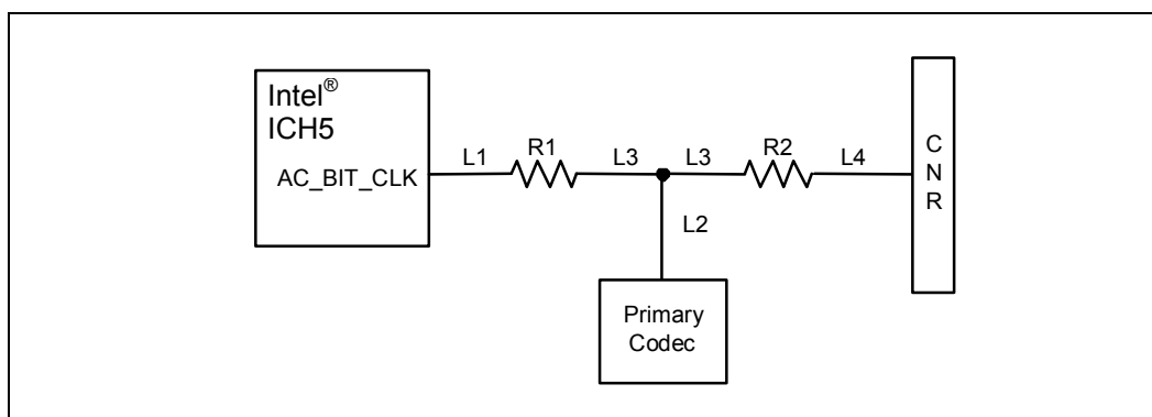
Figure 109. Intel® ICH5 AC '97 – AC_BIT_CLK Topology
