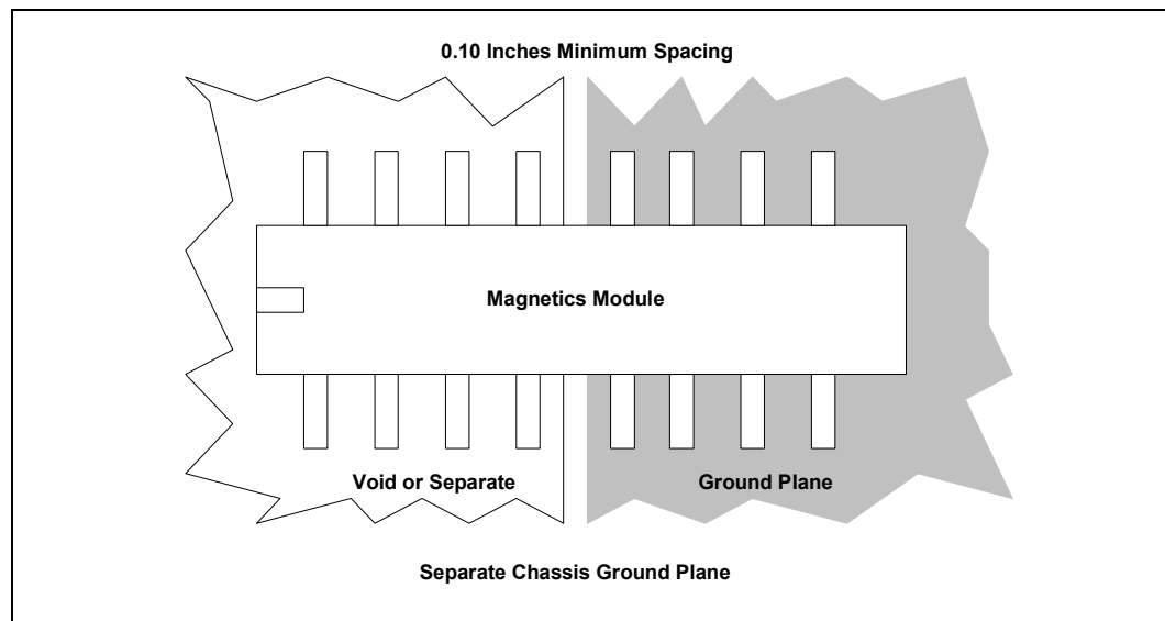
Figure 144. Ground Plane Separation
