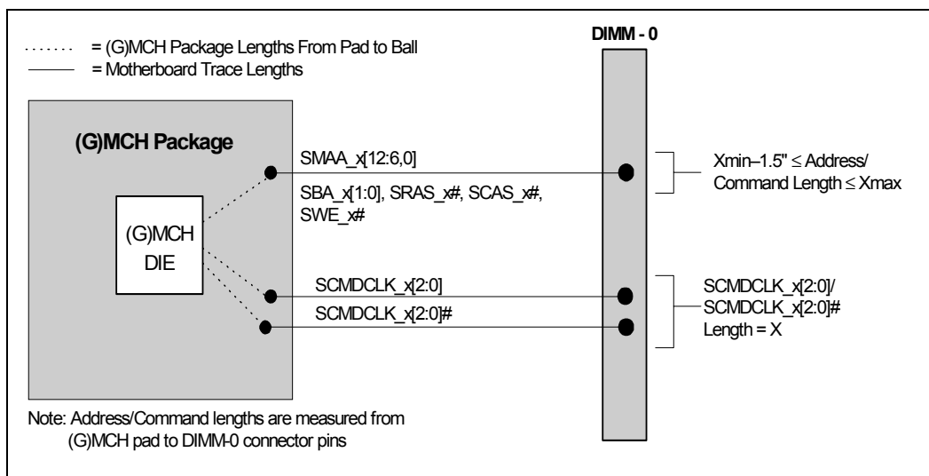
Figure 62. Address/Command to Clock Length Matching Requirements
