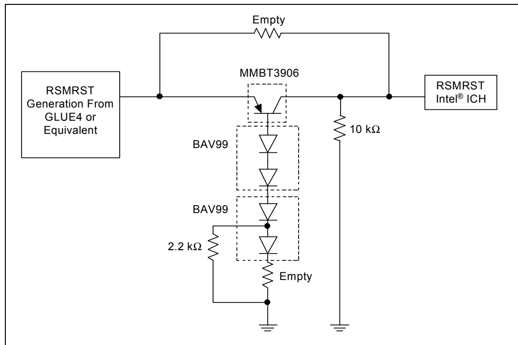
Figure 147. RTC Power Well Isolation Control
