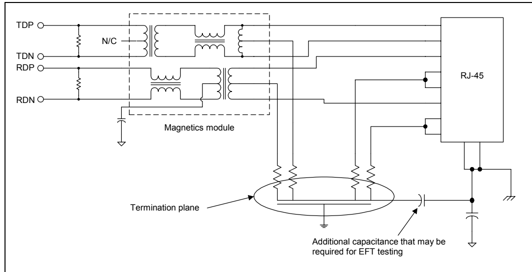
Figure 141. Termination Plane
