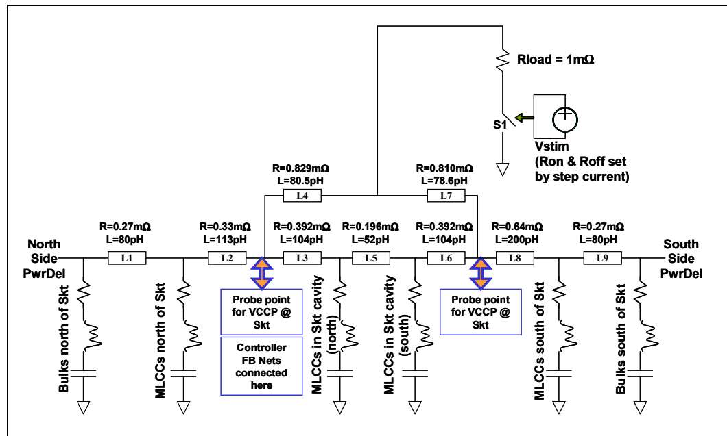
Figure 168. Detailed Power Distribution Model for Processor with Voltage Regulator on System Board
