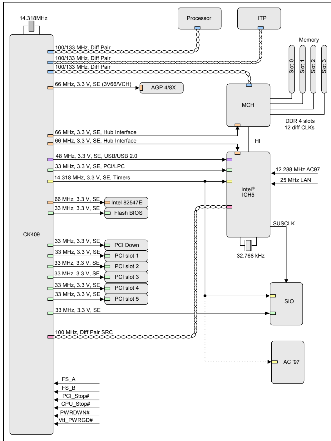
Figure 16. Intel® 865P Chipset-Based System Clocking Diagram
