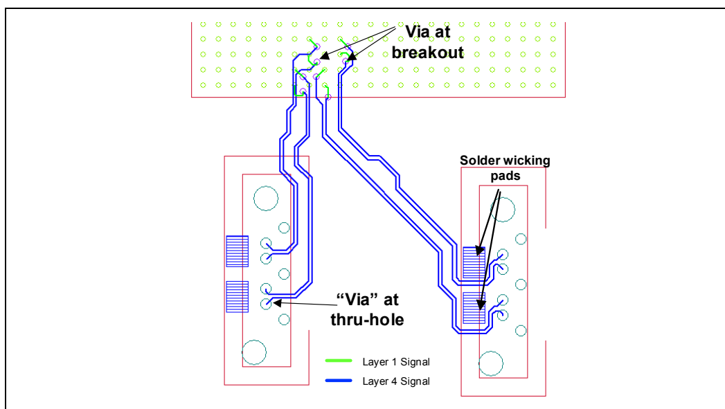
Figure 99. SATA Layout and Routing Example
