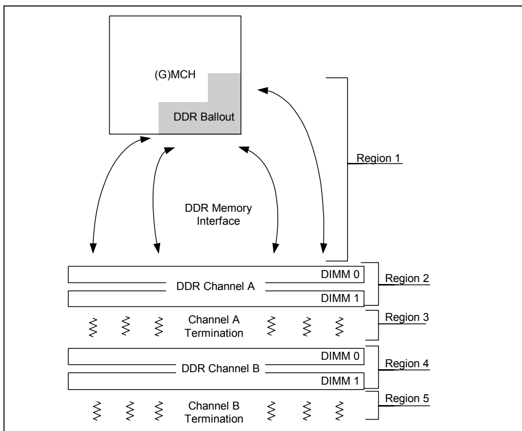
Figure 55. Two DIMM per-Channel DDR Regions for Trace Width and Spacing
