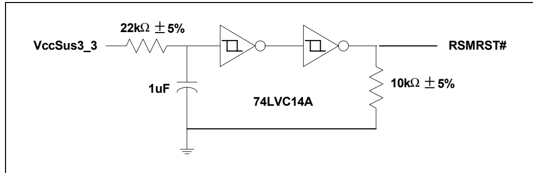
Figure 148. RSMRST# Generation from VCCSUS3_3
