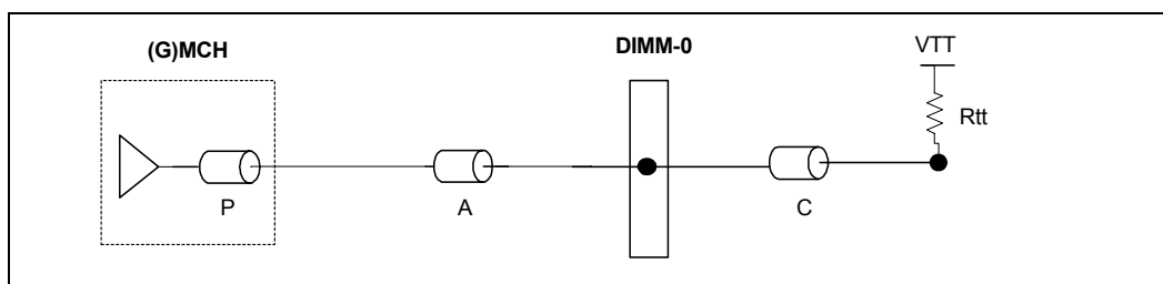
Figure 62. Address/Command to Clock Length Matching Requirements
