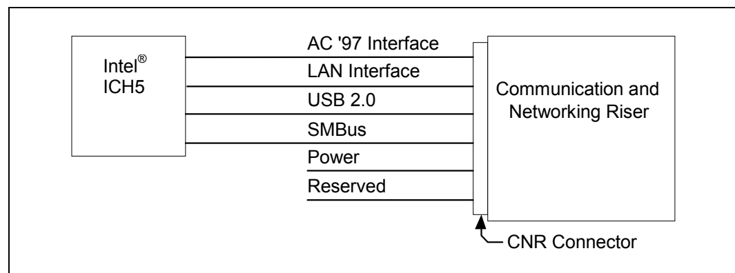
Figure 115. CNR Interface
