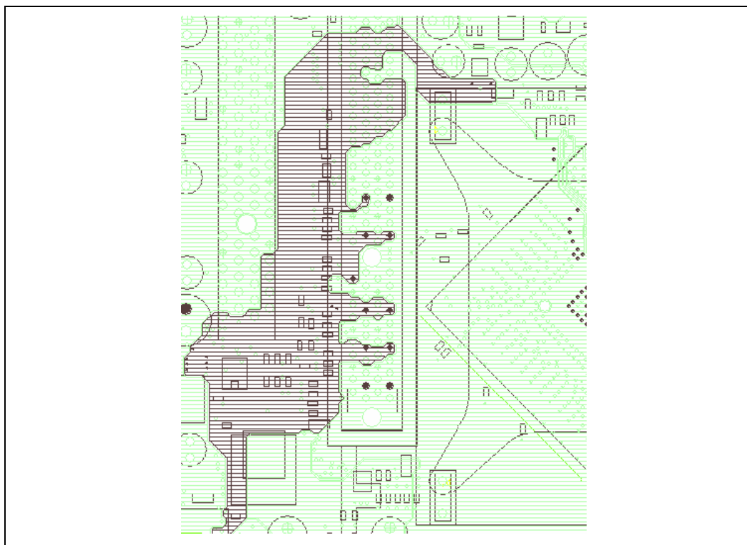
Figure 180. 1.5 V Power Plane (Layer 2)
