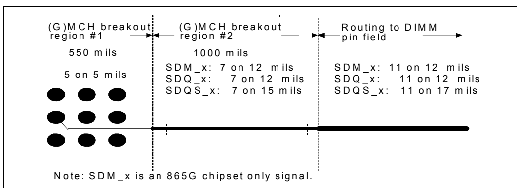
Figure 63. Data Signal Breakout Topology for Byte Lane Lengths > 5.7 Inches
