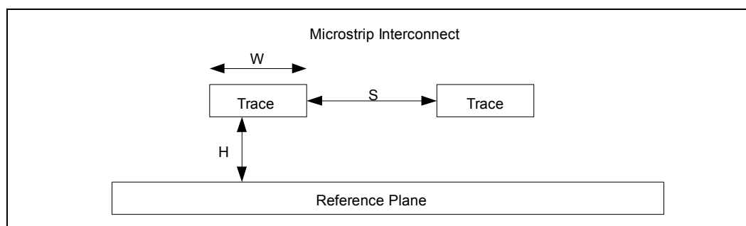
Figure 80. Spacing to Dielectric Height Diagram
