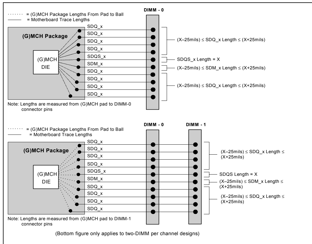
Figure 67. Data Signal and Data Mask Length Matching Requirements to Data Strobe
