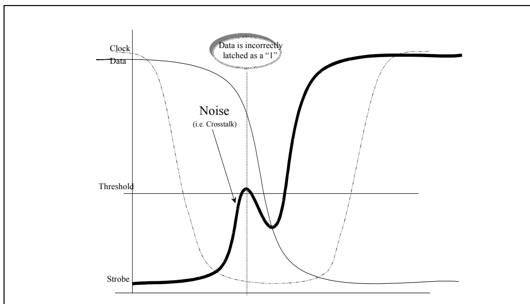
Figure 94. Effect of Crosstalk on Strobe Signal
