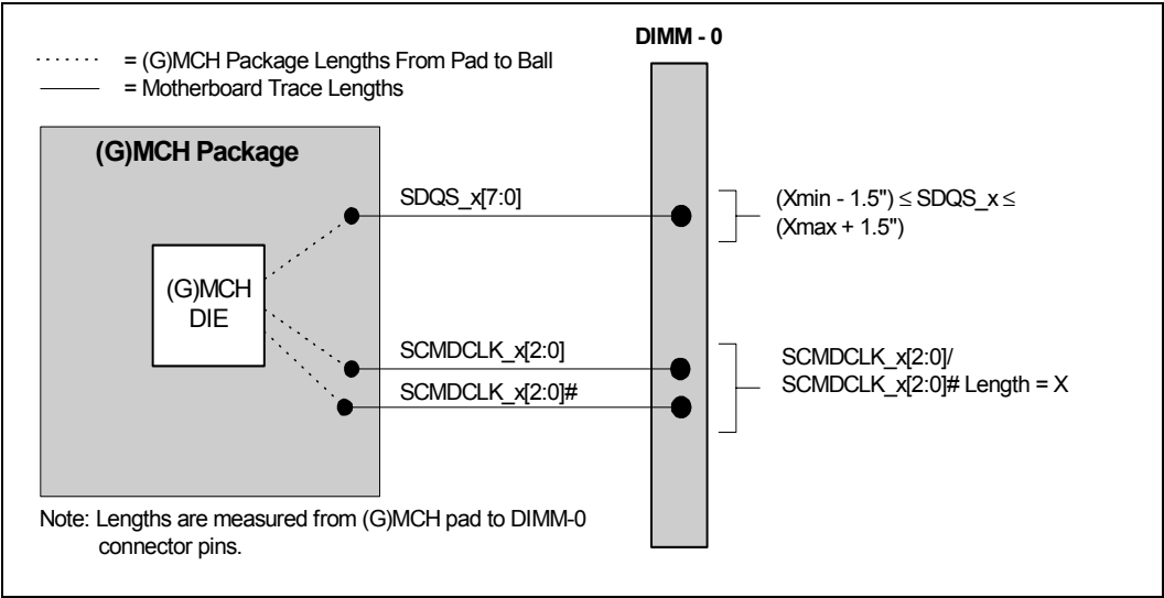
Figure 66. Data Strobe Length Matching Requirements to DDR Clock
