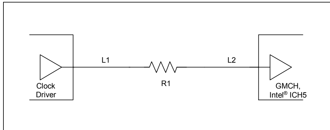
Figure 28. Topology for DOTCLK (Intel® 865G Chipset Only)
