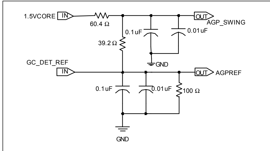
Figure 83. GVREF/GSWING Circuit
