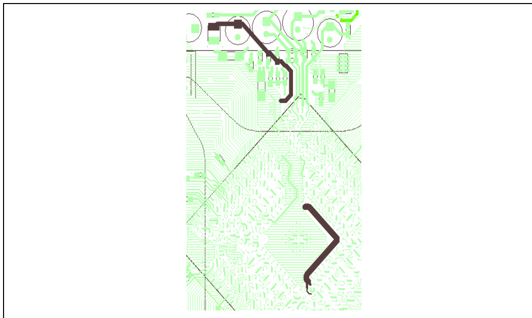
Figure 188. Layer 4 VCCA_DDR
