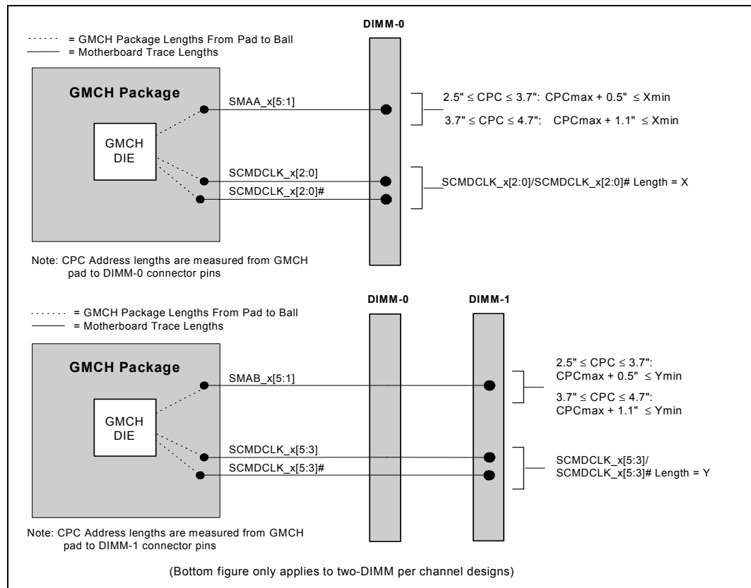
Figure 71. CPC Address Length Matching Requirements
