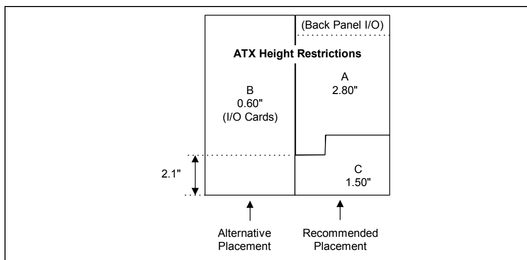
Figure 104. SATA Host Connector Placement Region Recommendations
