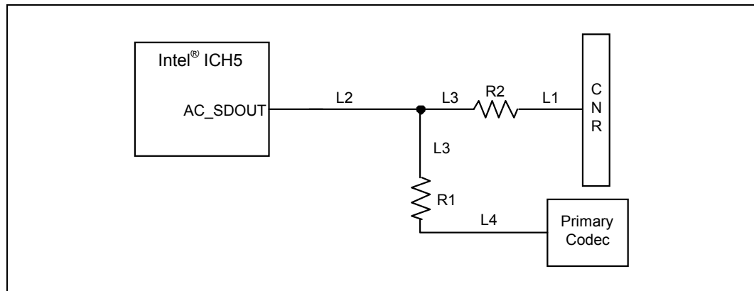
Figure 110. Intel® ICH5 AC '97 – AC_SDOOUT/AC_SYNC Topology
