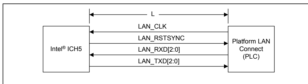
Figure 135. Single Solution Interconnect
