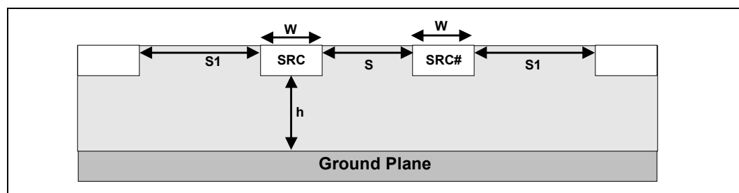
Figure 30. Trace Spacing for SRC Clocks
