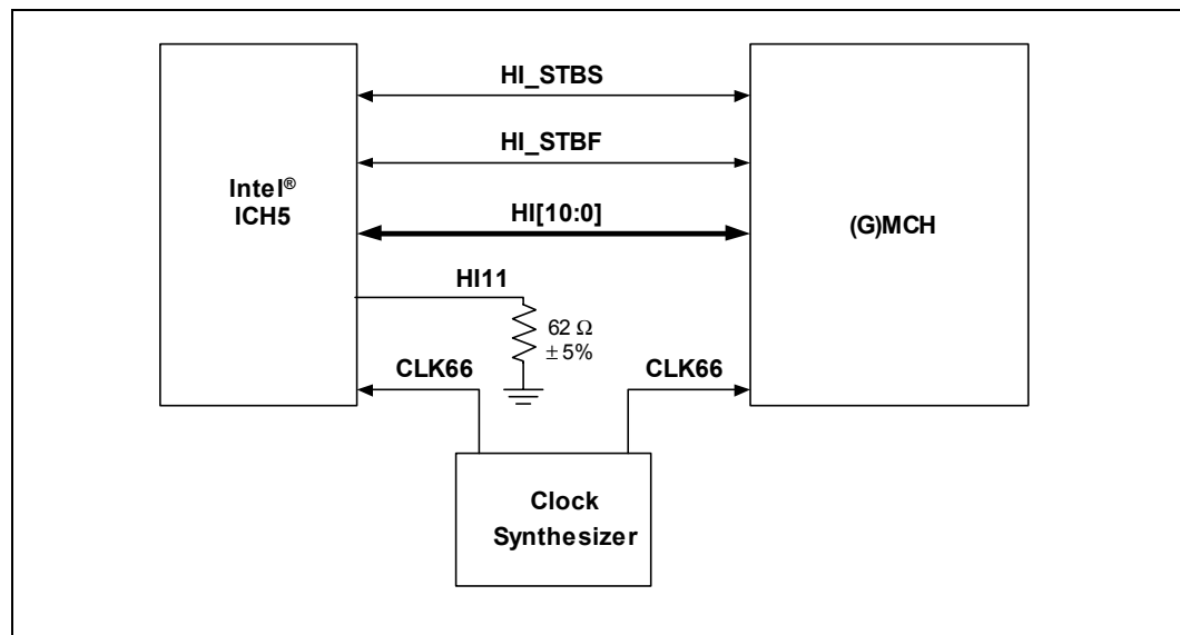
Figure 76. Hub Interface Routing Example
