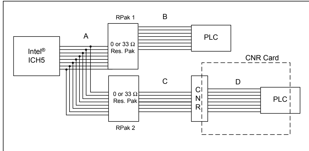
Figure 136. LOM/CNR Interconnect
