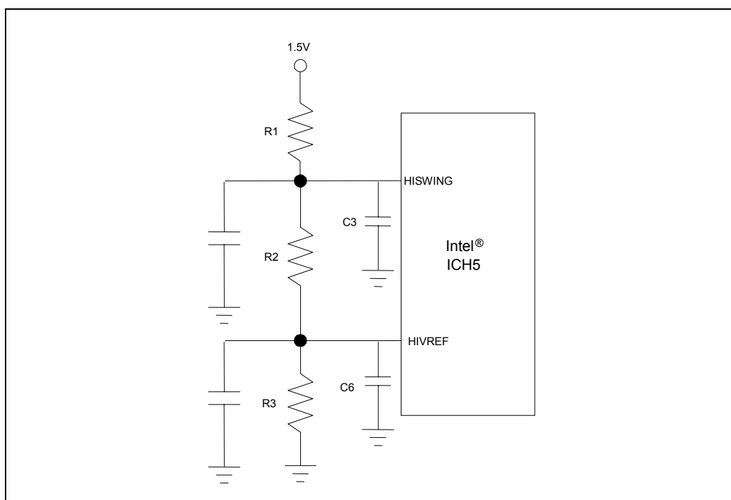
Figure 79. Hub Interface Local HIVREF/HISWING Generation Circuit (Intel® ICH5 Side)
