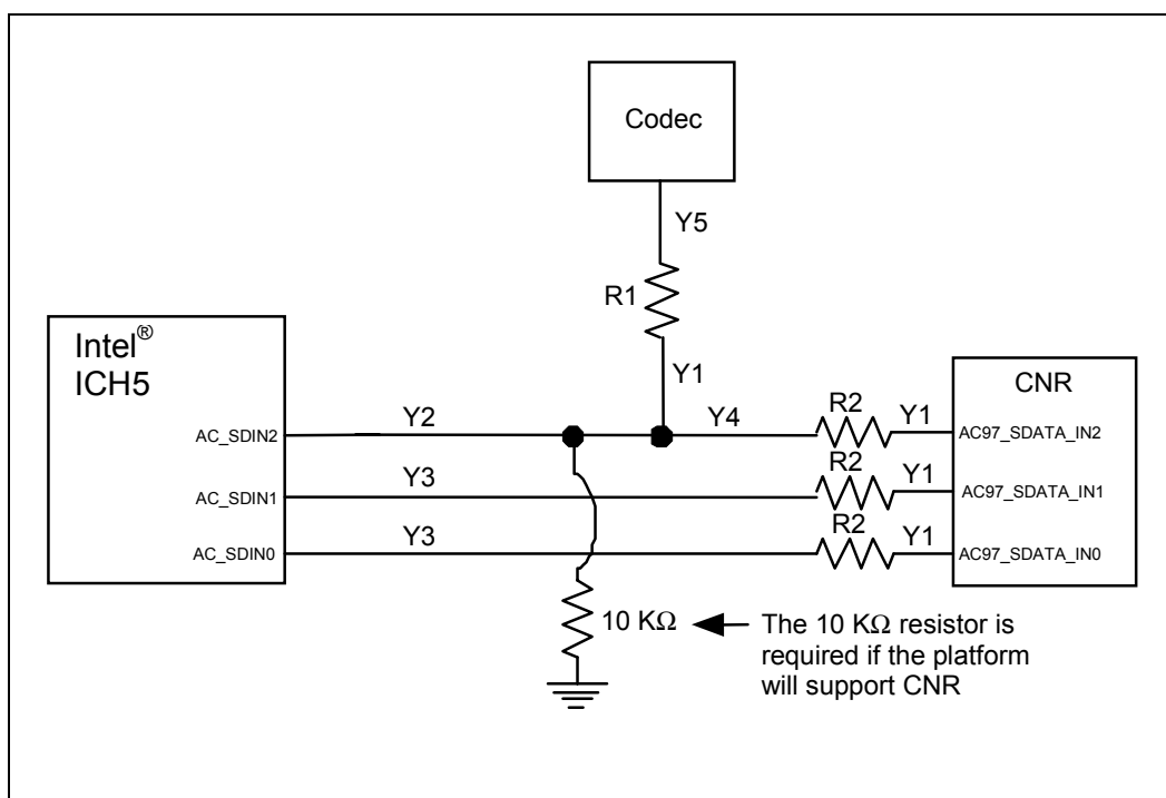
Figure 111. Intel® ICH5 AC '97 – AC_SDIN Topology
