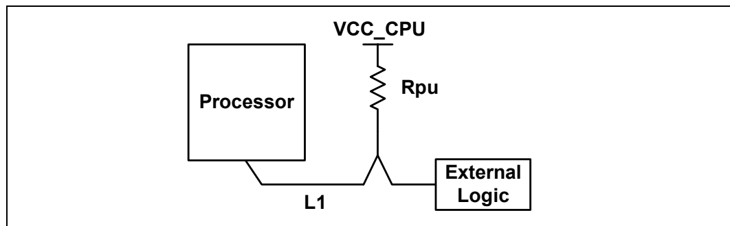
Figure 36. Routing Illustration for IERR
