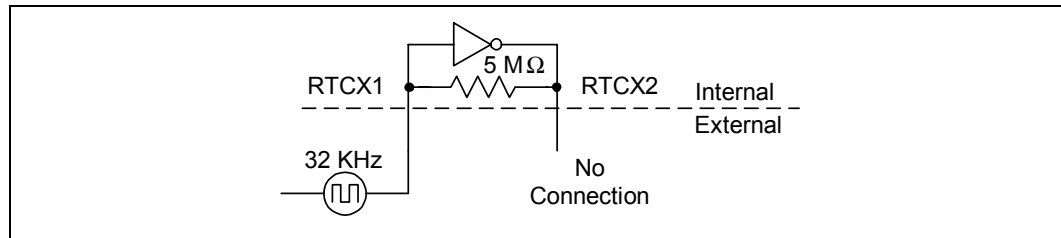
Figure 130. External Circuitry for the Intel® ICH5 Where the Internal RTC Is Not Used
