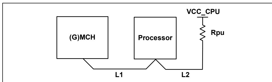
Figure 37. Routing Illustration for RESET# and BR0#
