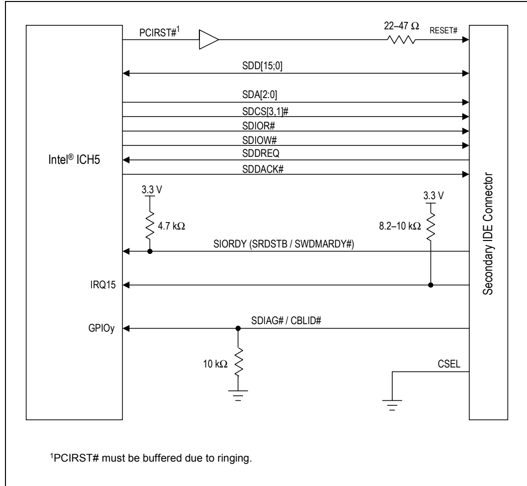
Figure 98. Connection Requirements for Secondary IDE Connector
