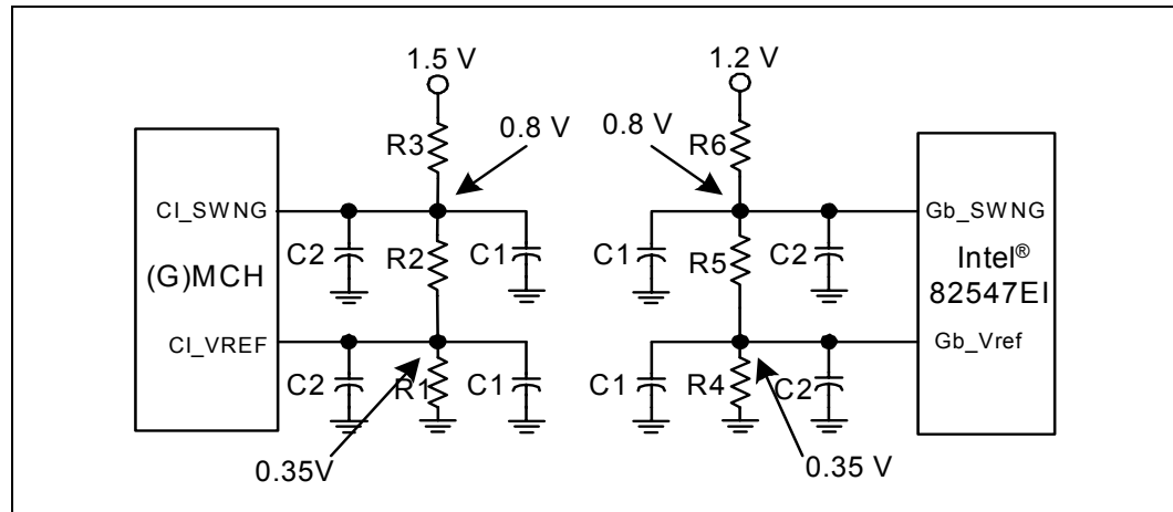
Figure 90. CSA Port Locally Generated Reference Divider Circuits
