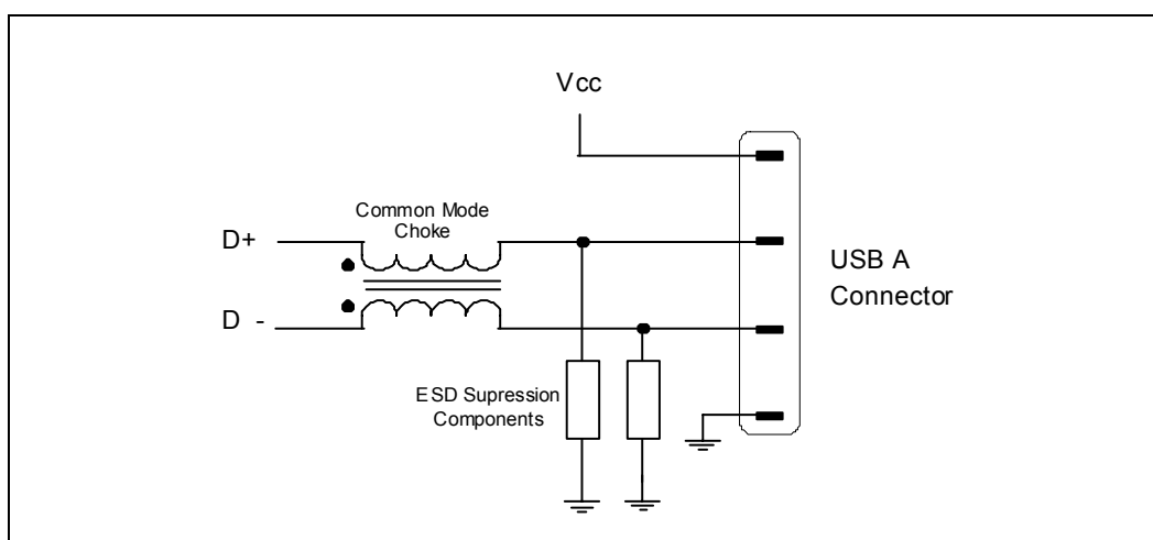
Figure 121. A Common-Mode Choke
