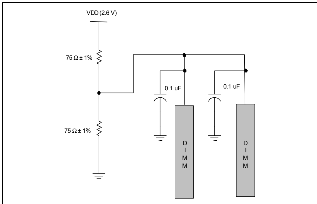
Figure 73. DDR VREF Generation Example Circuit at the DIMMs
