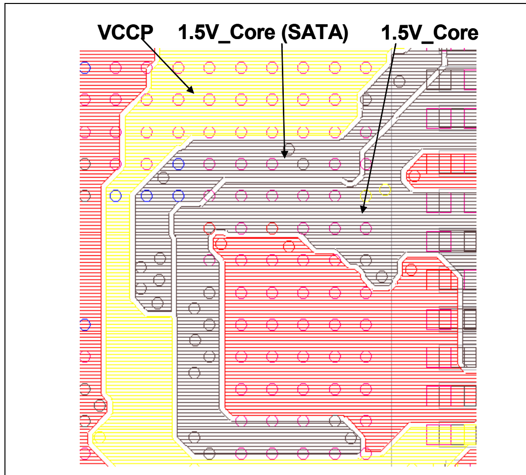
Figure 196. Layer 2 Close Up
