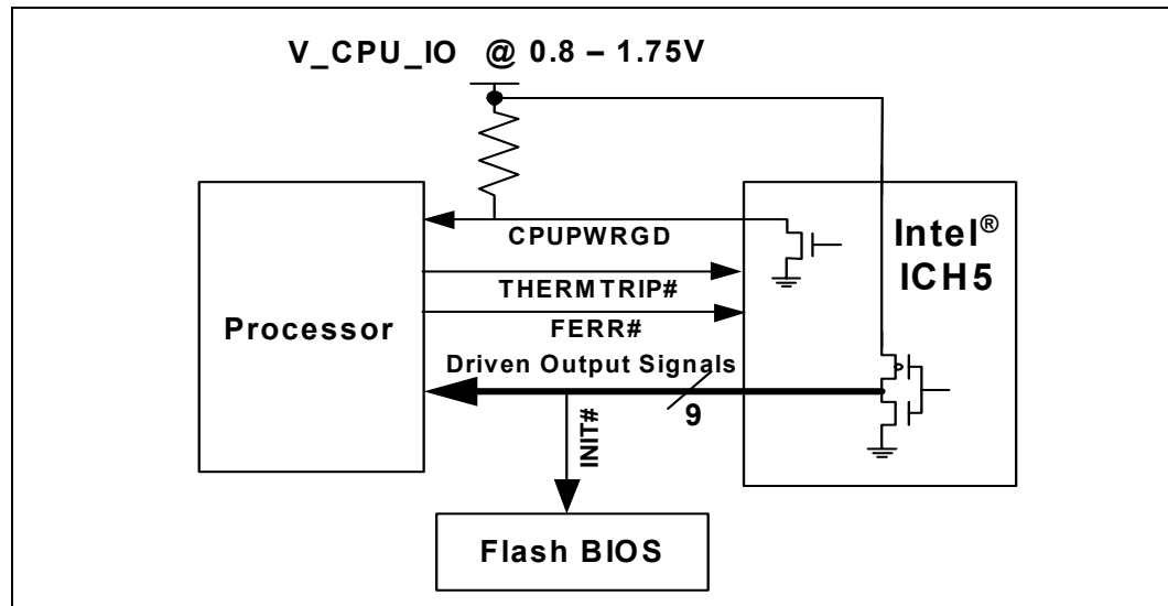
Figure 152. Intel® ICH5 Processor CMOS Signals with Processor and Flash BIOS
