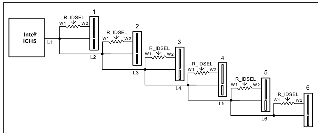
Figure 128. PCI Bus Layout Example with IDSEL
