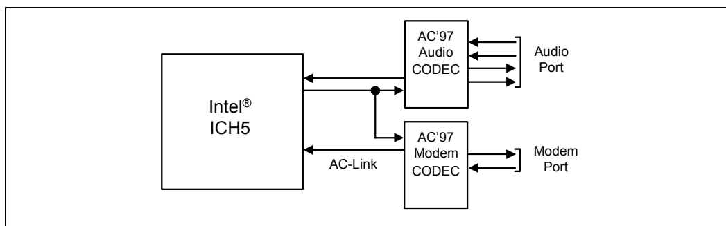
Figure 6. AC '97 with Audio and Modem Codec
