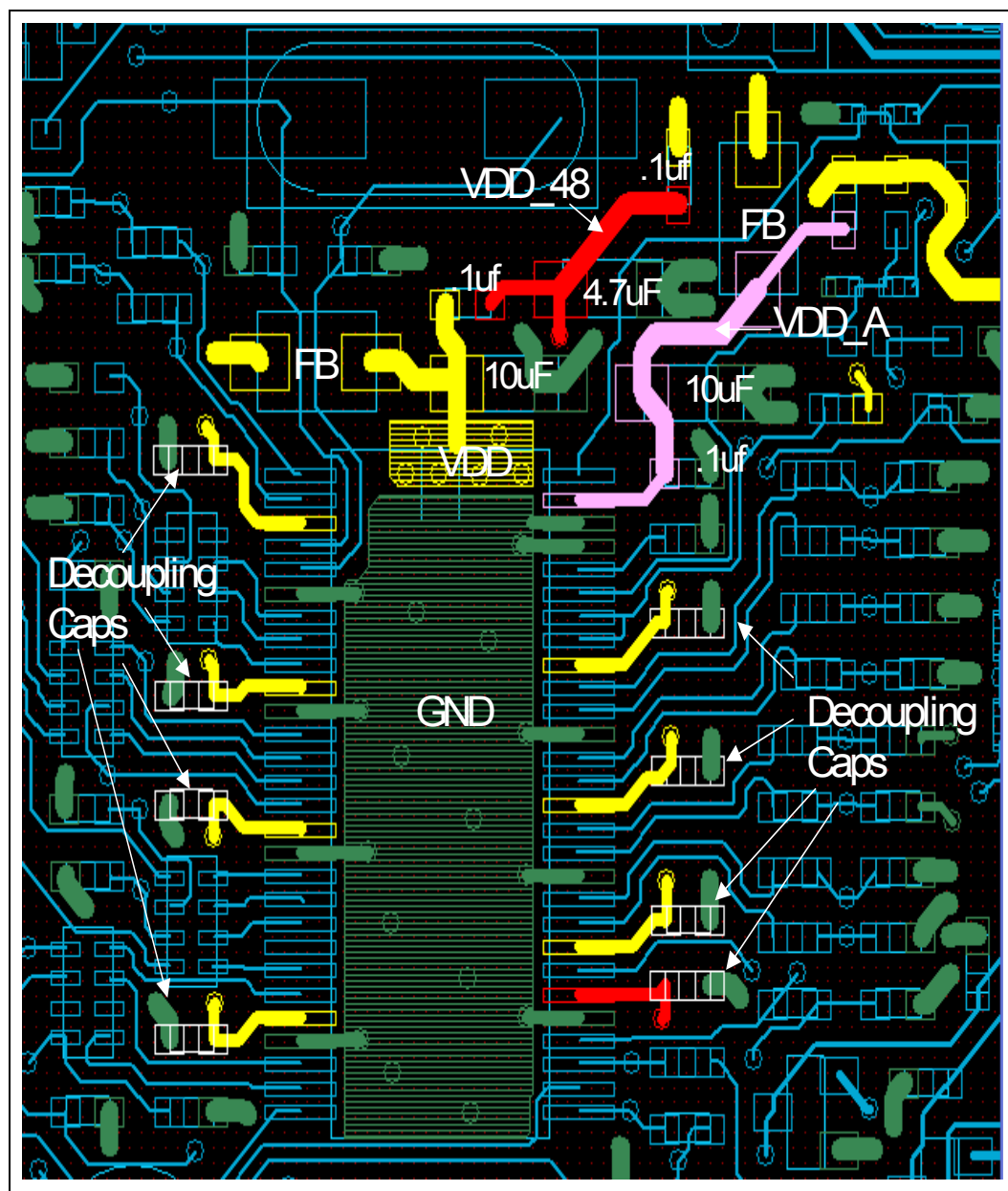
Figure 31. Decoupling Capacitors Placement and Connectivity
