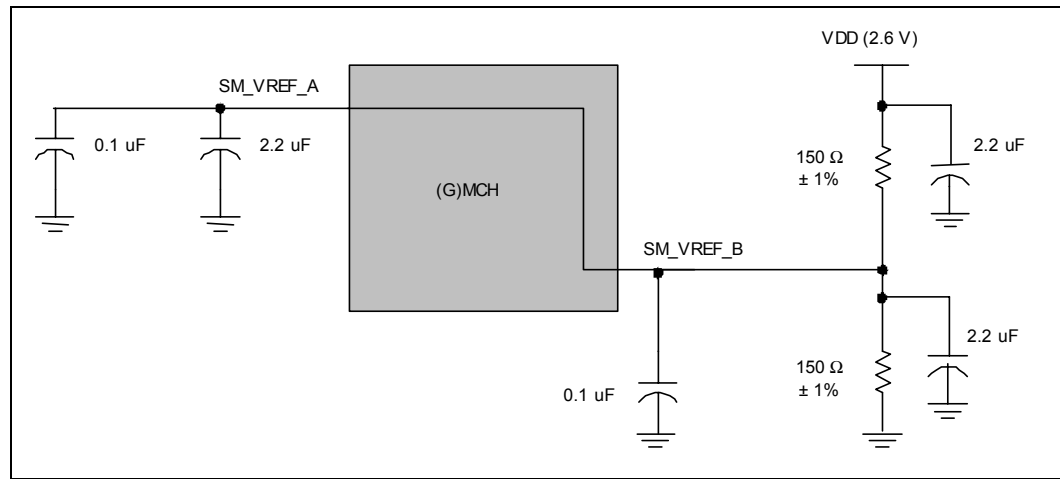
Figure 72. DDR VREF Generation Example Circuit at the (G)MCH
