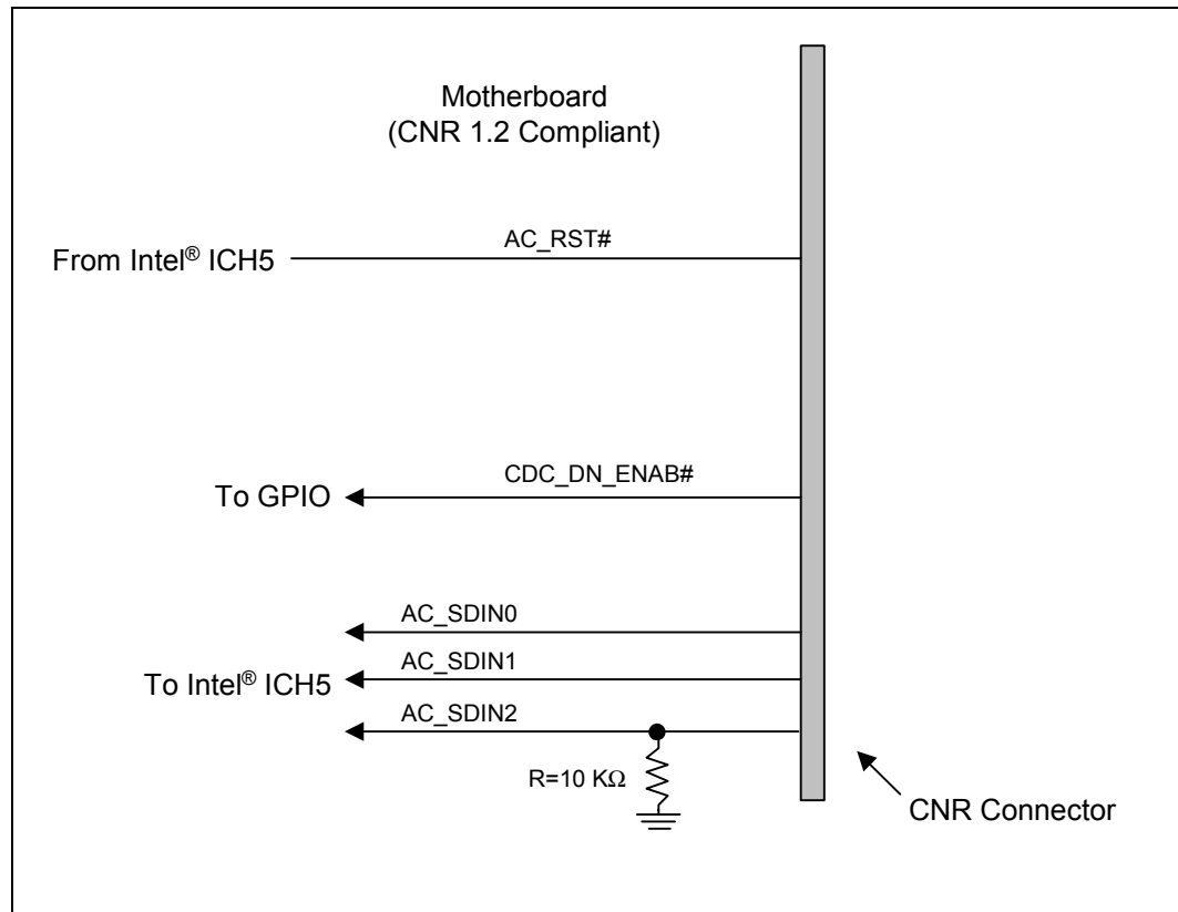
Figure 117. Motherboard AC '97 CNR Implementation with No Codec down on Board
