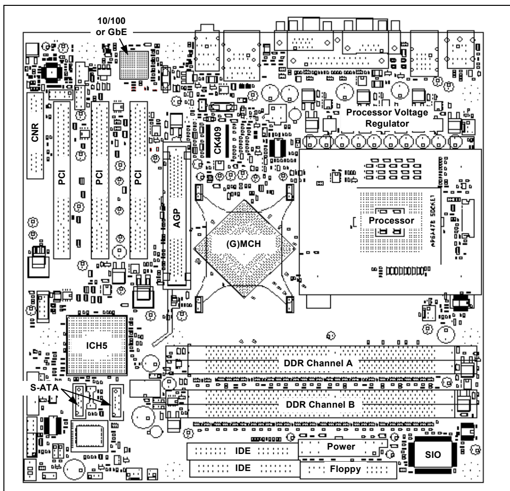
Figure 14. Component Placement Example Using a 4-DIMM \mu ATX Board
