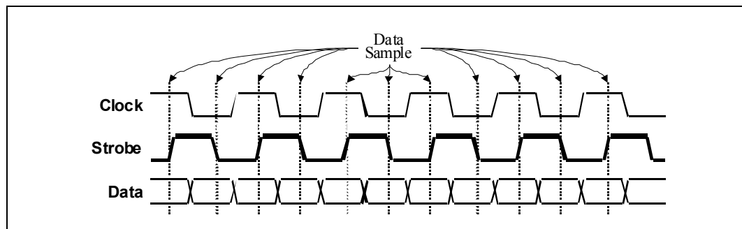
Figure 92. Data Strobing Example
