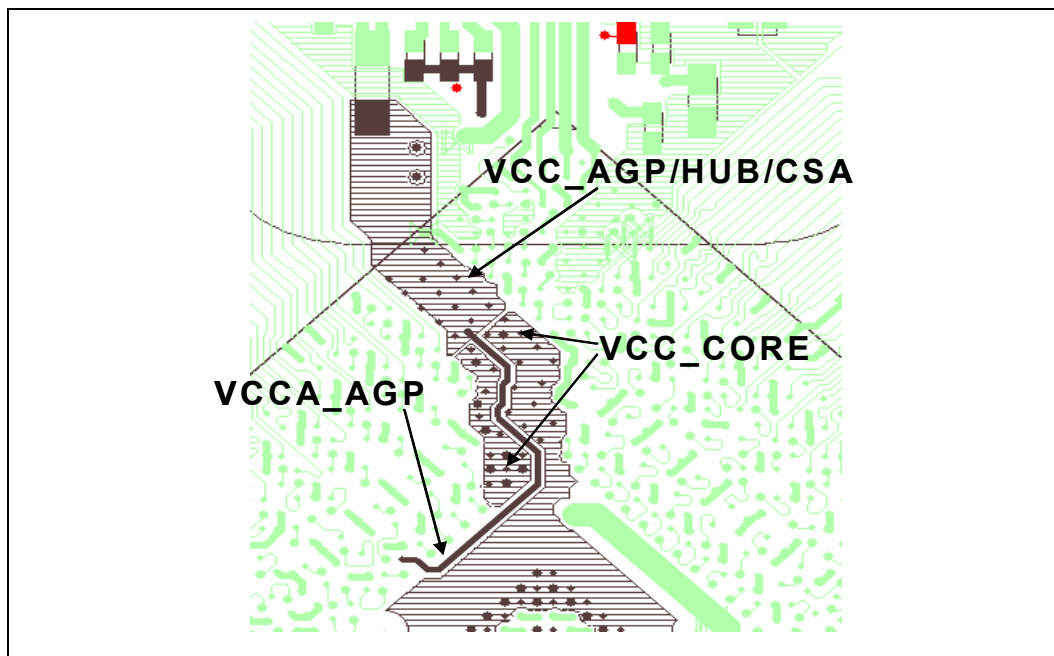
Figure 179. 1.5 V Power Plane (Layer 1)
