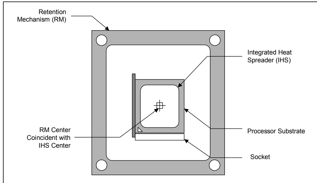
Figure 53. Processor Location Recommendation Relative to Retention Mechanism
