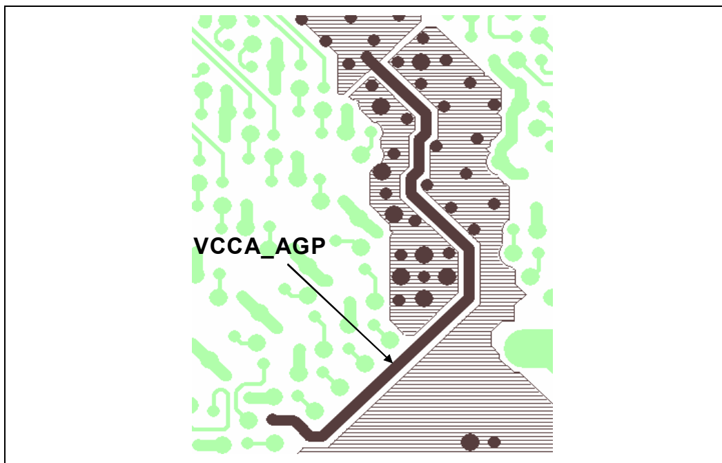
Figure 186. VCCA_AGP Routing
