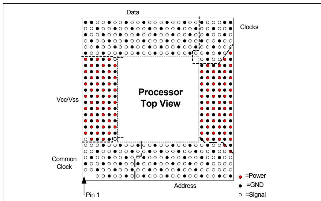
Figure 11. Processor Component Quadrant Layout (Top View)
