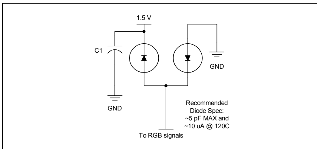
Figure 88. RGB Protection Diodes
