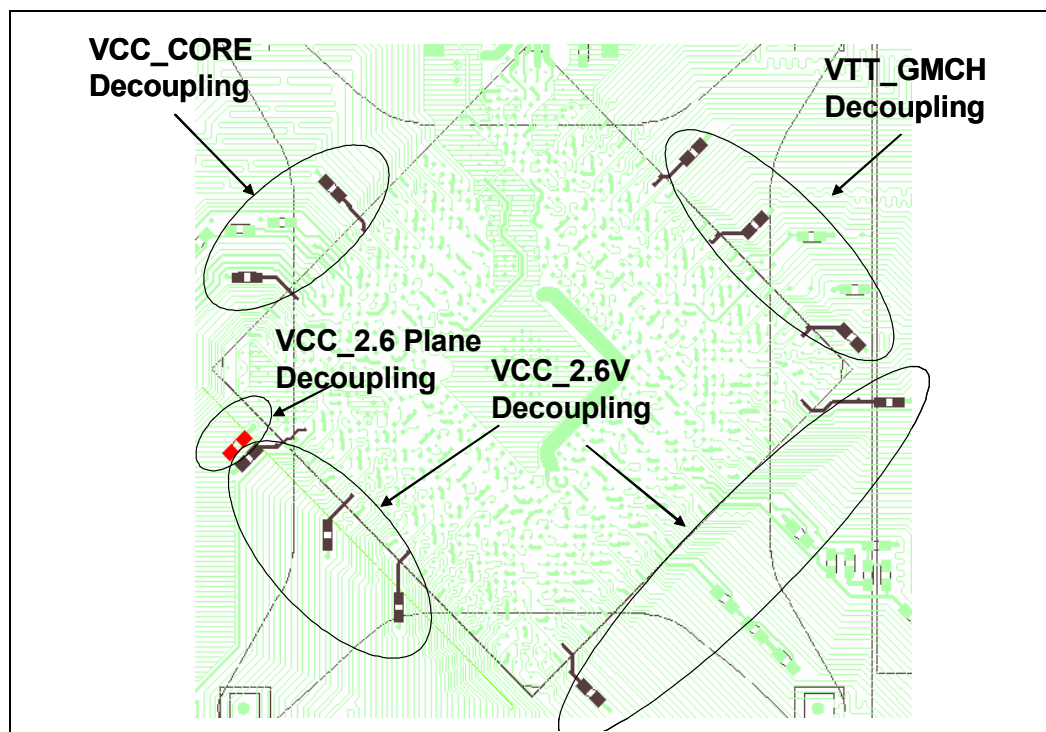
Figure 182. (G)MCH High-Frequency Decoupling Capacitor Placement
