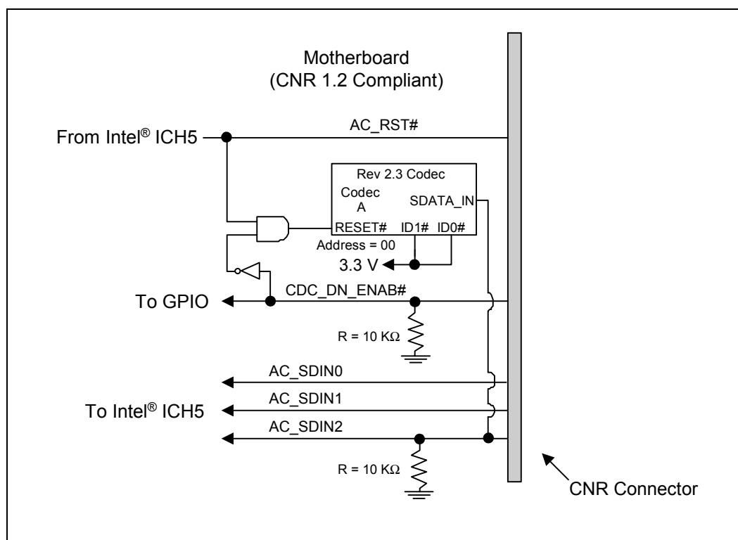
Figure 116. Motherboard AC '97 CNR Implementation with a Single Codec down on Board
