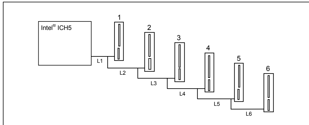
Figure 127. PCI Bus Layout Example
