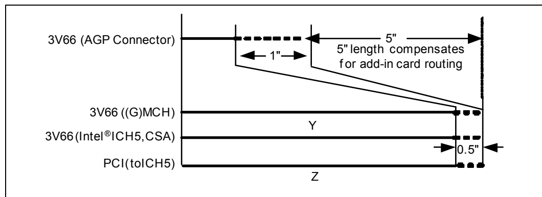
Figure 20. 66 MHz/33 MHz Clock Relationships
