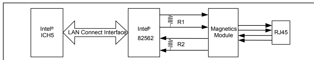
Figure 138. Intel® 82562EZ/ET/EX/EM PLC Components/ Intel® 82551QM PLC Components Termination
