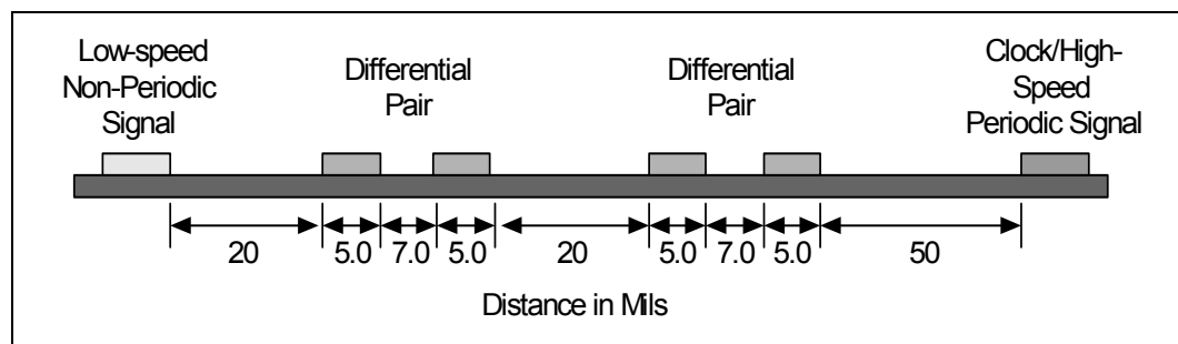
Figure 100. Recommended Serial ATA Trace Spacing
