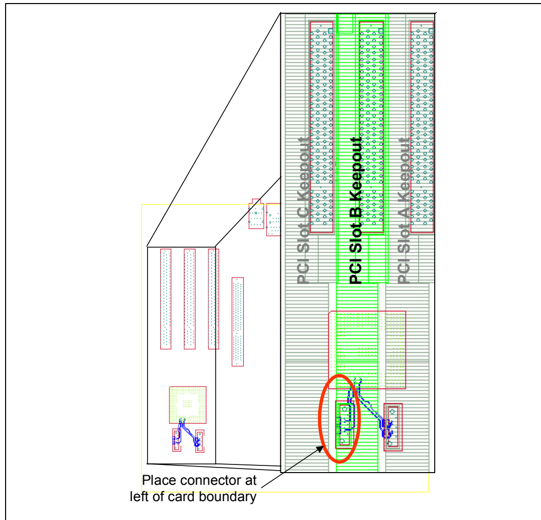
Figure 105. SATA Host Connector Placement ATX Area B Example
