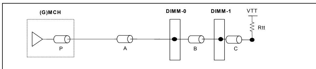
Figure 61. One DIMM per-Channel Address/Command Length Matching Topology
