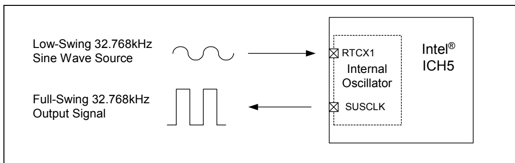
Figure 129. RTCX1 and SUSCLK Relationship in Intel® ICH5
