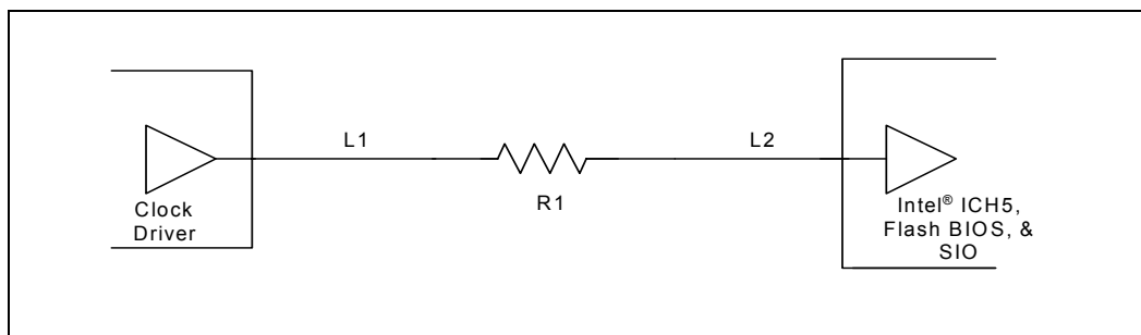
Figure 25. Topology for CLK33 to PCI Slot
