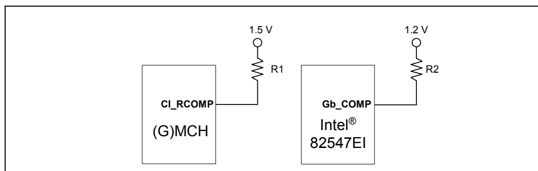
Figure 91. CSA Port RCOMP Circuits
