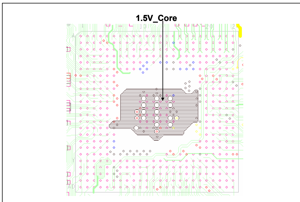
Figure 198. Intel® ICH5 Layer 4 Power Delivery
