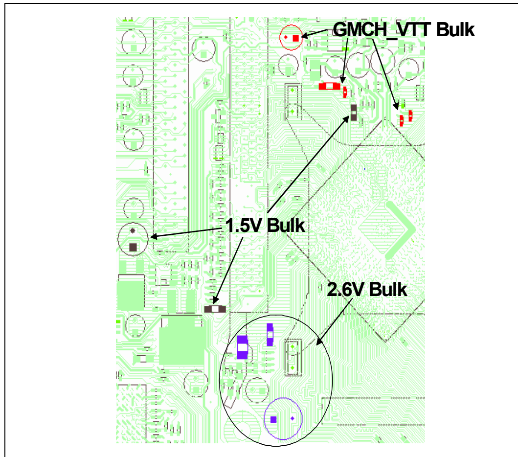
Figure 183. (G)MCH Bulk Decoupling Capacitor Placement
