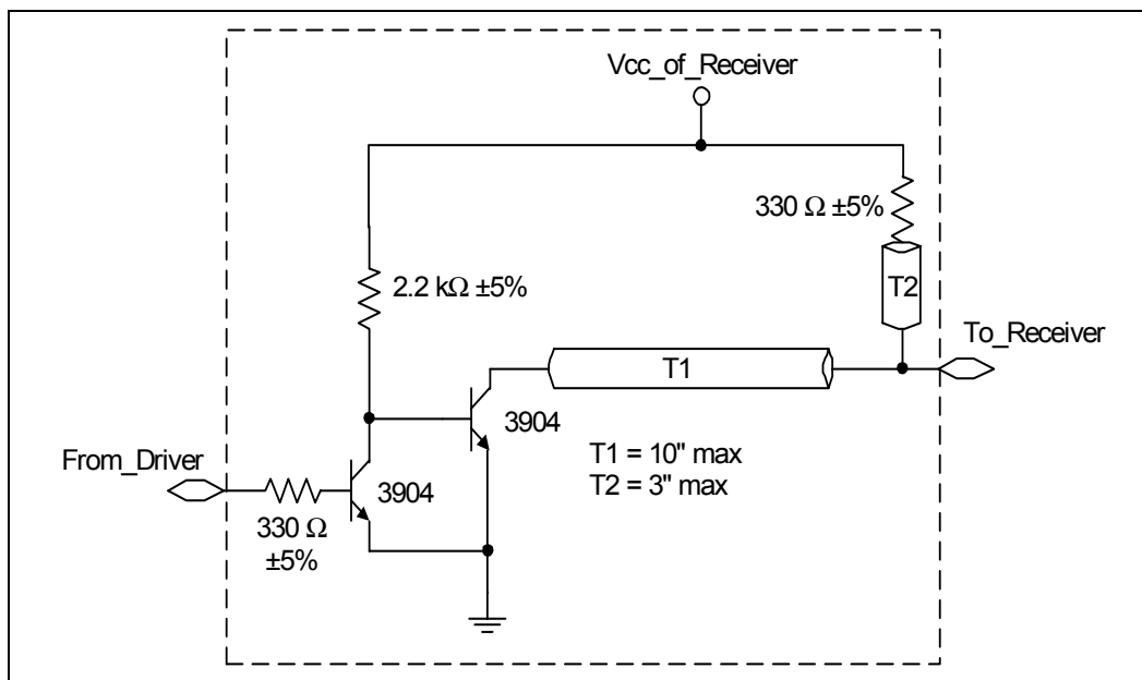
Figure 154. Flash BIOS Level Translation Circuitry
