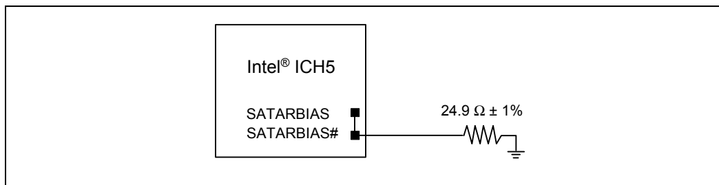
Figure 101. SATARBIAS/SATARBIAS# Connection
