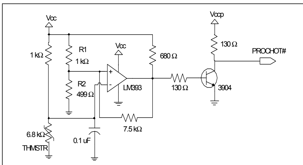
Figure 167. Example VR Thermal Monitor Circuit
