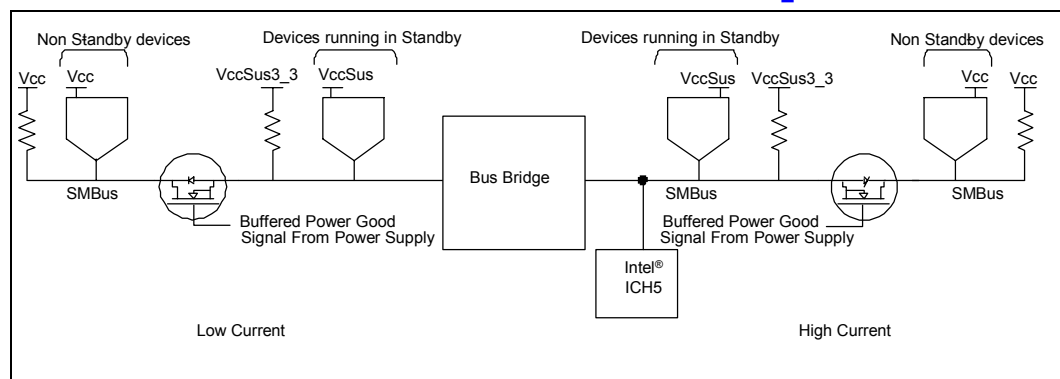
Figure 126. High Power/Low Power Mixed VCC_SUSPEND/ VCC_CORE Architecture
