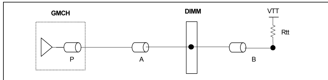
Figure 71. CPC Address Length Matching Requirements
