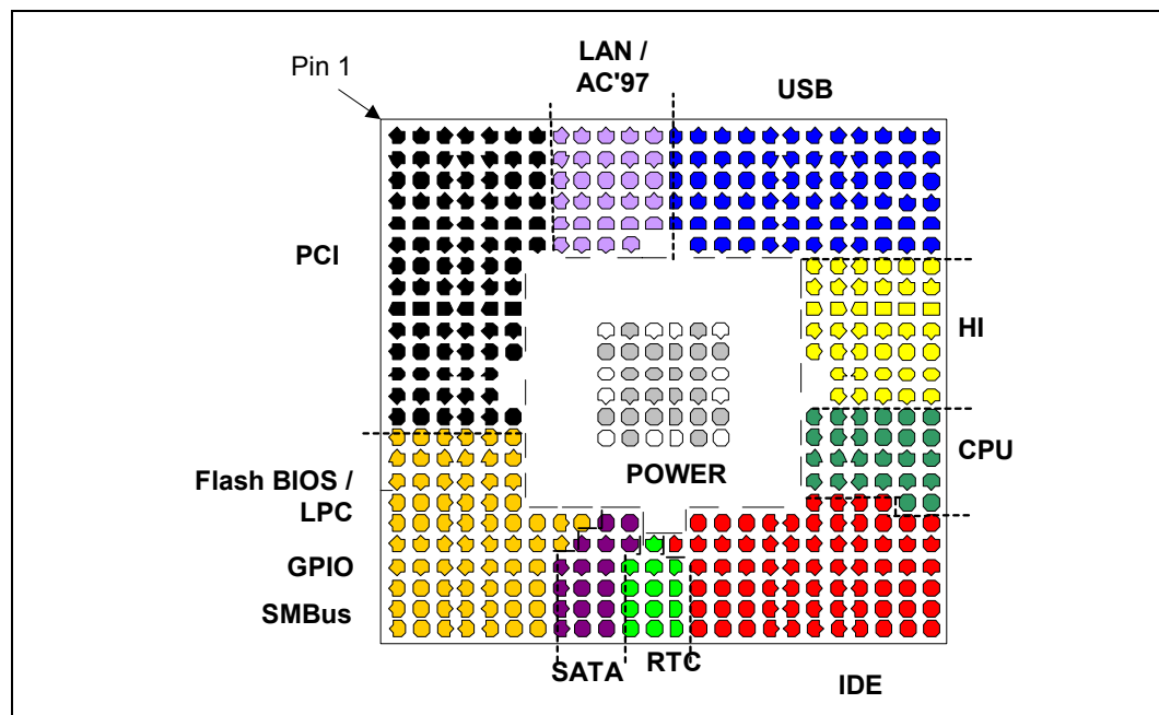
Figure 13. Intel® ICH5 Quadrant Layout (Top View)
