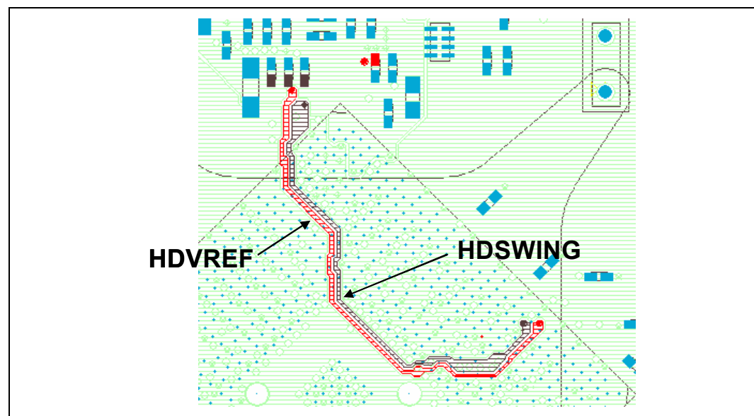
Figure 48. Host SWING Routing Example
