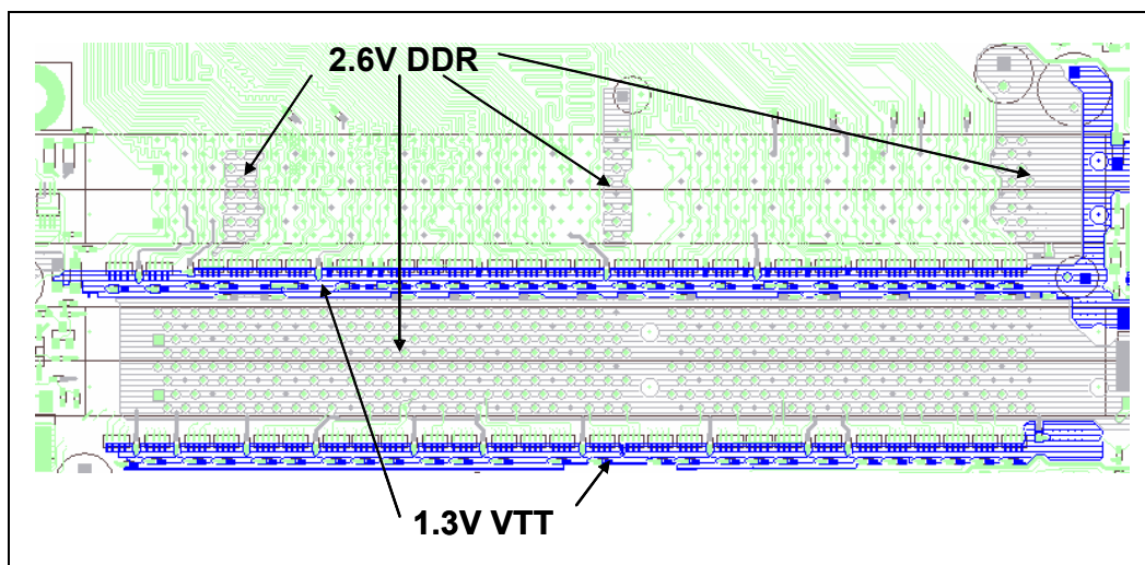
Figure 190. DDR DIMMS Layer 4 Power Delivery
