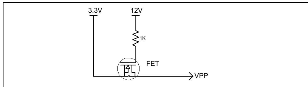
Figure 155. Flash BIOS VPP Circuitry
