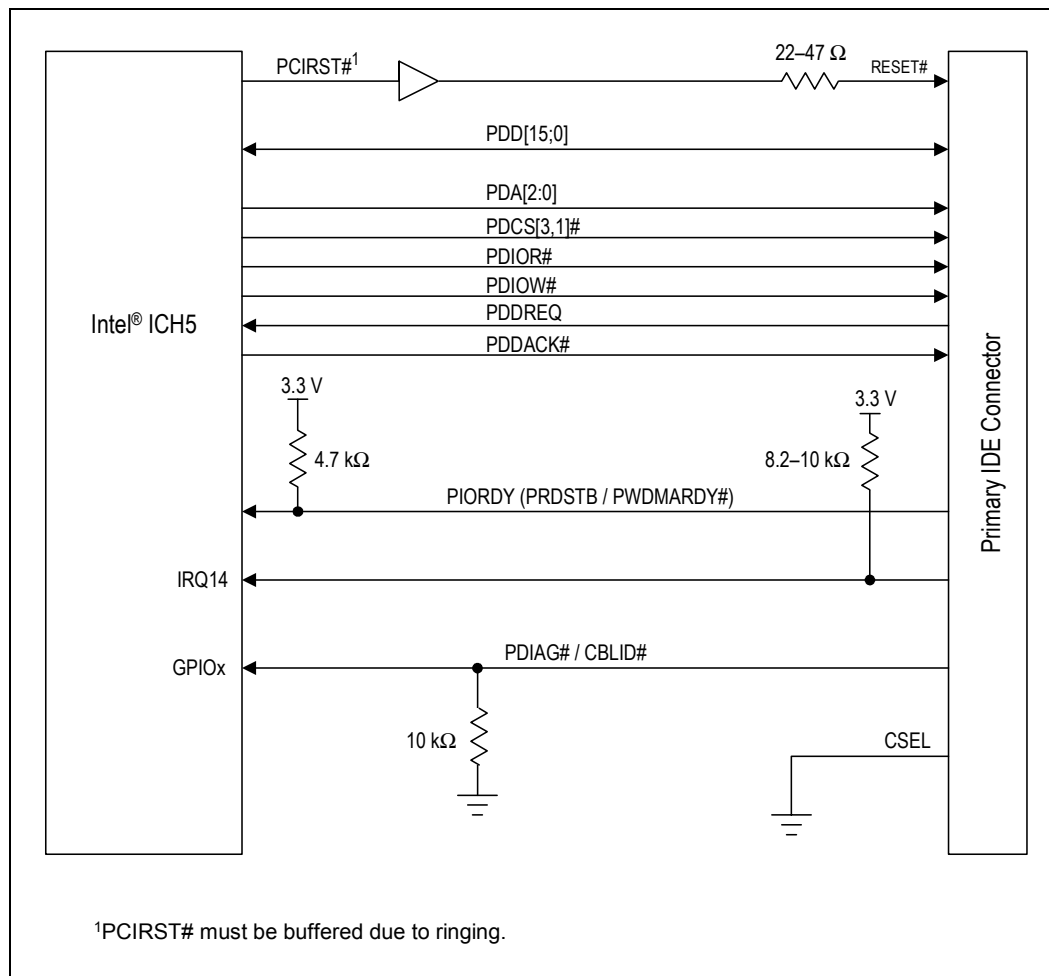
Figure 97. Connection Requirements for Primary IDE Connector
