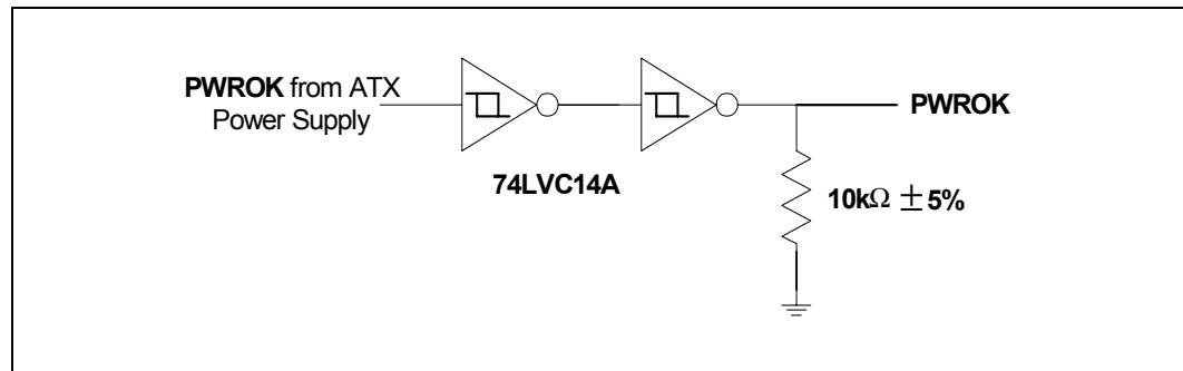
Figure 149. PWROK Generation from PWR_OK Output of ATX Supply
