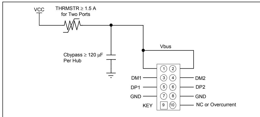
Figure 122. Front Panel Header Schematic
