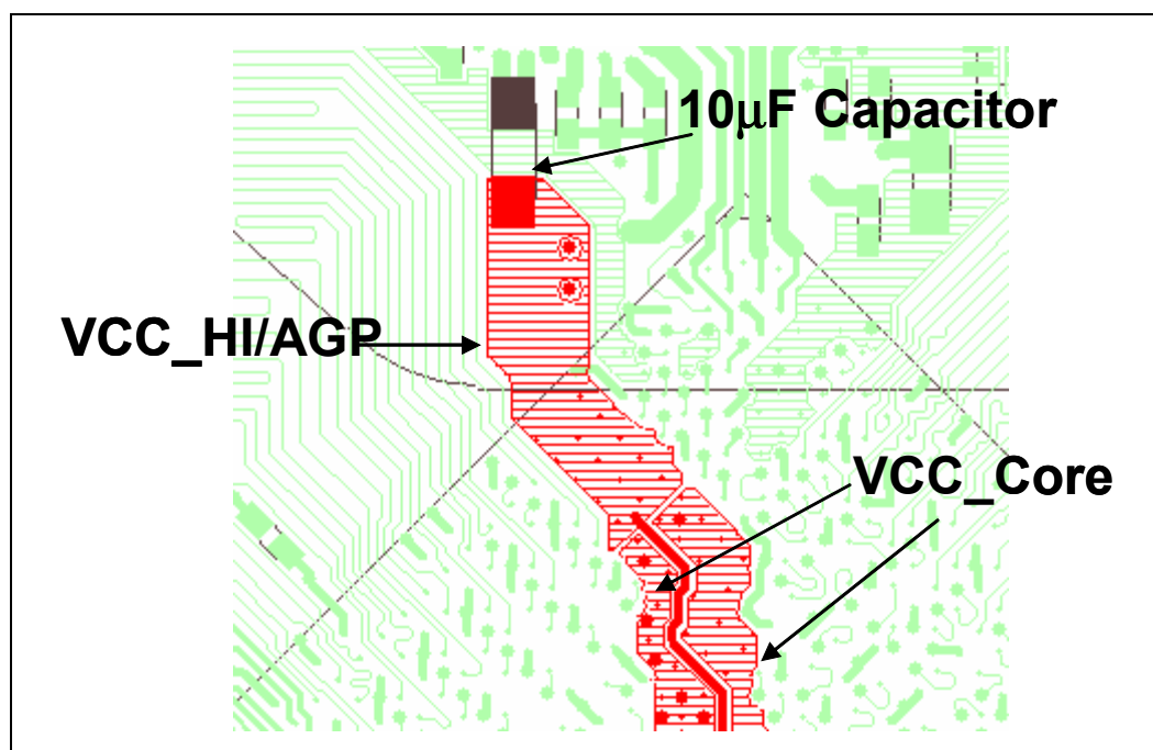
Figure 184. (G)MCH Filter Topology for 1.5 V Core
