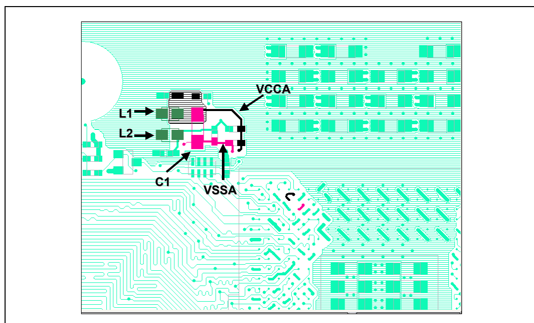
Figure 174. VCCA and VSSA Layer 4 Routing
