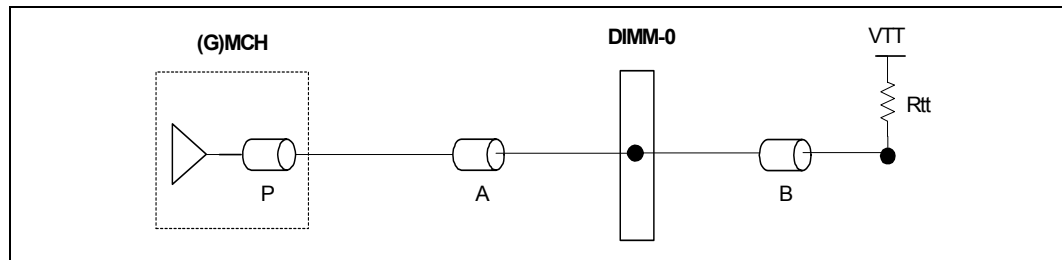
Figure 69. Control Signal Length Matching Requirements
