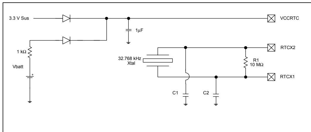
Figure 131. External Circuitry for the Intel® ICH5 RTC
