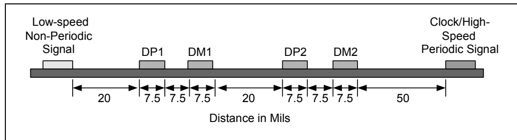
Figure 118. Recommended USB Trace Spacing
