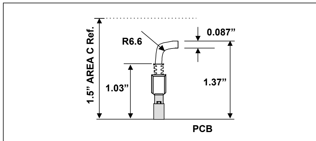
Figure 103. SATA Cable 90-Degree Bend Height Example
