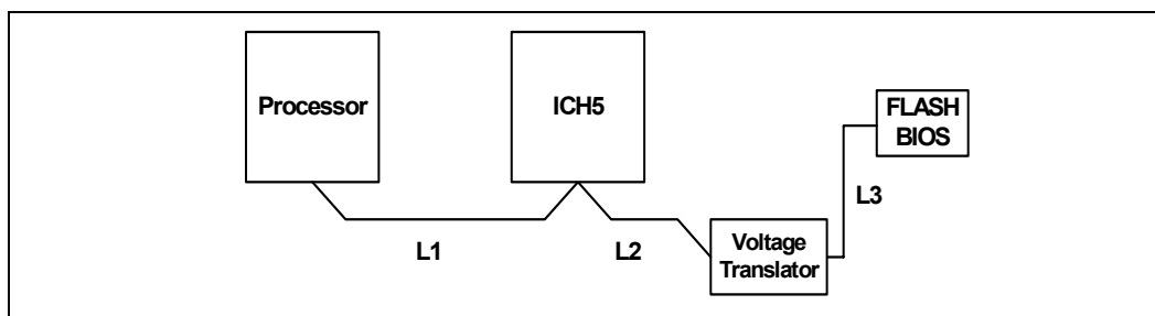
Figure 153. Flash BIOS Signal Topology Solution
