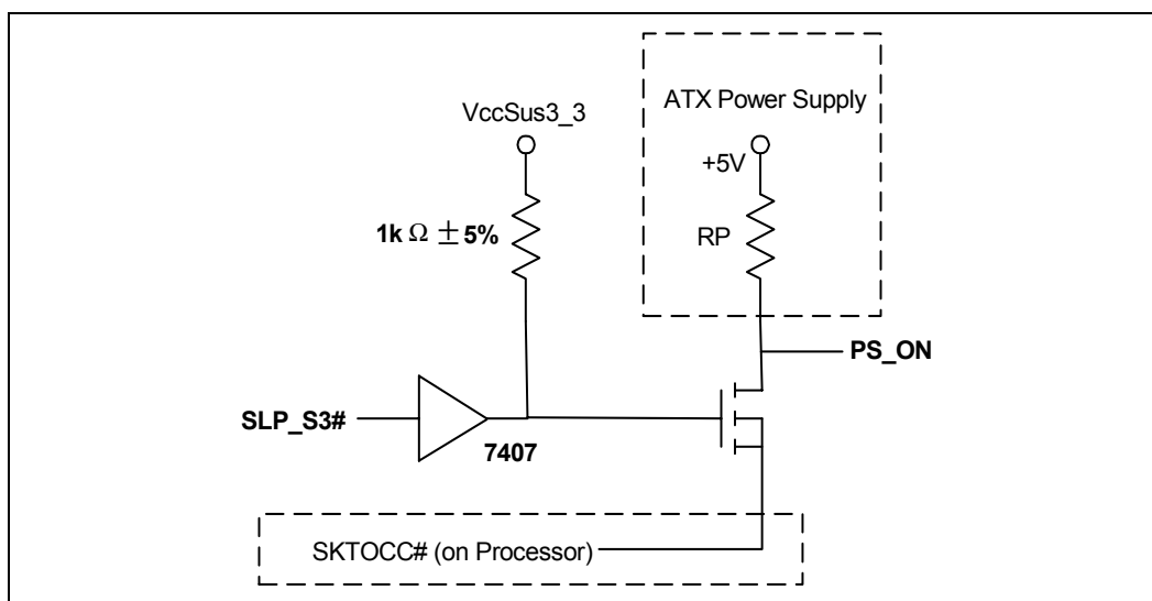
Figure 151. PS_ON Generation from SLP_S3# and SKTOCC#
