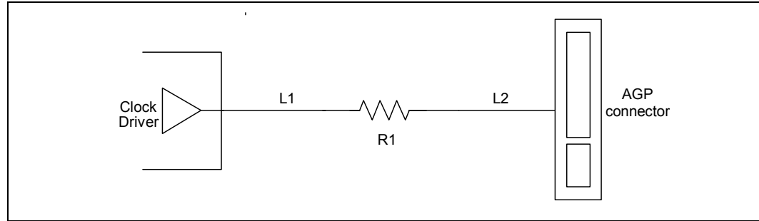
Figure 23. Topology for CLK66 to (G)MCH, Intel® ICH5, and Intel® 82647EI GbE Controller
