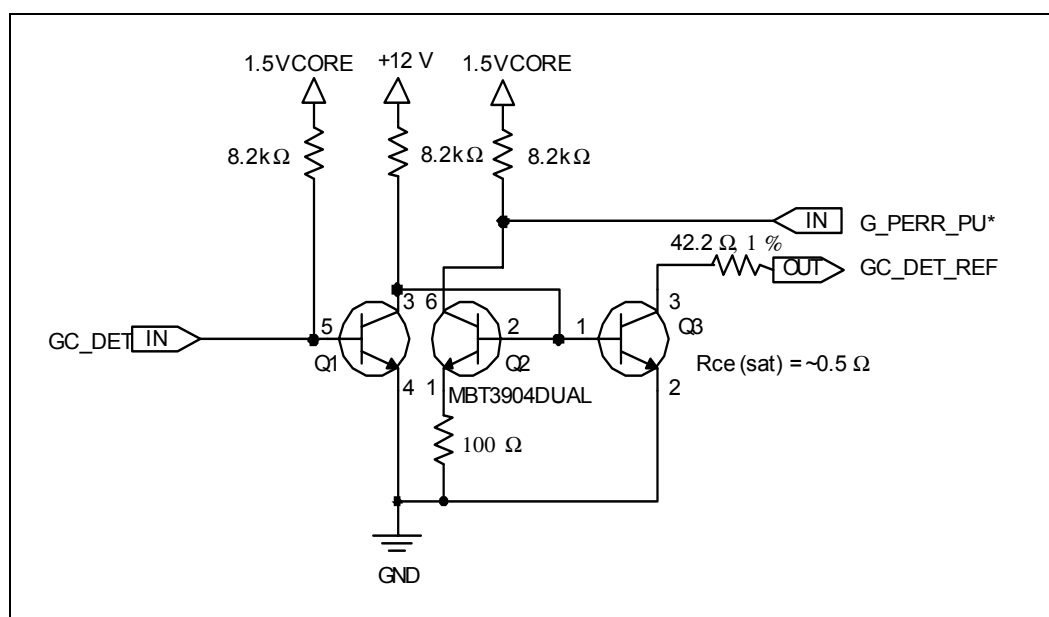
Figure 82. AGP Mode Detection Circuit (Option 2)
