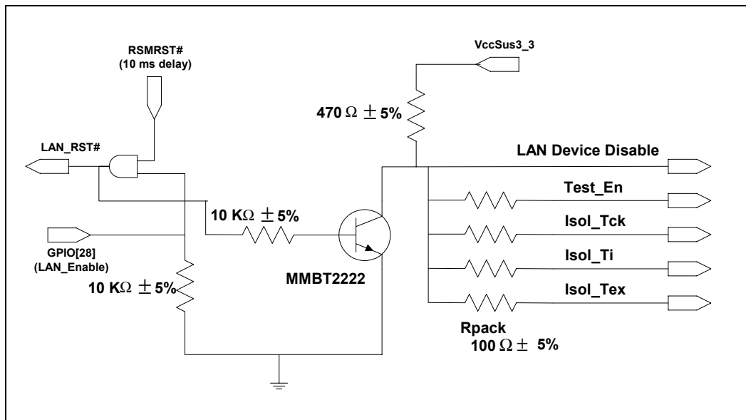
Figure 142. Intel® 82562EZ/ET/EX/EM PLC Components Disable Circuitry
