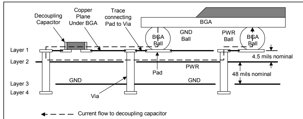
Figure 158. Minimized Loop Inductance Example
