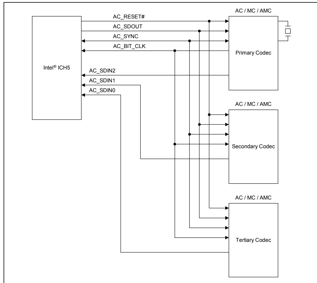
Figure 108. Intel® ICH5 AC '97 (Codec Connection)
